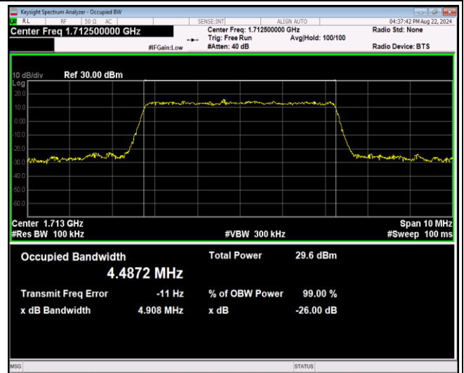
Band4-5MHz-16QAM-20375-25RB#0
