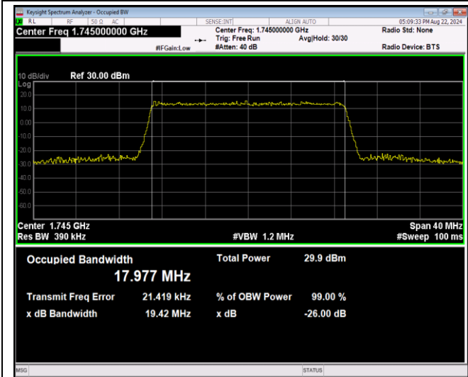
Band4-20MHz-64QAM-20175-100RB#0
