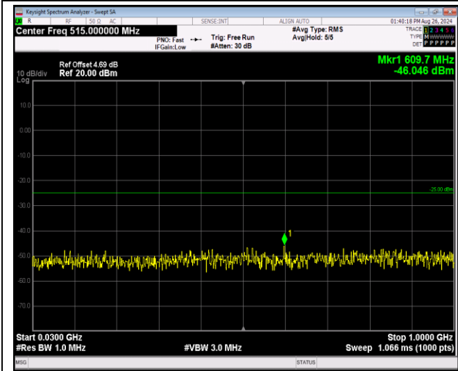
Band7-20MHz-QPSK-21100-1RB#0-Range1:30~1000 MHz
