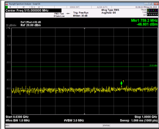
Band7-5MHz-16QAM-21425-1RB#0-Range1:30~1000 MHz
