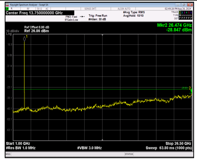
Band41-20MHz-16QAM-40140-1RB#0-Range2:1000~ 26500MHz
