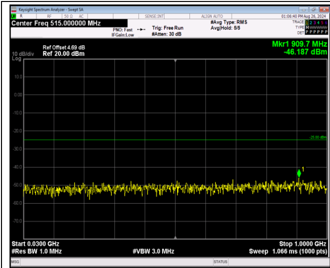
Band7-20MHz-QPSK-20850-1RB#0-Range1:30~1000 MHz
