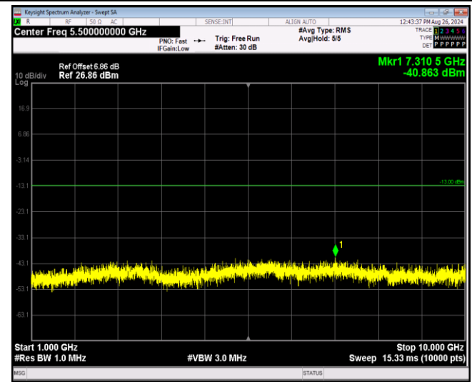
Band5-10MHz-16QAM-20525-1RB#0-Range2:1000~1 0000MHz
