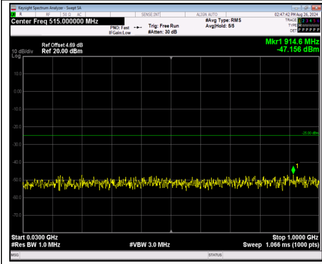
Band41-20MHz-16QAM-40140-1RB#0-Range1:30~10 00MHz
