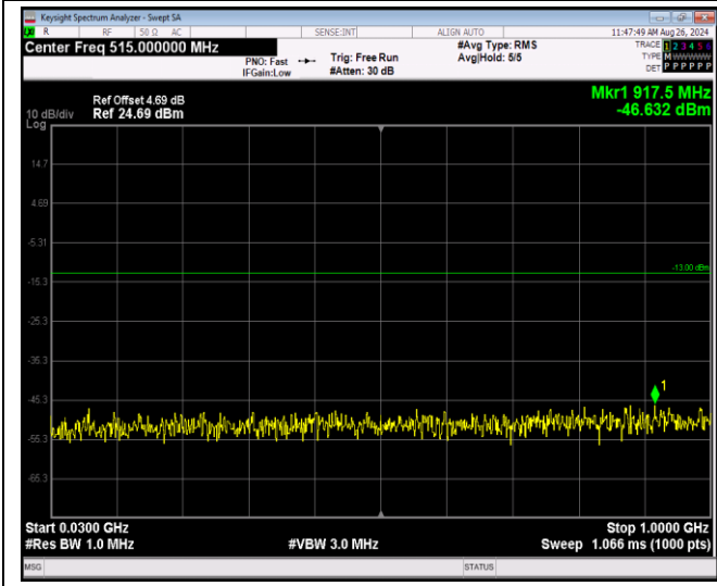
Band4-20MHz-64QAM-20175-1RB#0-Range1:30~100 OMHz
