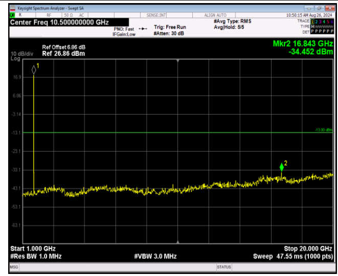
Band4-1.4MHz-64QAM-19957-1RB#0-Range2:1000~20000MHz
