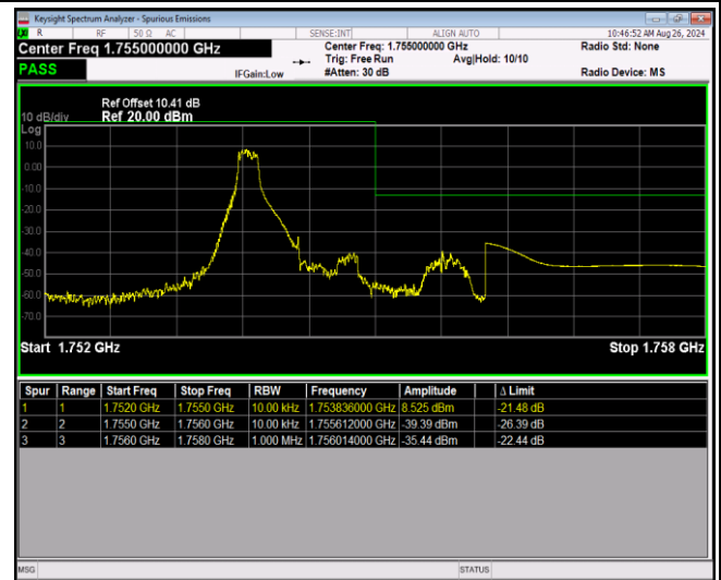
Band4-1.4MHz-64QAM-20393-6RB#0
