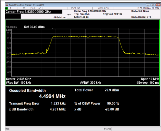
Band7-5MHz-64QAM-20775-25RB#0
