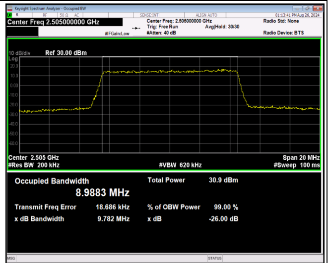
Band7-10MHz-QPSK-21400-50RB#0
