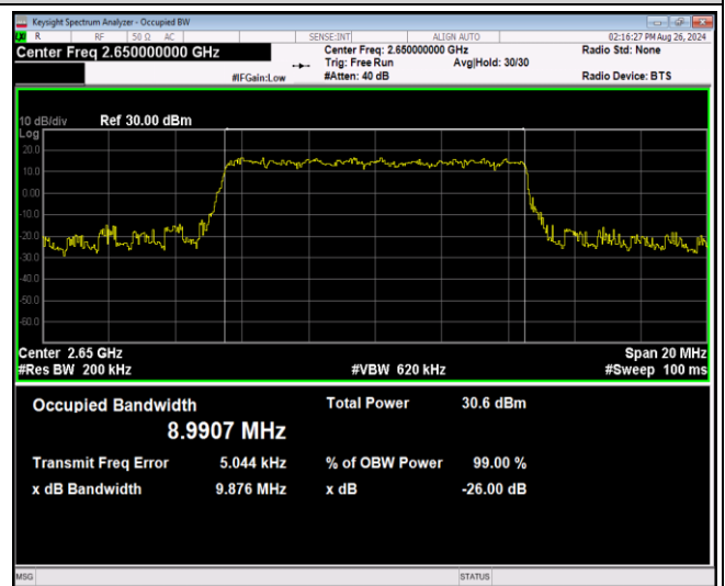
Band41-10MHz-16QAM-40640-50RB#0
