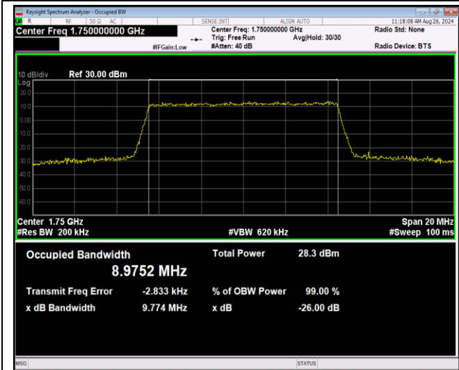
Band4-10MHz-64QAM-20175-50RB#0
