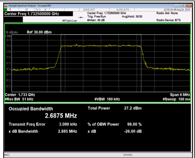
Band4-3MHz-64QAM-19965-15RB#0
