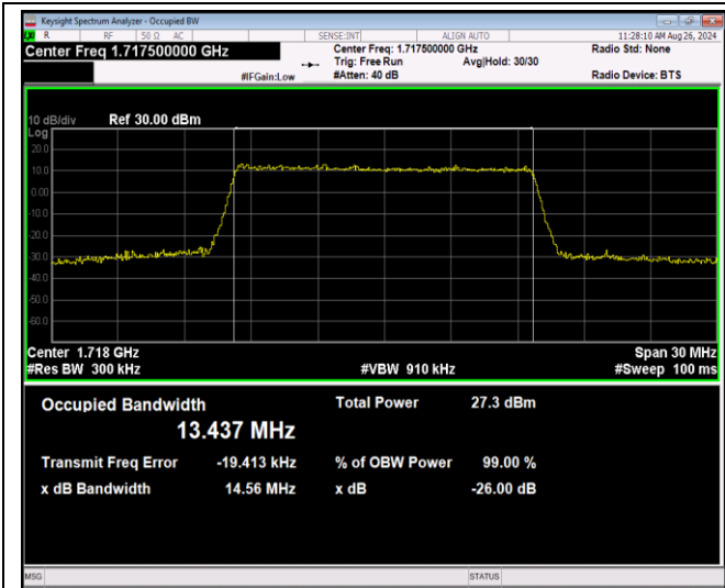
Band4-15MHz-64QAM-20325-75RB#0
