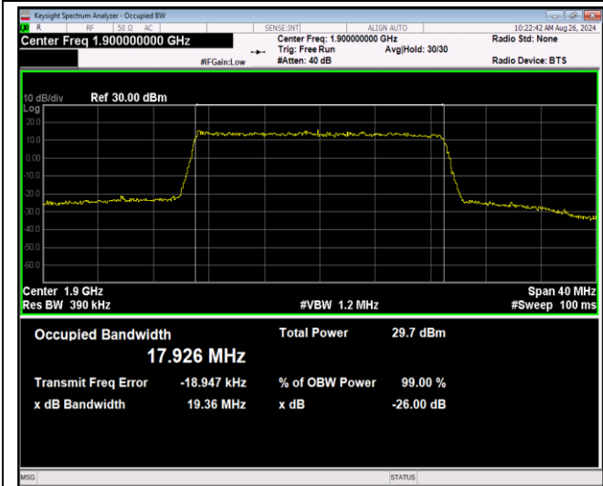
Band2-20MHz-64QAM-18900-100RB#0
