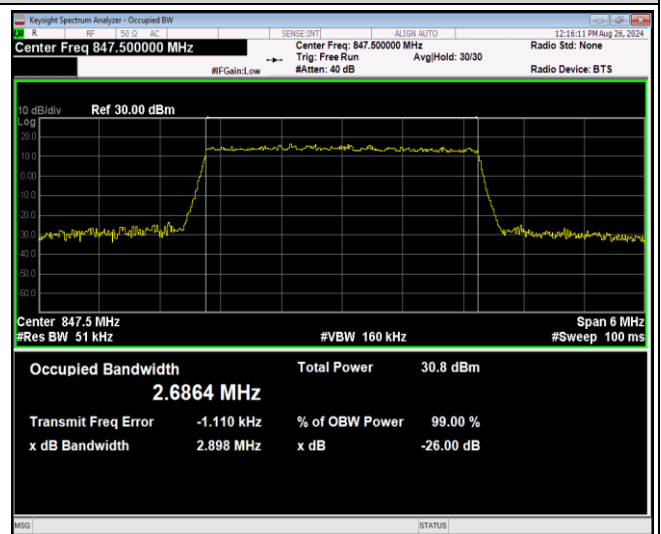
Band5-3MHz-16QAM-20525-15RB#0
