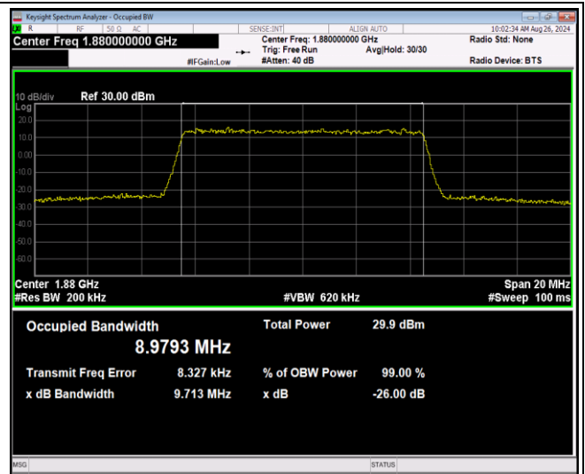
Band2-10MHz-64QAM-18650-50RB#0
