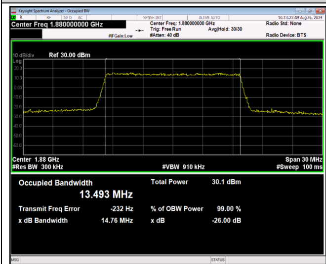
Band2-15MHz-64QAM-18675-75RB#0
