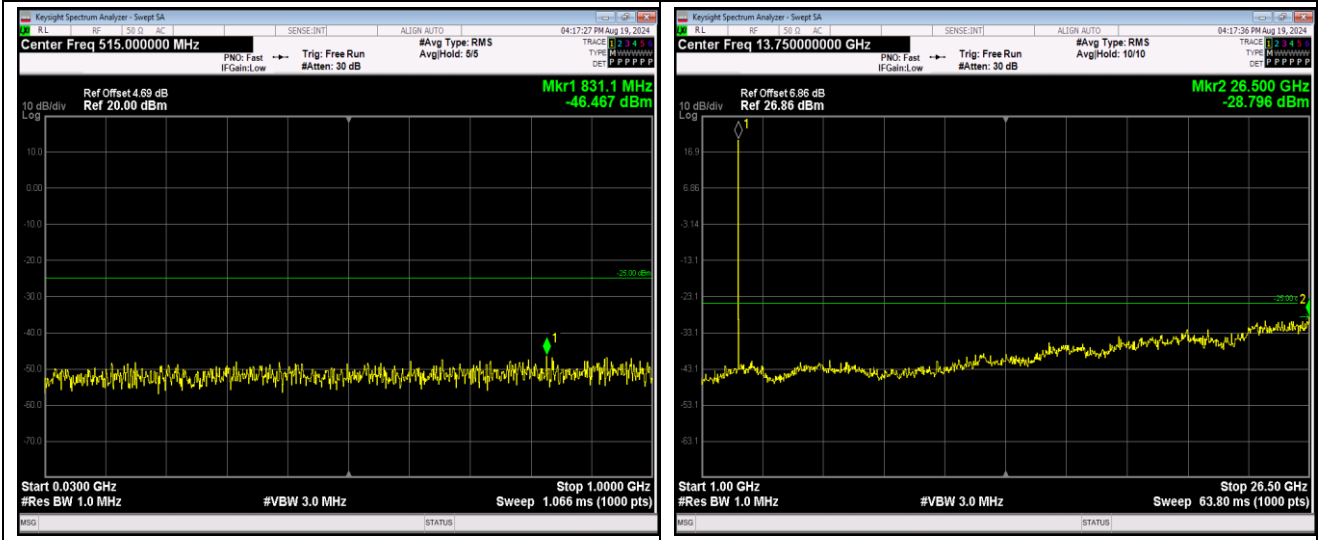
Band41-5MHz-64QAM-40640-1RB#0-Range1:30~1000MHz
