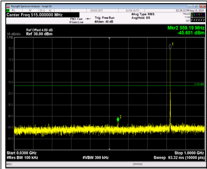
Band5-1.4MHz-64QAM-20525-1RB#0-Range1:30~1000MHz
