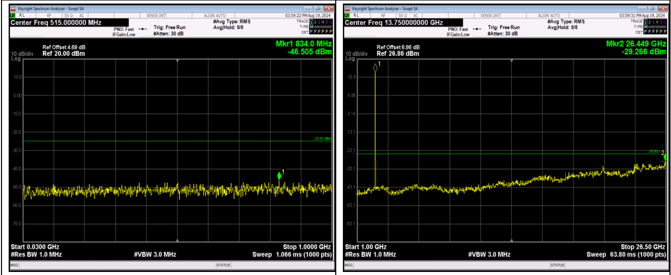
Band7-20MHz-64QAM-20850-1RB#0-Range1:30~1000MHz
