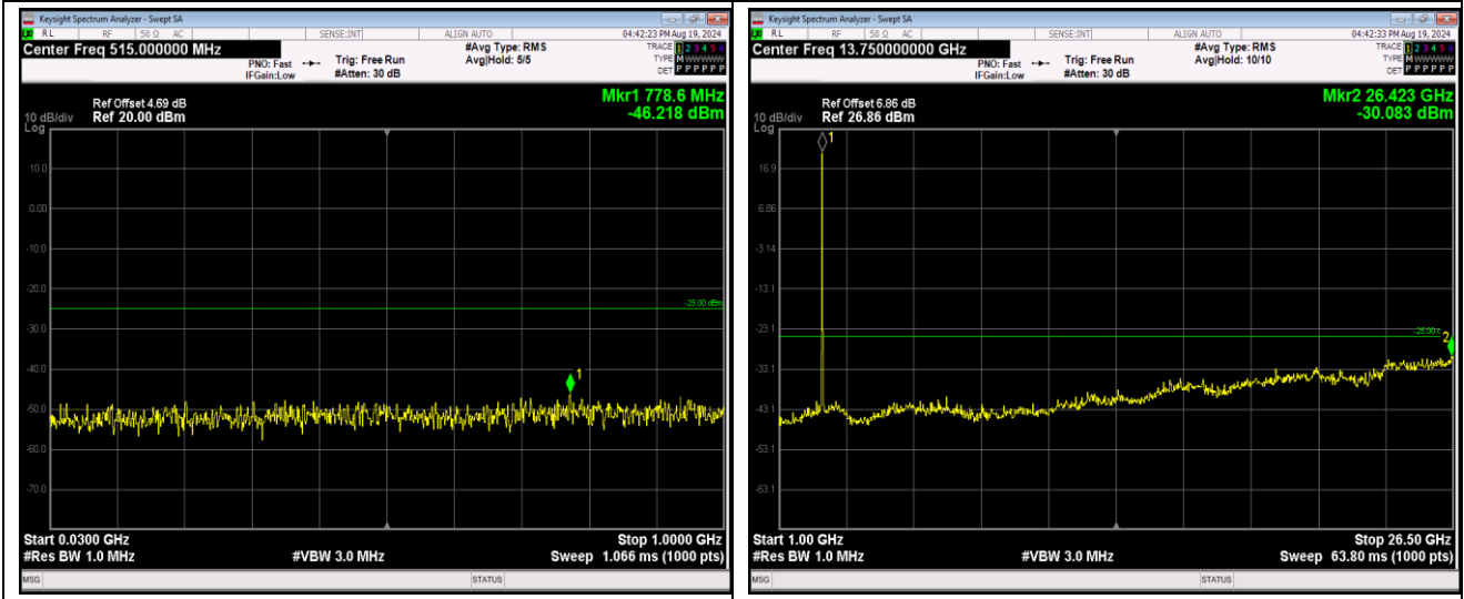
Band41-20MHz-16QAM-40140-1RB#0-Range1:30~1000MHz
