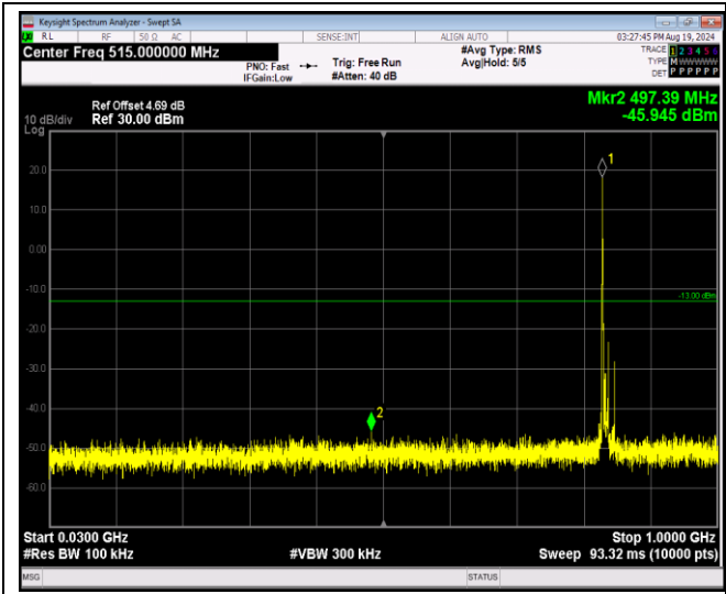
Band5-10MHz-64QAM-20600-1RB#0-Range1:30~1000MHz
