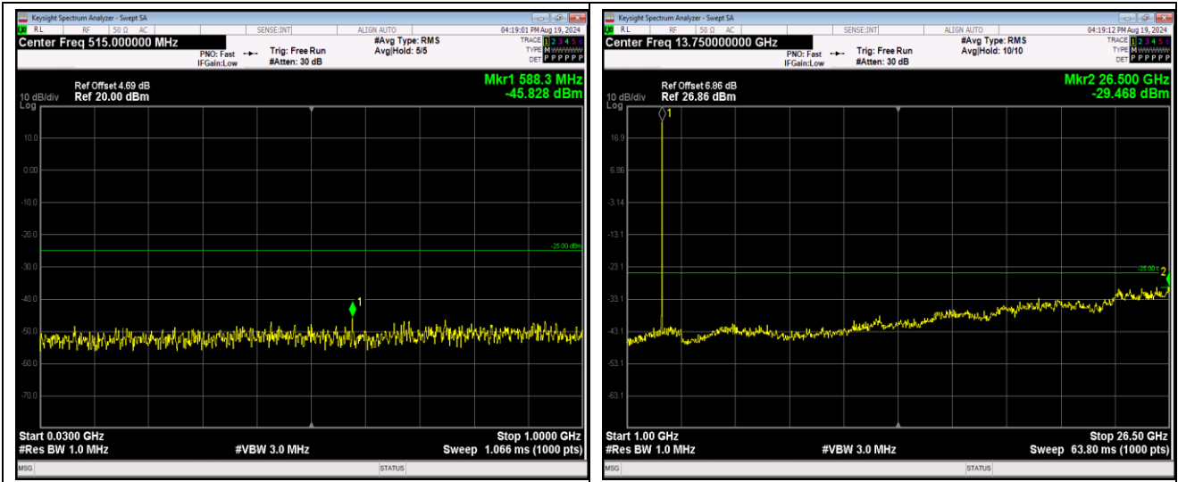
Band41-5MHz-64QAM-40065-1RB#0-Range1:30~1000MHz
