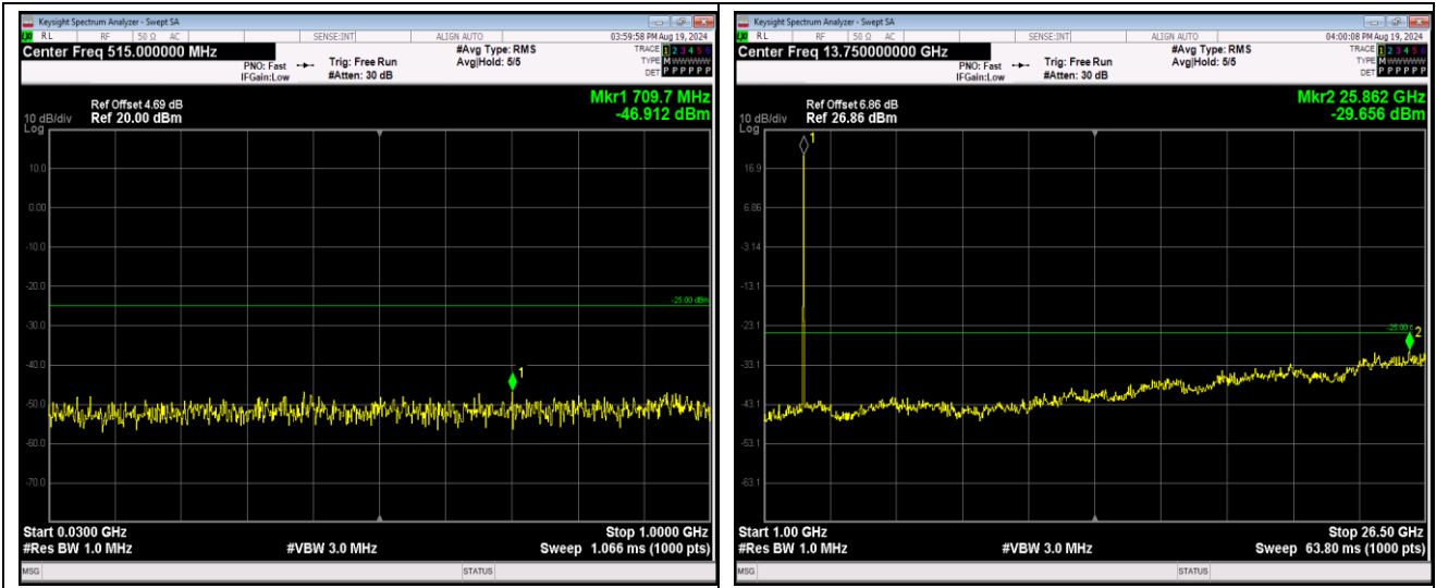
Band7-20MHz-16QAM-21350-1RB#0-Range1:30~1000MHz
