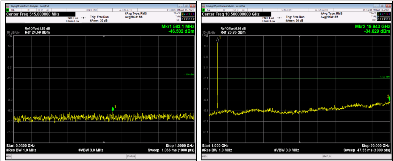
Band4-1.4MHz-QPSK-19957-1RB#0-Range1:30~1000MHz
