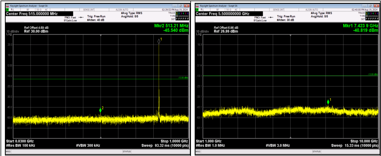
Band5-1.4MHz-QPSK-20643-1RB#0-Range1:30~1000MHz
