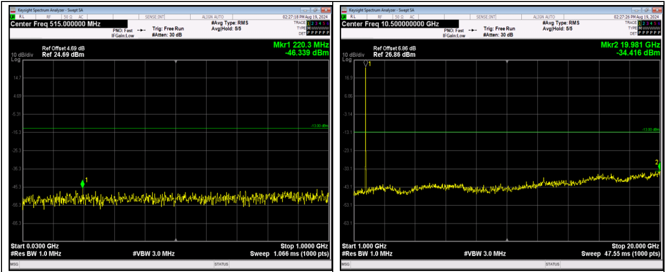
Band4-20MHz-64QAM-20050-1RB#0-Range1:30~1000MHz
