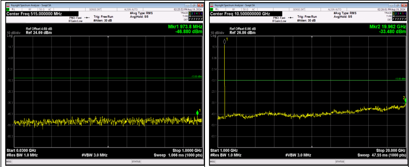
Band4-20MHz-64QAM-20175-1RB#0-Range1:30~1000MHz
