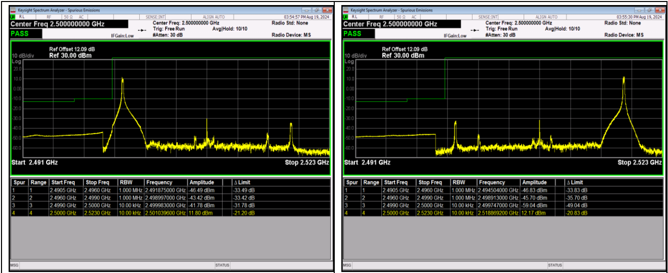
Band7-20MHz-64QAM-20850-100RB#0
