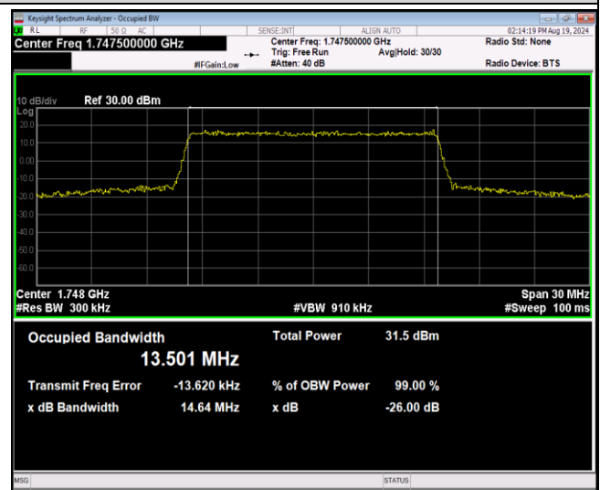
Band4-15MHz-64QAM-20175-75RB#0
