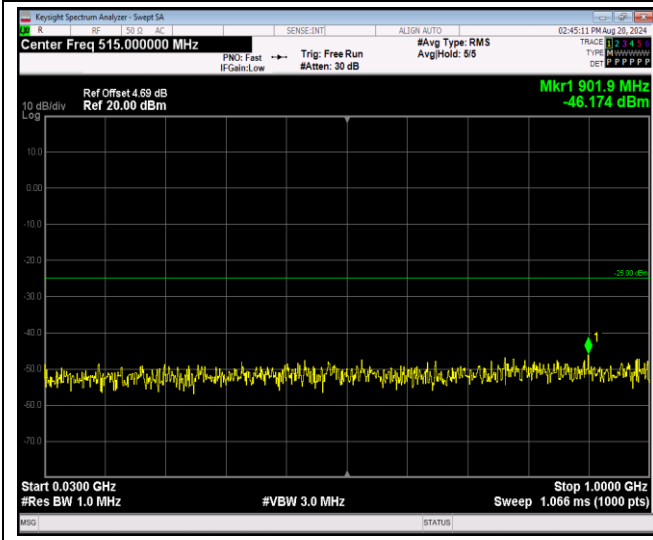
Band41-5MHz-64QAM-40640-1RB#0-Range1:30~1000MHz
