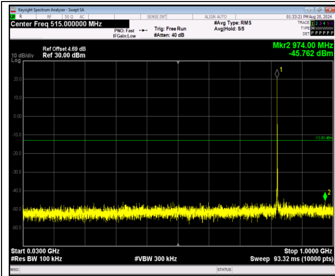
Band5-1.4MHz-64QAM-20525-1RB#0-Range1:30~1000MHz
