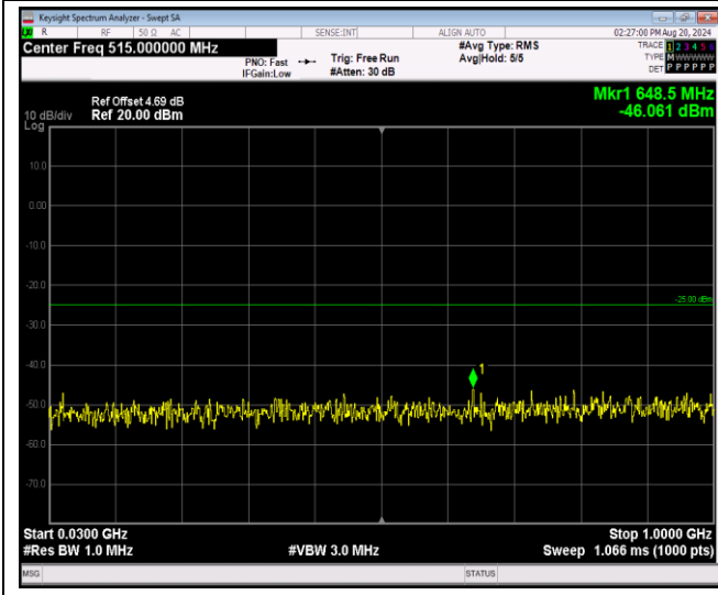
Band7-20MHz-QPSK-21100-1RB#0-Range1:30~100 OMHz
