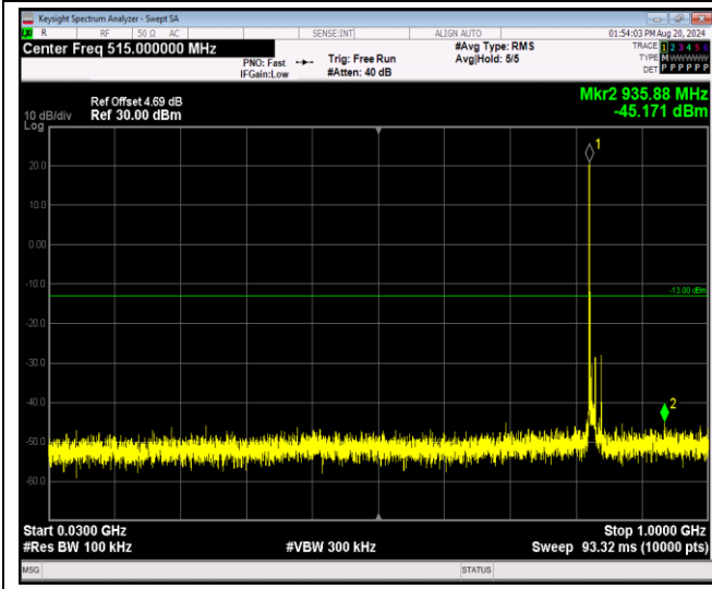
Band5-10MHz-16QAM-20525-1RB#0-Range1:30~1000MHz
