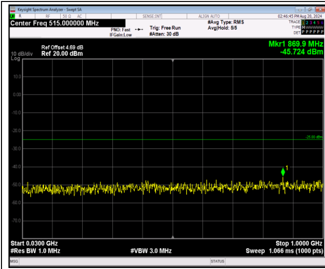
Band41-5MHz-64QAM-40065-1RB#0-Range1:30~1000MHz
