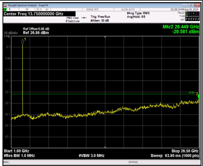
Band7-20MHz-64QAM-20850-1RB#0-Range2:1000~26500MHz
