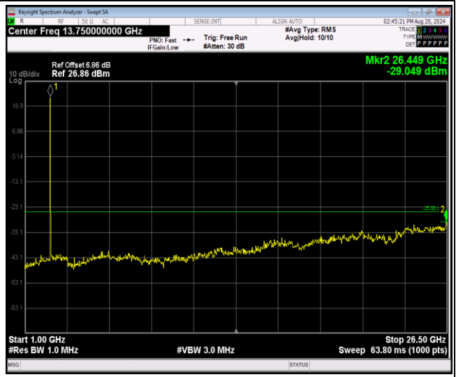
Band41-5MHz-64QAM-40640-1RB#0-Range2:1000~26500MHz
