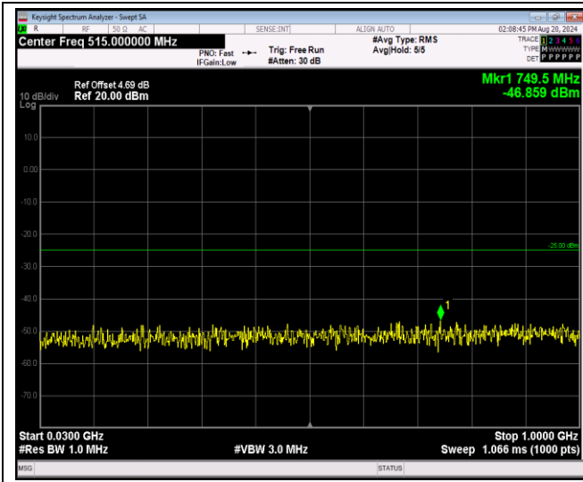
Band7-5MHz-16QAM-21100-1RB#0-Range1:30~100 0MHz
