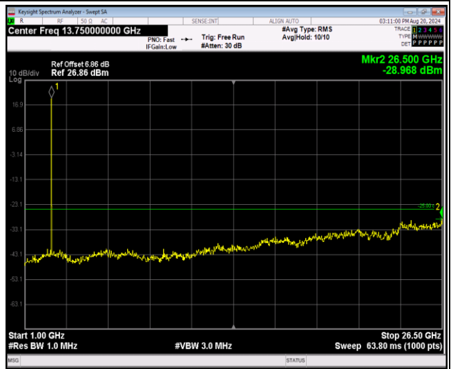
Band41-20MHz-16QAM-40140-1RB#0-Range2:1000~26500MHz
