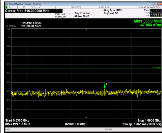
Band7-20MHz-64QAM-20850-1RB#0-Range1:30~1000MHz
