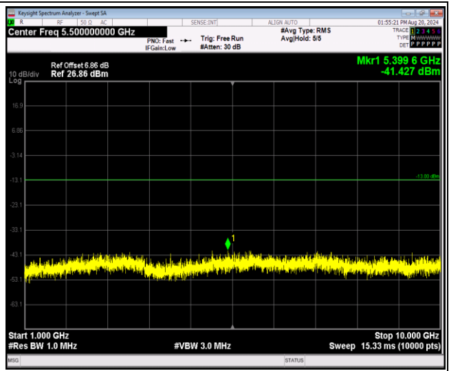
Band5-10MHz-64QAM-20600-1RB#0-Range2:1000~10000MHz
