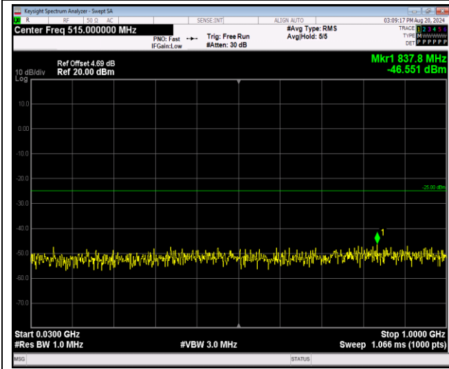
Band41-20MHz-16QAM-40140-1RB#0-Range1:30~1000MHz
