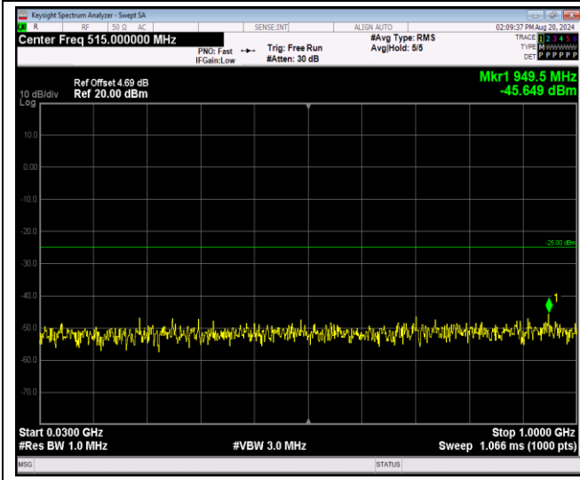
Band7-5MHz-16QAM-21425-1RB#0-Range1:30~100 0MHz
