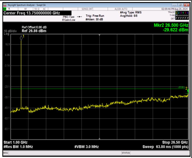
Band7-5MHz-16QAM-21425-1RB#0-Range2:1000~2 6500MHz
