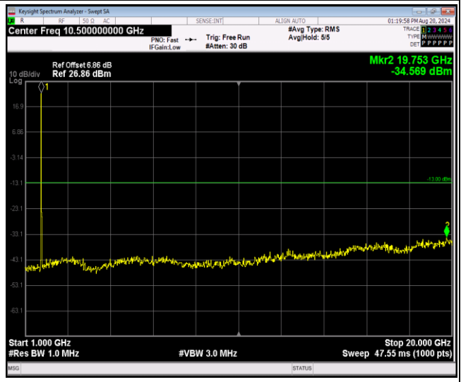
Band4-20MHz-64QAM-20175-1RB#0-Range2:1000~20000MHz
