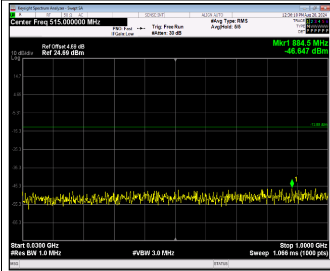
Band2-1.4MHz-64QAM-19193-1RB#0-Range1:30~1000MHz
