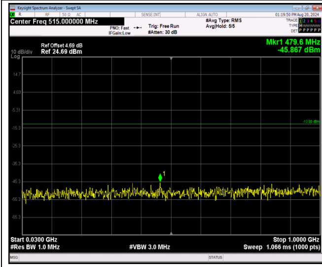
Band4-20MHz-64QAM-20175-1RB#0-Range1:30~1000MHz
