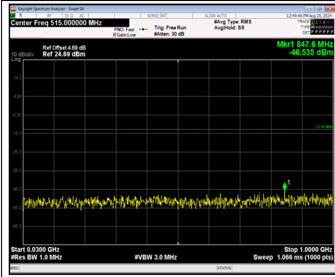
Band4-1.4MHz-QPSK-20175-1RB#0-Range1:30~1000MHz
