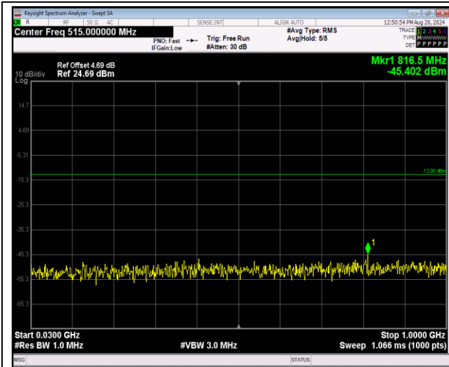
Band4-1.4MHz-16QAM-20393-1RB#0-Range1:30~1000MHz
