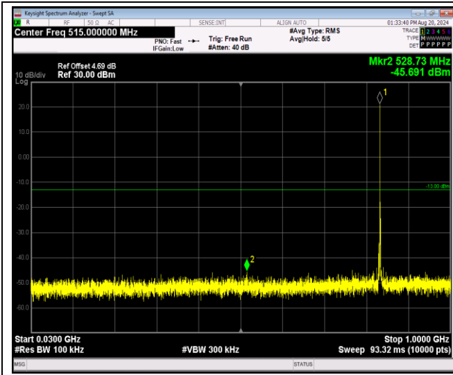
Band5-1.4MHz-QPSK-20643-1RB#0-Range1:30~1000MHz
