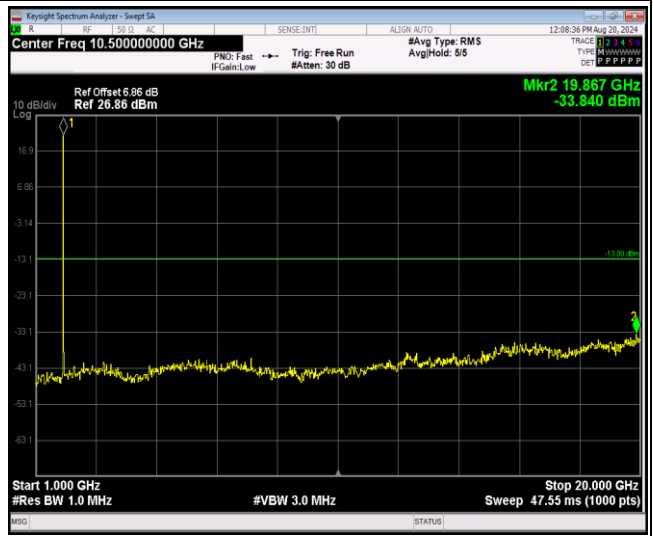
Band2-1.4MHz-16QAM-18607-1RB#0-Range2:1000~20000MHz
