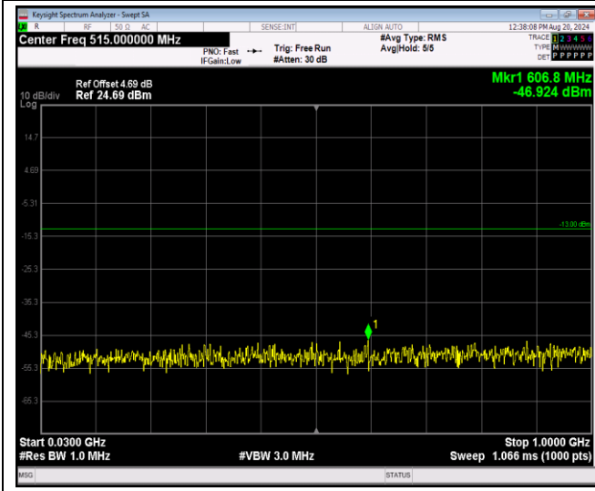
Band2-20MHz-16QAM-19100-1RB#0-Range1:30~1000MHz
