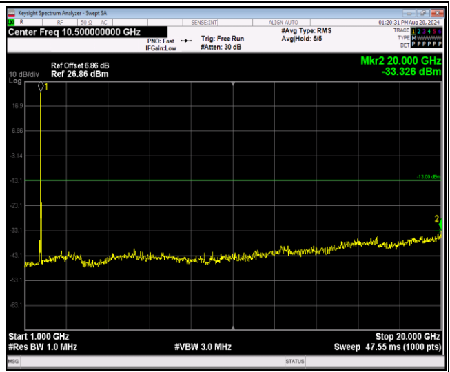
Band4-20MHz-64QAM-20050-1RB#0-Range2:1000~20000MHz
