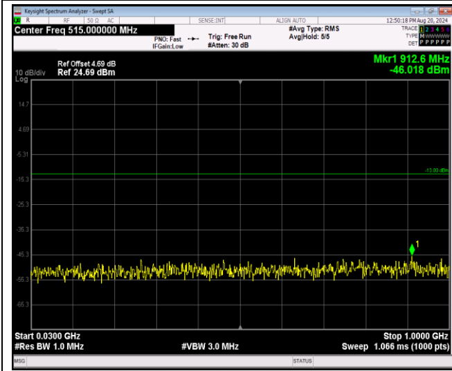
Band4-1.4MHz-64QAM-19957-1RB#0-Range1:30~1000MHz
