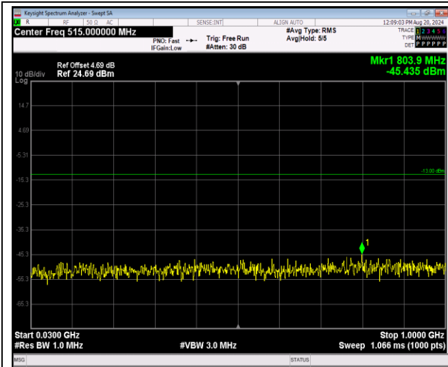
Band2-1.4MHz-16QAM-18607-1RB#0-Range1:30~1000MHz
