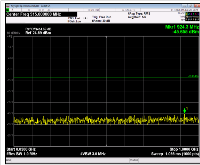
Band4-20MHz-QPSK-20175-1RB#0-Range1:130~100 OMHz
