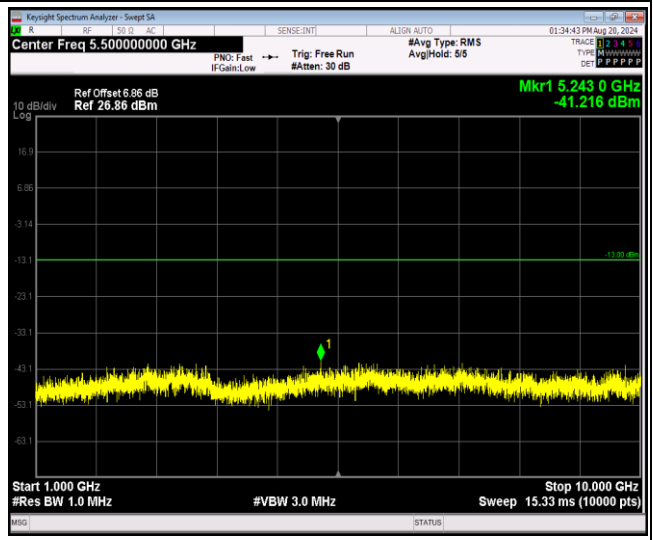
Band5-1.4MHz-16QAM-20407-1RB#0-Range2:1000~10000MHz
