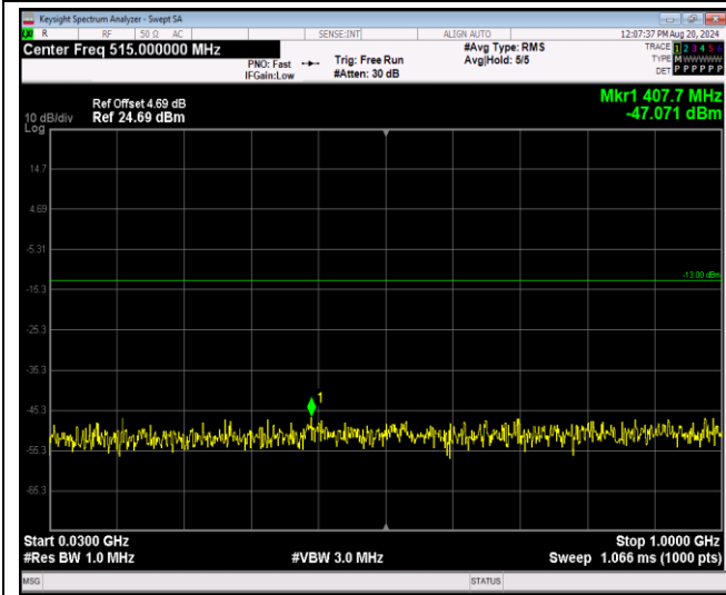
Band2-1.4MHz-16QAM-18900-1RB#0-Range1:30~1000MHz
