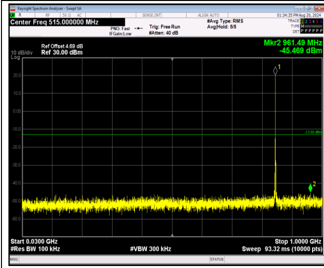
Band5-1.4MHz-16QAM-20407-1RB#0-Range1:30~1000MHz
