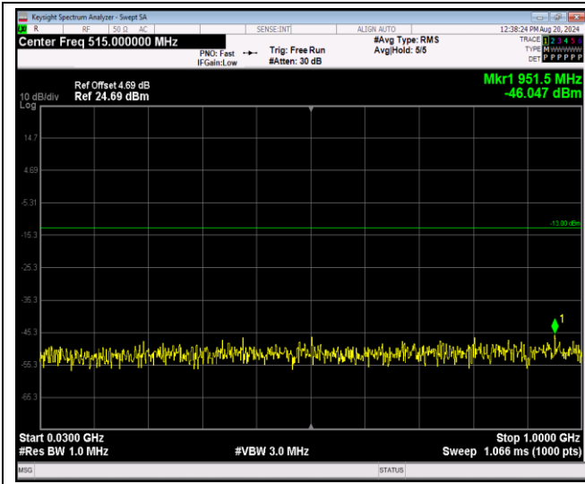
Band4-1.4MHz-QPSK-19957-1RB#0-Range1:30~1000MHz
