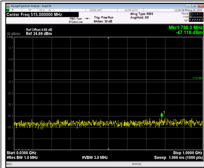
Band2-20MHz-16QAM-18900-1RB#0-Range1:30~1000MHz
