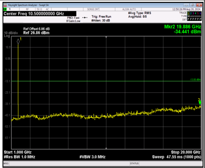
Band4-1.4MHz-64QAM-19957-1RB#0-Range2:1000~20000MHz
