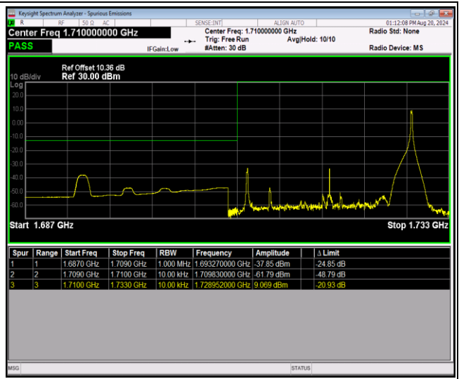
Band4-20MHz-16QAM-20300-1RB#0
