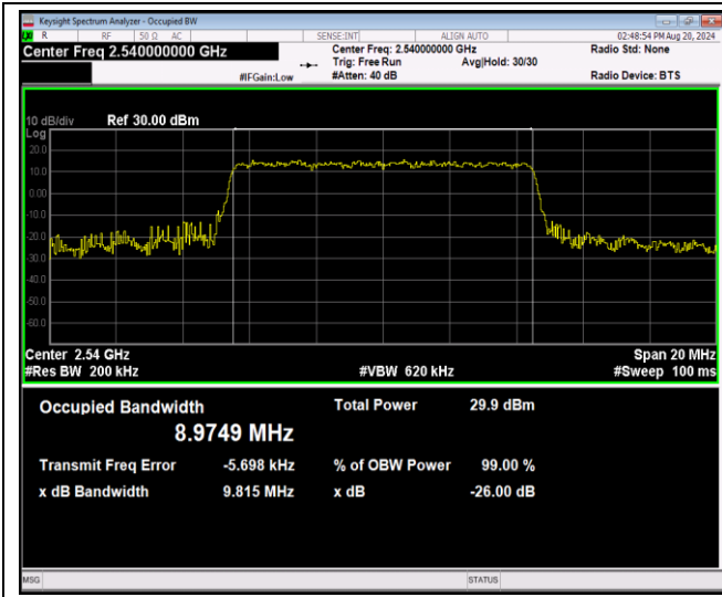
Band41-10MHz-16QAM-41190-50RB#0
