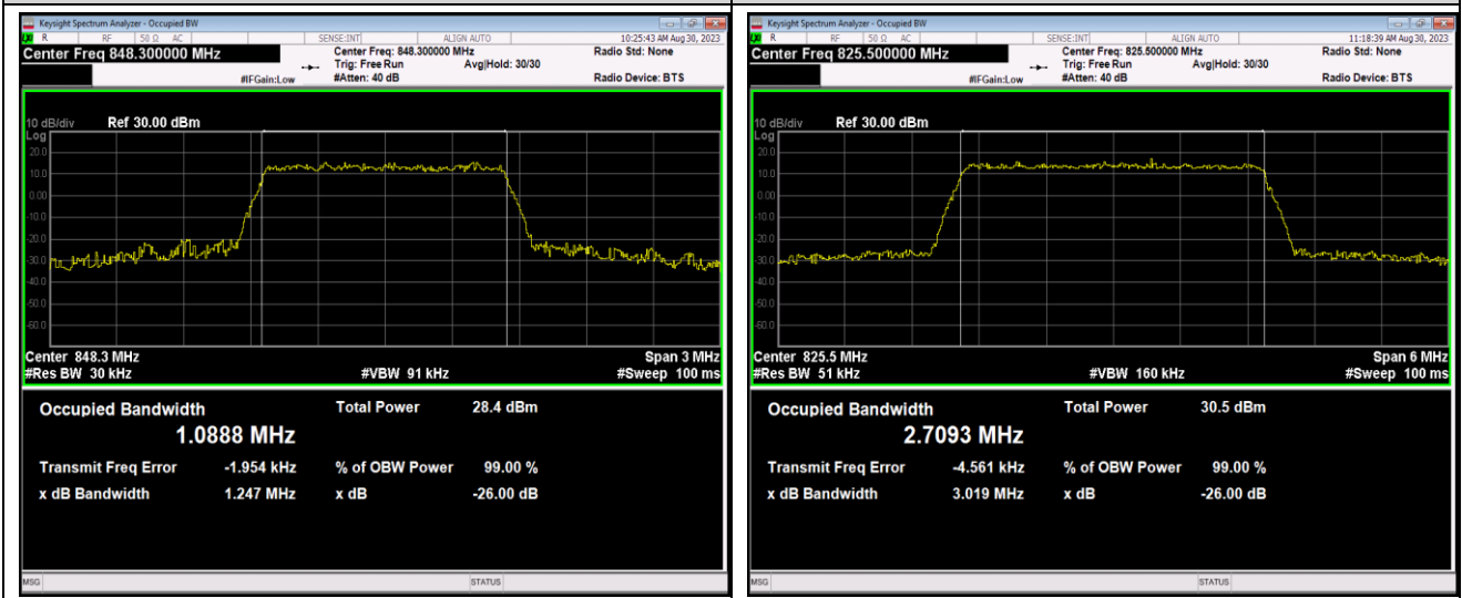
Band5-3MHz-QPSK-20525-15RB#0
