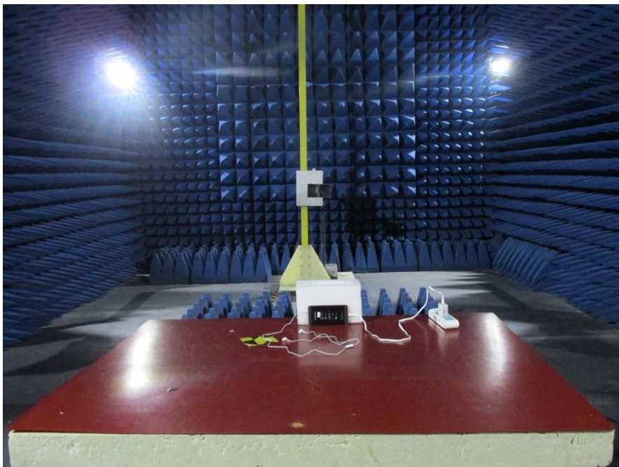
RF TEST
