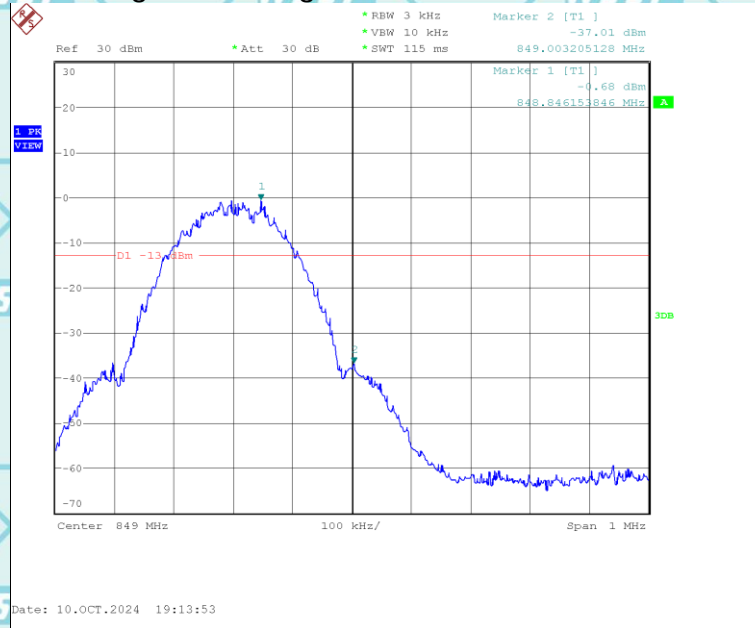
High Band Edge GSM 850 Band CH 251
