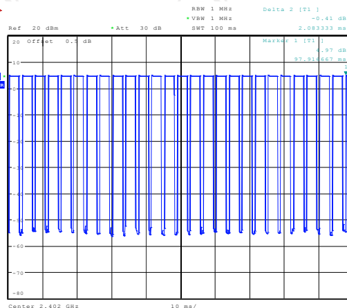
DH5 on time (Count Pulses) Plot on Channel 00
