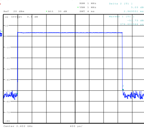
DH5 on time (One Pulse) Plot on Channel 00
