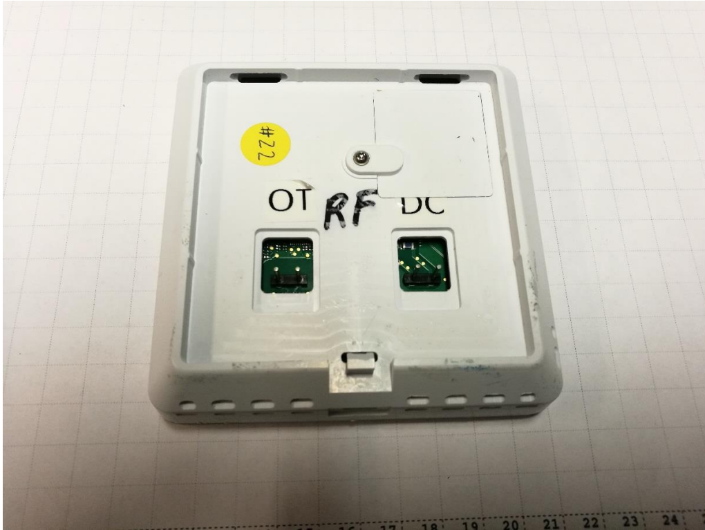
Photograph 3: ViCare Thermostat – Back Side
