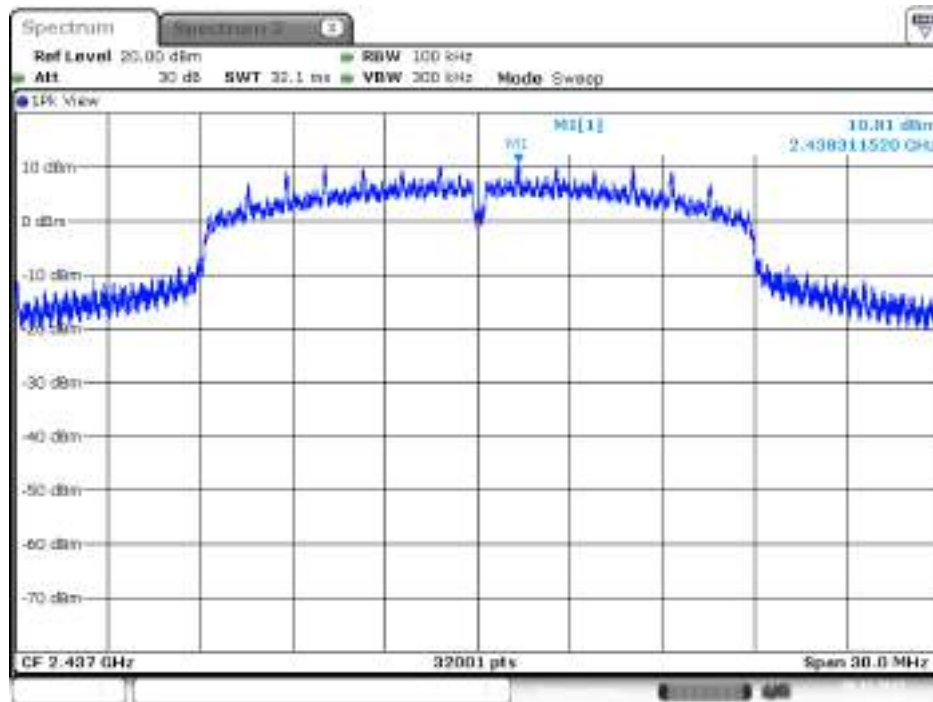
Plot on Configuration IEEE 802.11n MCS0 HT20 / Reference Level / Chain 1
