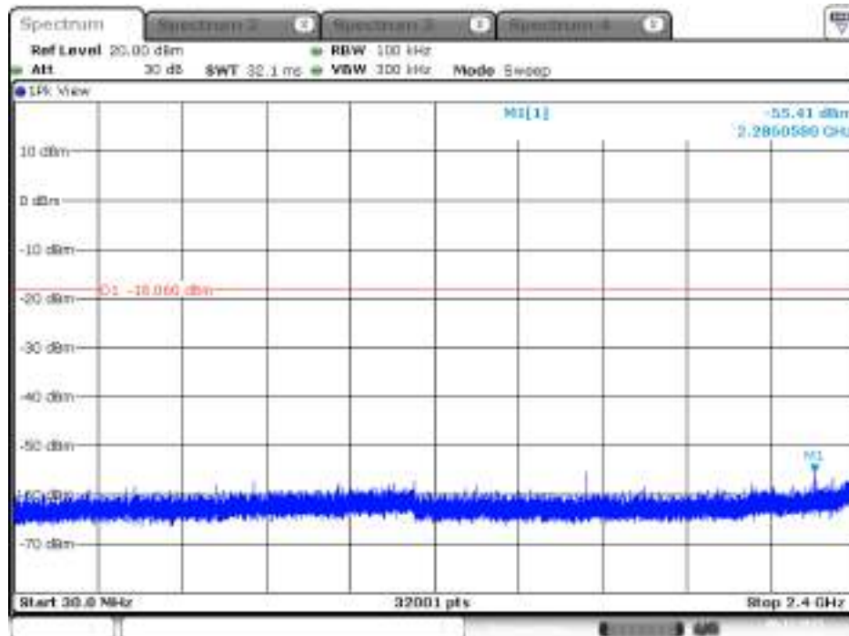
Plot on Configuration IEEE 802.11b / CH 2462 MHz / 30MHz~2400MHz (down 30dBc) / Chain 2
