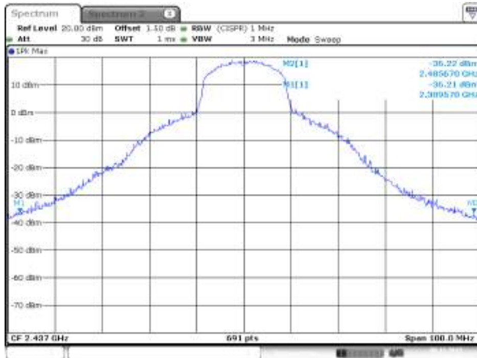
Plot on Configuration IEEE 802.11n MCS0 HT20 / 2437 MHz / Peak / Chain 1
