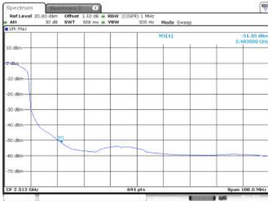
Plot on Configuration IEEE 802.11n MCS0 HT20 / 2462 MHz / Average / Chain 2
