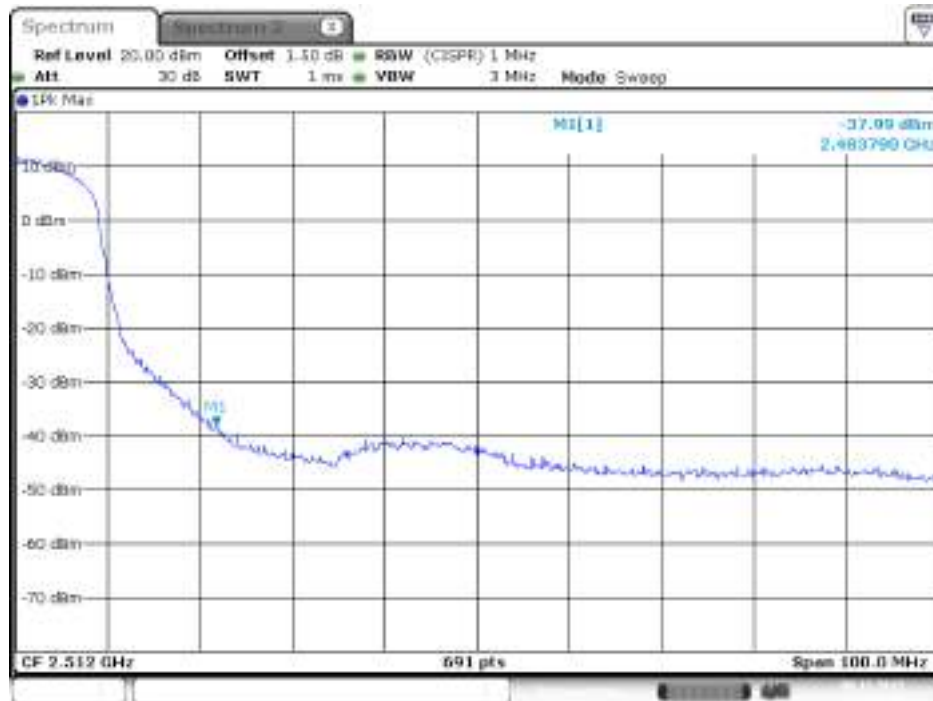
Plot on Configuration IEEE 802.11n MCS0 HT20 / 2462 MHz / Peak / Chain 2
