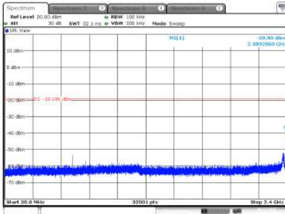
Plot on Configuration IEEE 802.11n MCS0 HT20 / 2412 MHz / 30MHz~2400MHz (down 30dBc) / Chain 1
