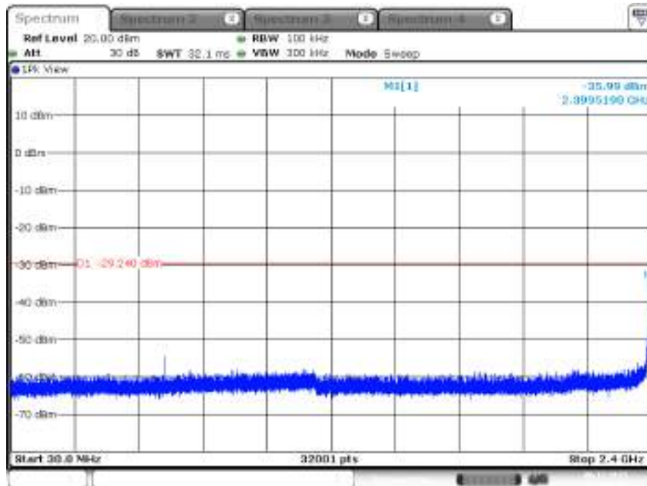
Plot on Configuration IEEE 802.11n MCS0 HT40 / 2422 MHz / 30MHz~2400MHz (down 30dBc) / Chain 1
