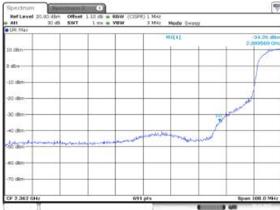
Plot on Configuration IEEE 802.11n MCS0 HT20 / 2412 MHz / Peak / Chain 2
