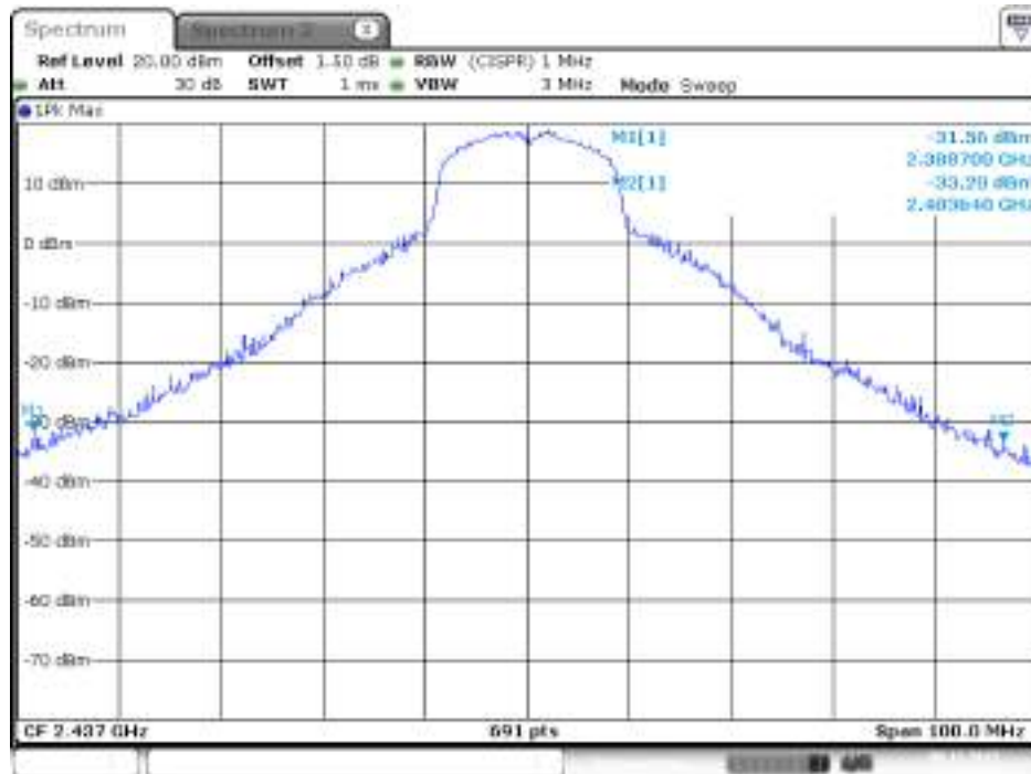
Plot on Configuration IEEE 802.11n MCS0 HT20 / 2437 MHz / Peak / Chain 2
