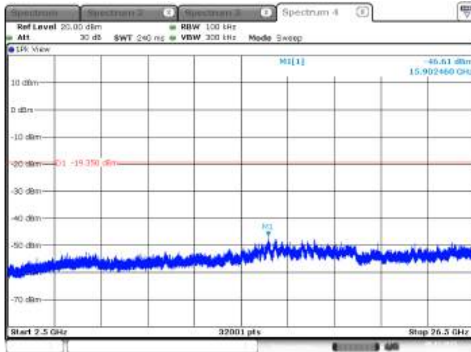
Plot on Configuration IEEE 802.11g / 2412 MHz / 2500MHz~26500MHz (down 30dBc) / Chain 1
