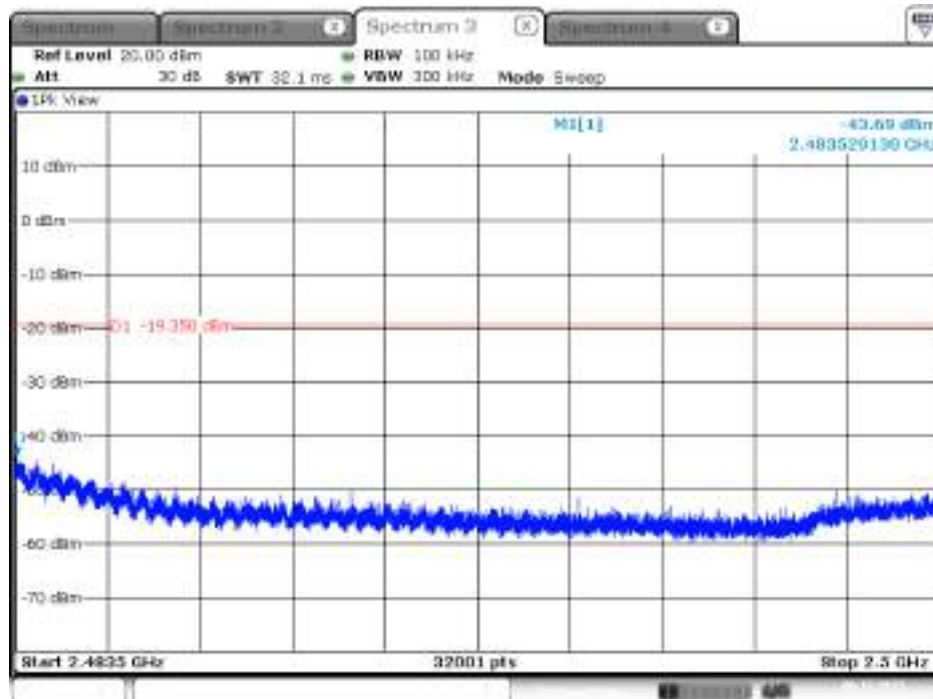
Plot on Configuration IEEE 802.11g / 2462 MHz / 2483.5MHz~2500MHz (down 30dBc) / Chain 1
