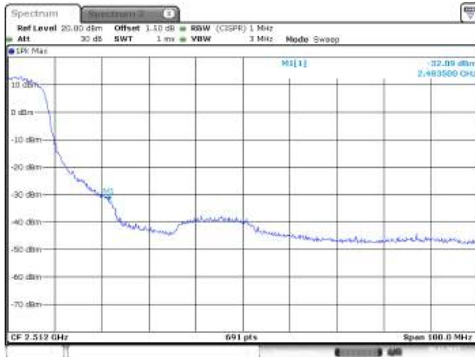
Plot on Configuration IEEE 802.11g / 2462 MHz / Peak / Chain 1
