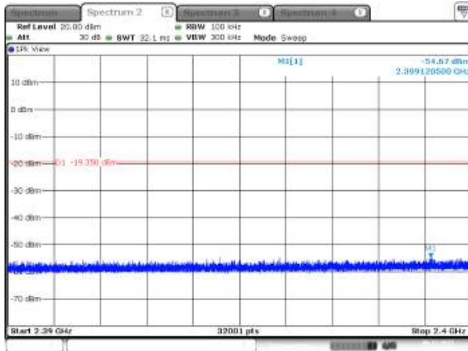
Plot on Configuration IEEE 802.11g / 2462 MHz / 2390MHz~2400MHz (down 30dBc) / Chain 1
