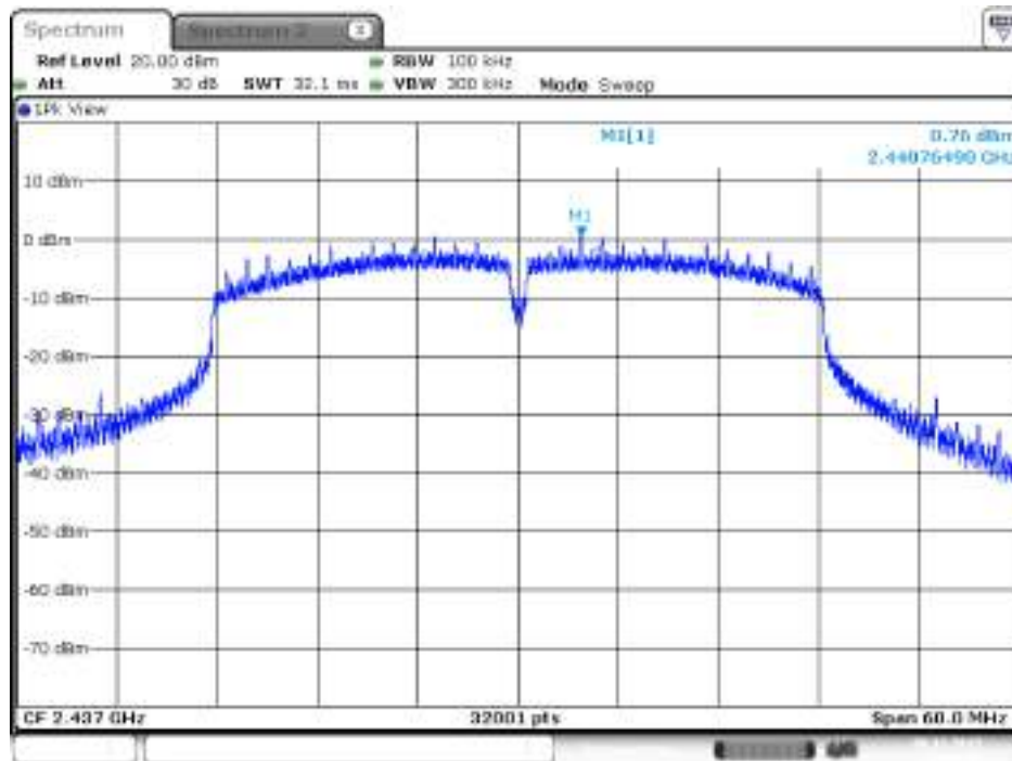
Plot on Configuration IEEE 802.11n MCS0 HT40 / Reference Level / Chain 1
