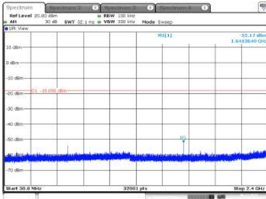
Plot on Configuration IEEE 802.11b / CH 2462 MHz / 30MHz~2400MHz (down 30dBc) / Chain 1
