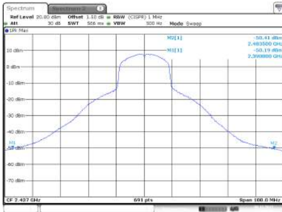
Plot on Configuration IEEE 802.11n MCS0 HT20 / 2437 MHz / Average / Chain 1
