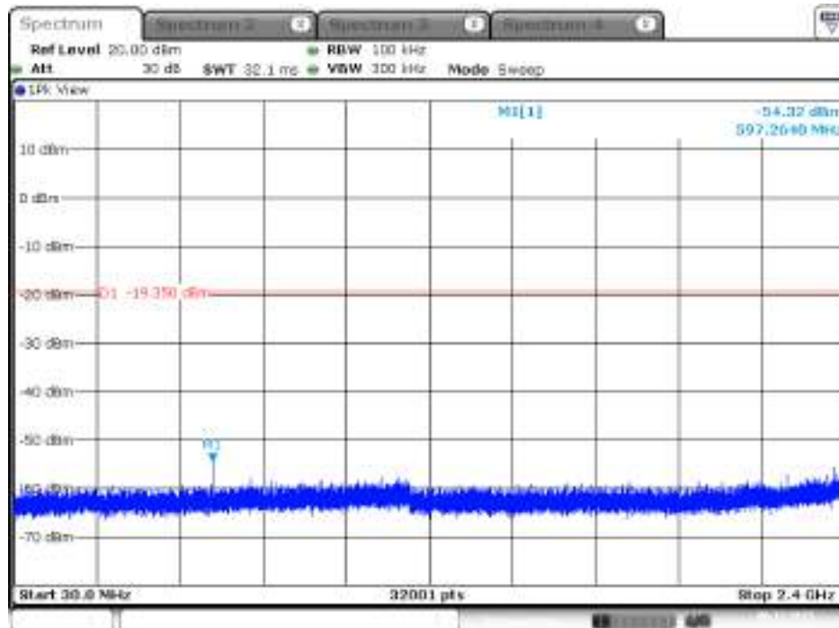
Plot on Configuration IEEE 802.11g / 2462 MHz / 30MHz~2400MHz (down 30dBc) / Chain 1
