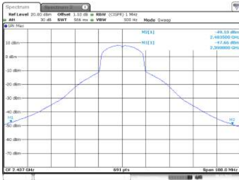
Plot on Configuration IEEE 802.11n MCS0 HT20 / 2437 MHz / Average / Chain 2
