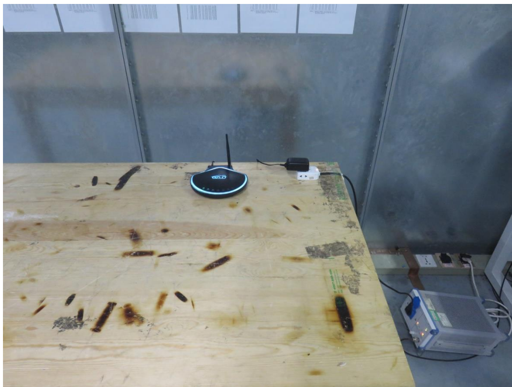
conducted emission
