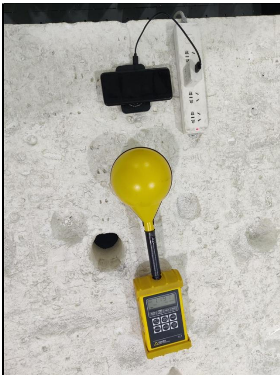
Test Position C - Exposure photo from side edge surface-Front(15cm) (TM1)
