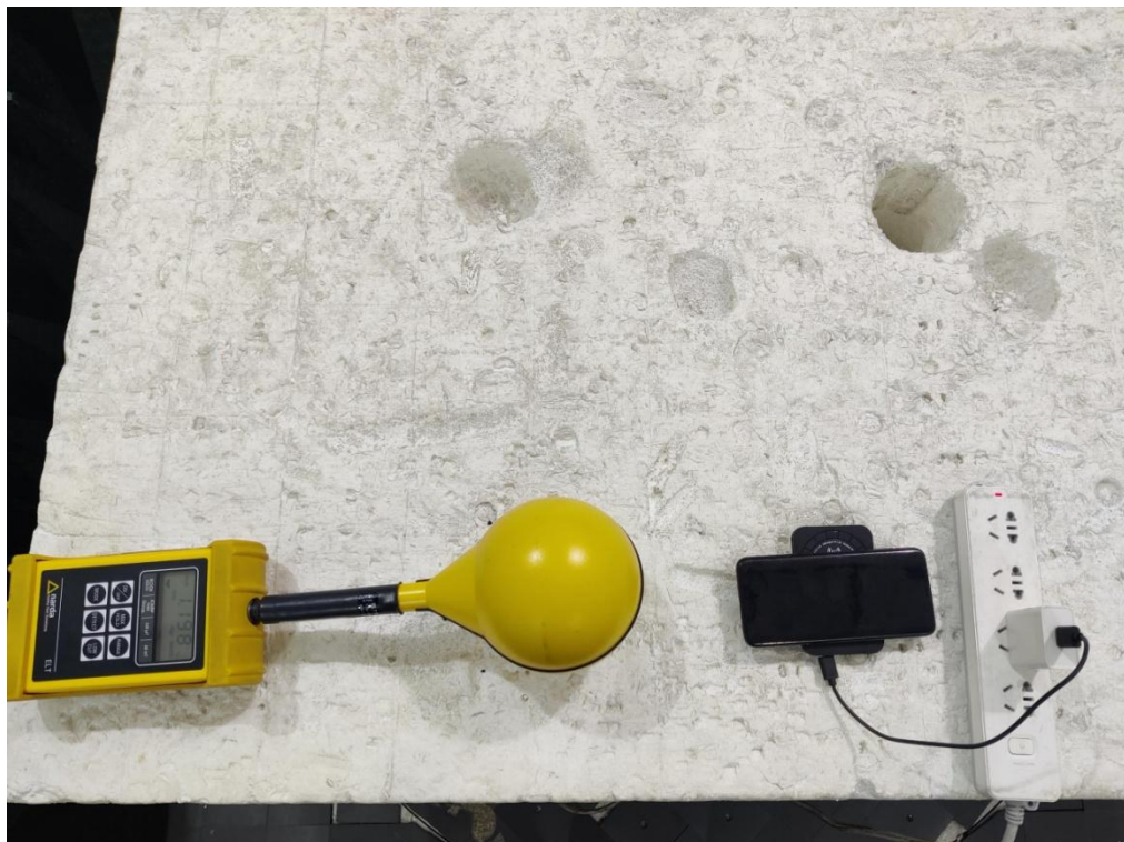
Test Position B - Exposure photo from side edge surface-Left(15cm) (TM1)
