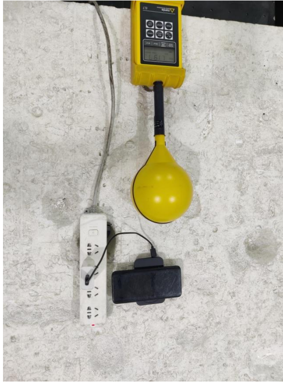
Test Position A - Exposure photo from side edge surface-Rear(15cm) (TM1)
