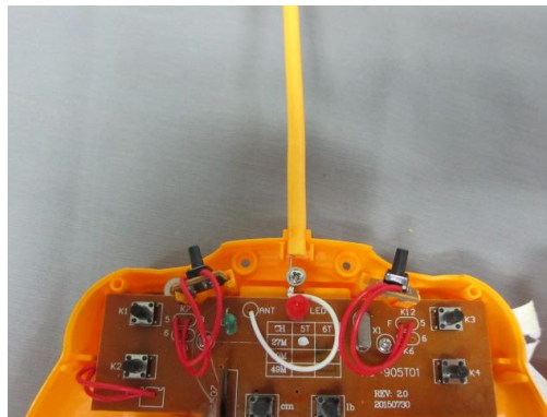
Internal irreplaceable antenna
