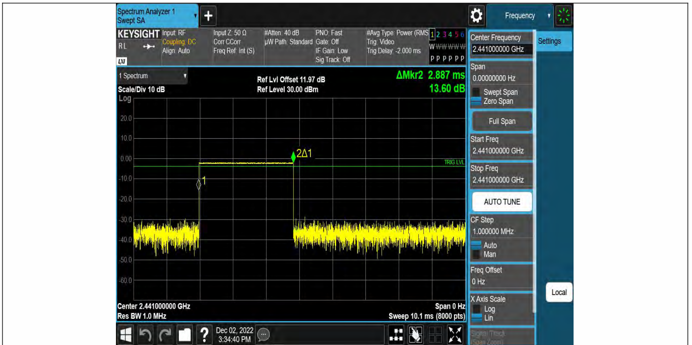
DH5-Ant1-Hop-2.887-106.67
