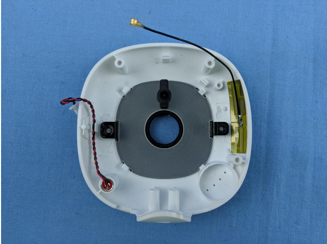
Front Housing
