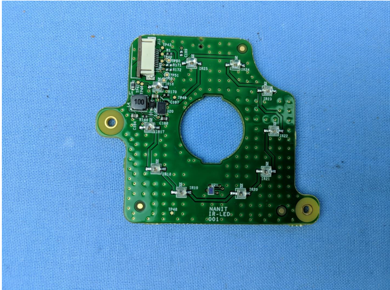
LED Board Front
