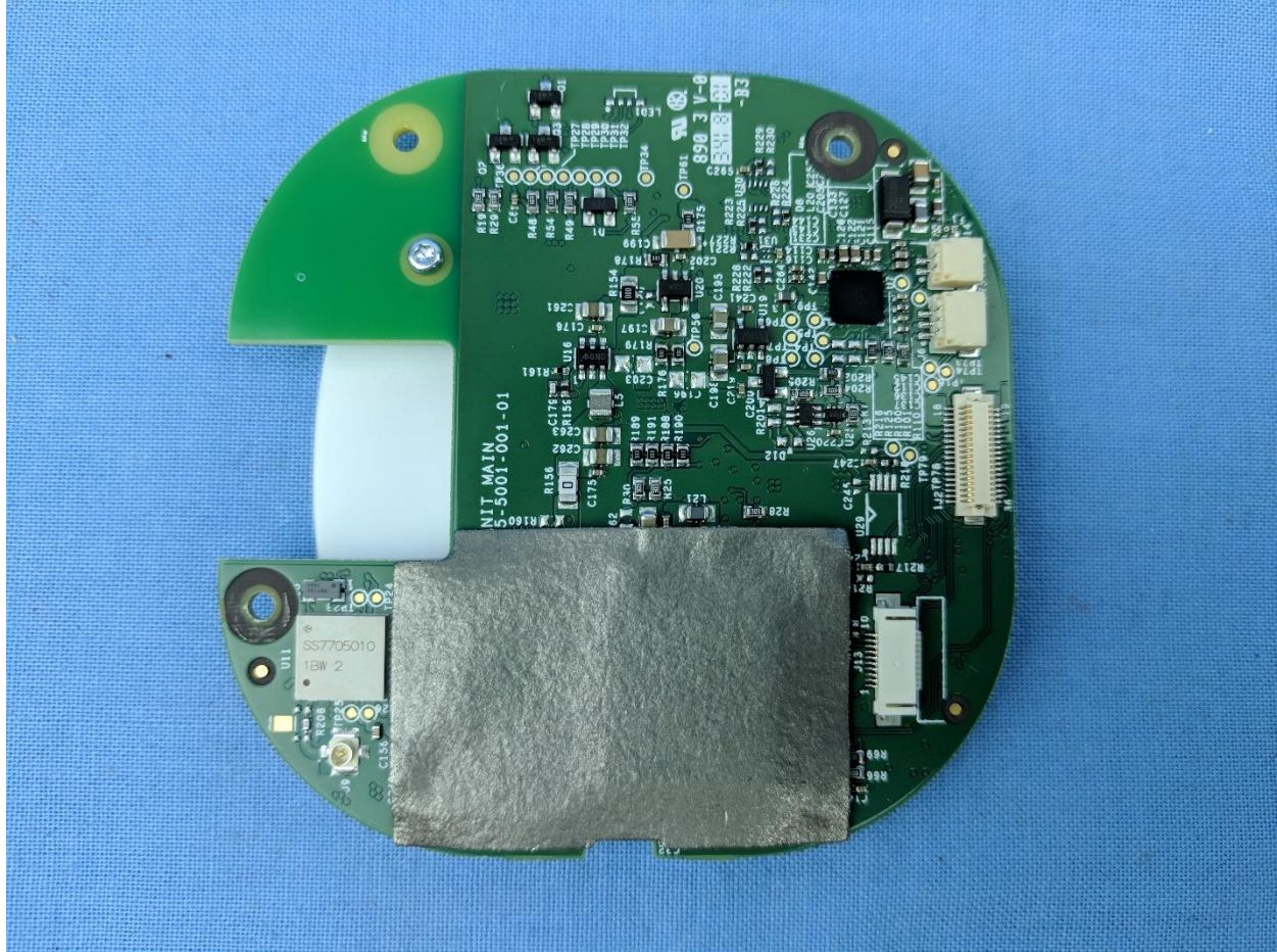
Digital Board Front with Shielding
