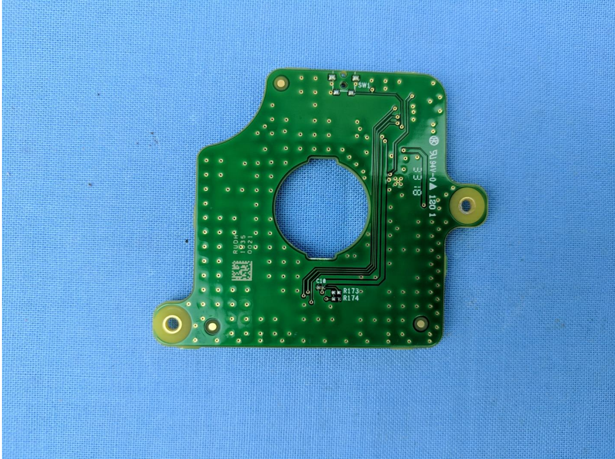
LED Board Back
