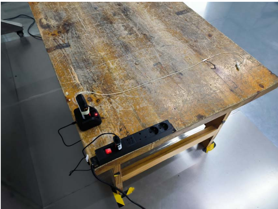
Conducted Emissions Side View With Charging Base
