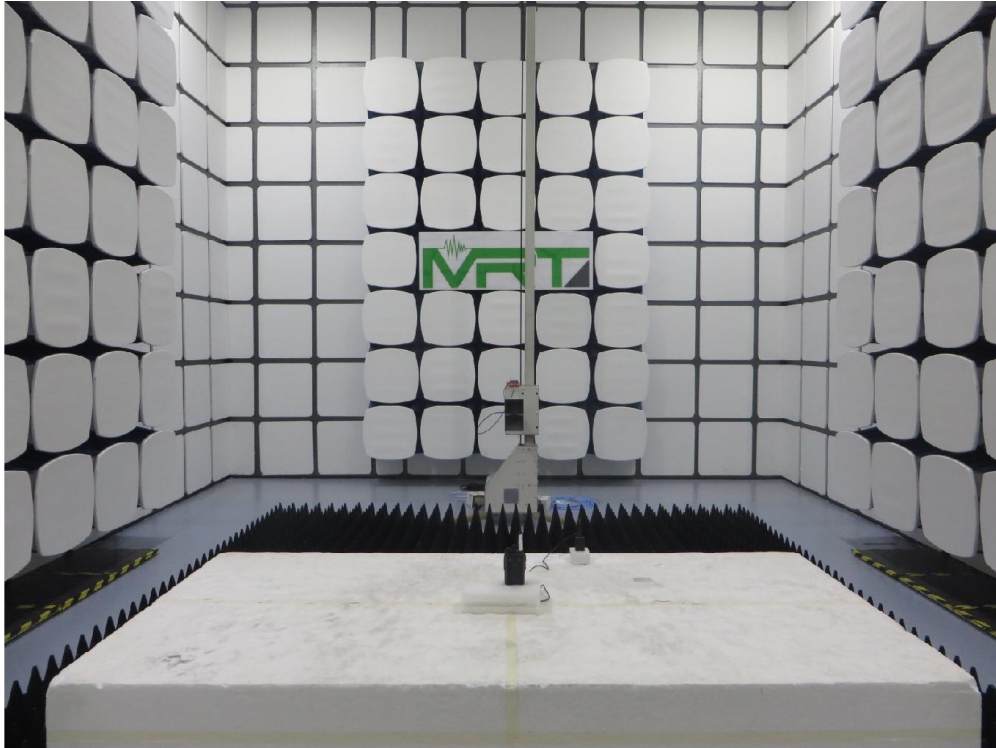
Description: Radiated Emission Test Setup for 1GHz ~ 12.75GHz
