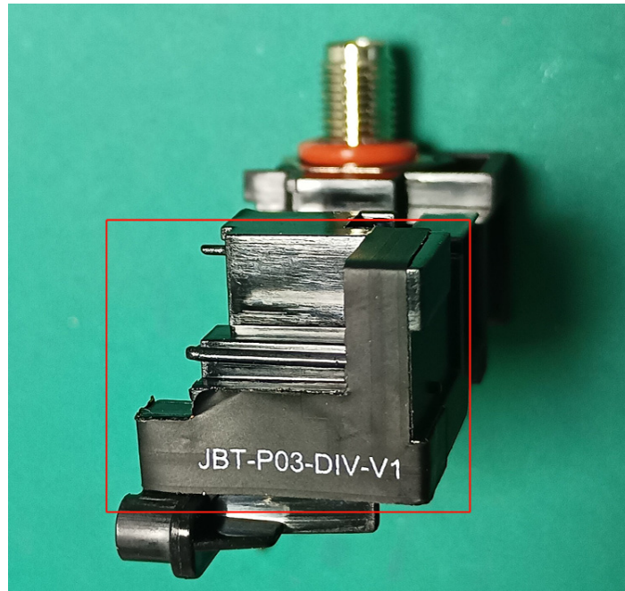
BT/Wi-Fi ANT
