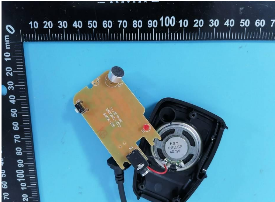
Speaking microphone 2
