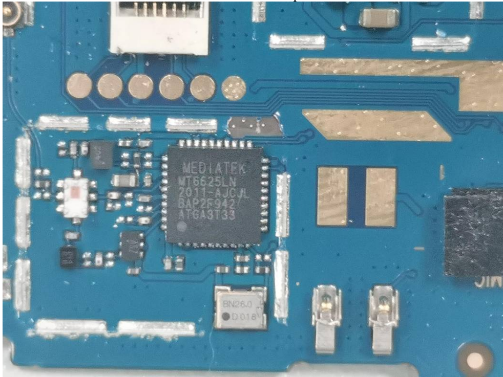
BT&WIFI Chip
