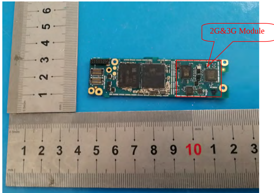
EUT – PCB-2 IC Chip View
