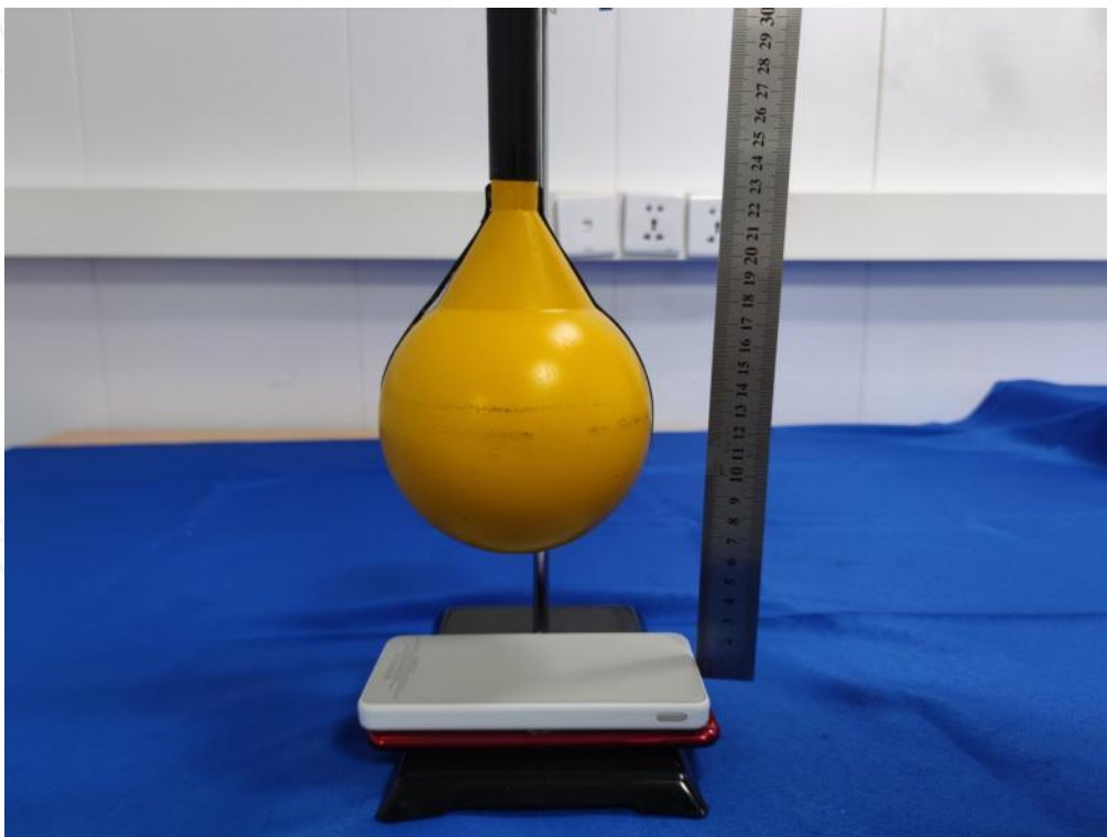
Test Position F(6cm) - Exposure photo from bottom surface(TM10)
