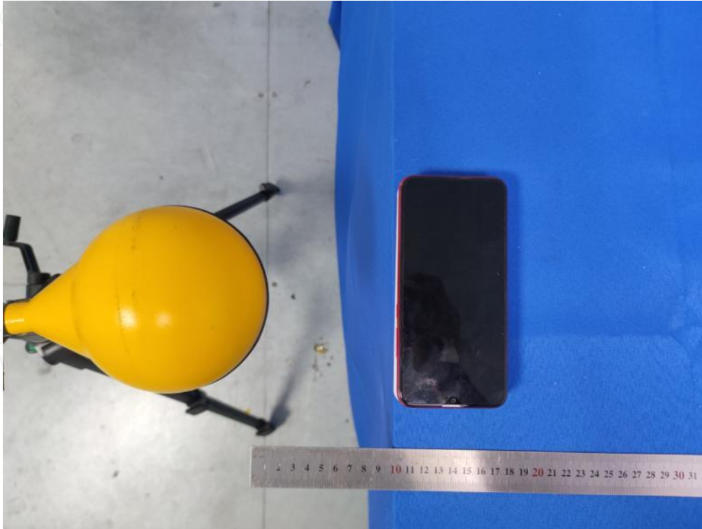
Test Position E(10cm) - Exposure photo from side edge surface-Right(TM10)
