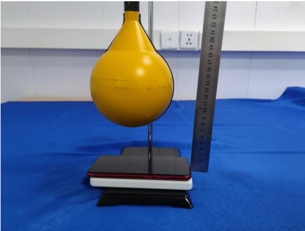
Test Position A (8cm) - Exposure photo from top surface (TM10)
