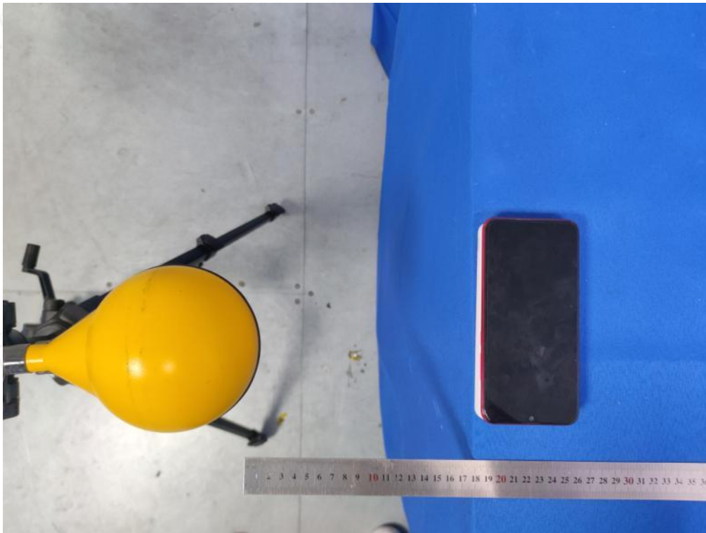
Test Position E(18cm) - Exposure photo from side edge surface-Right(TM10)
