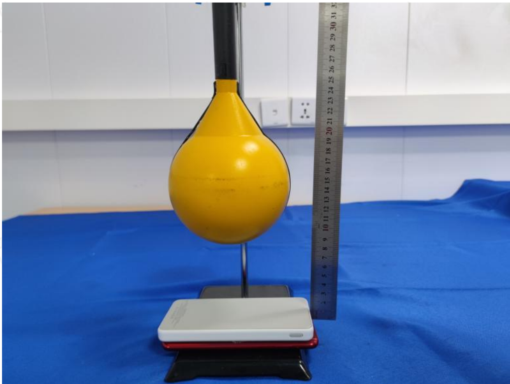
Test Position F(8cm) - Exposure photo from bottom surface(TM10)
