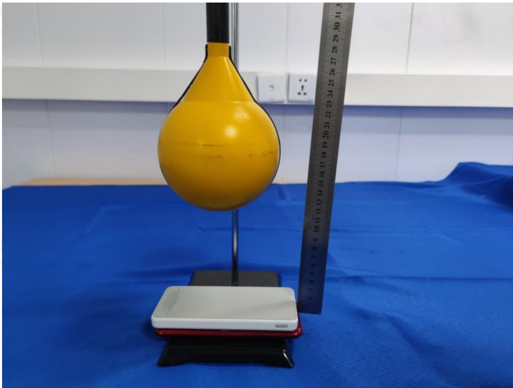
Test Position F(10cm) - Exposure photo from bottom surface(TM10)
