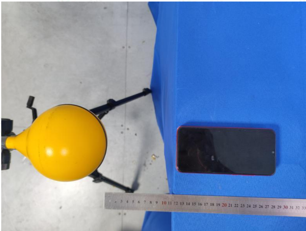
Test Position D(12cm) - Exposure photo from side edge surface-Front(TM10)
