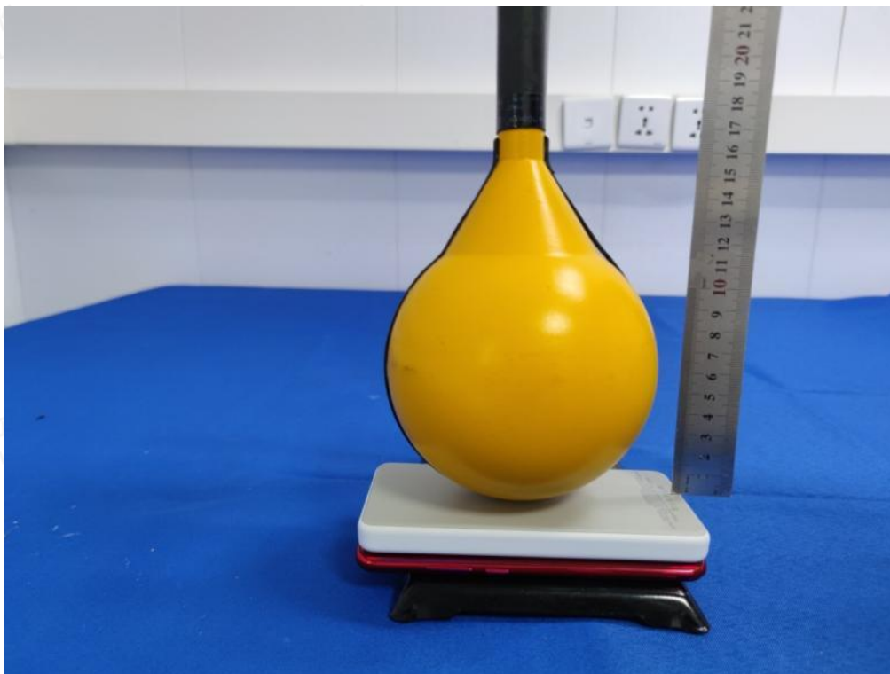
Test Position F(0cm) - Exposure photo from bottom surface(TM10)
