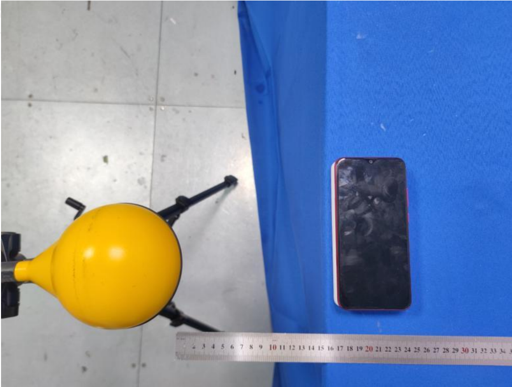
Test Position C(16cm) - Exposure photo from side edge surface-Left(TM10)
