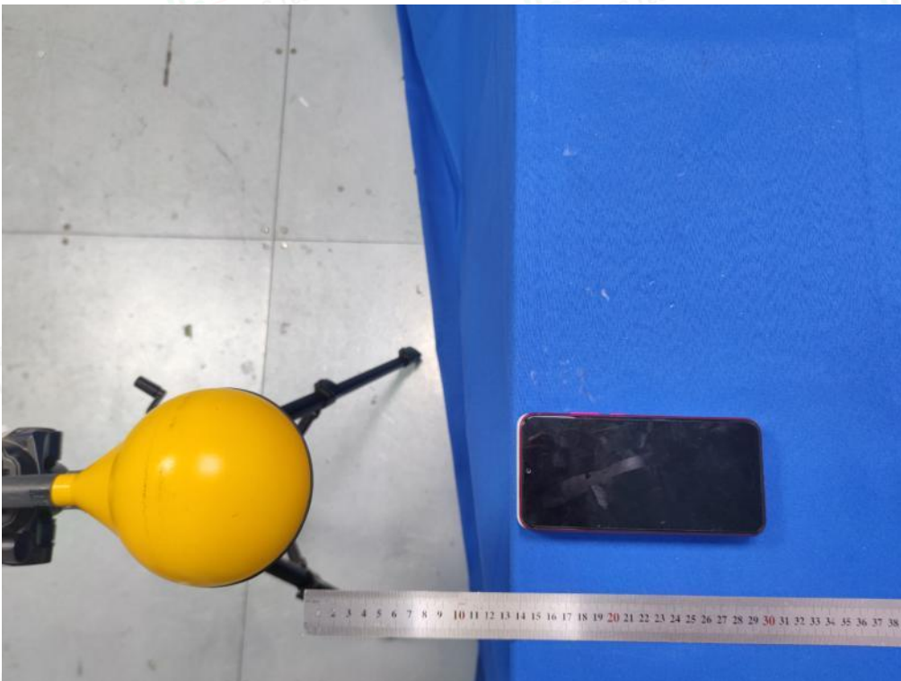
Test Position B(14cm) - Exposure photo from side edge surface-Rear(TM10)
