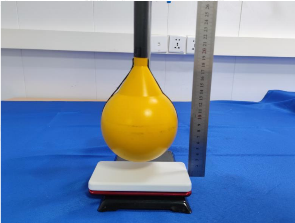
Test Position F(2cm) - Exposure photo from bottom surface(TM10)
