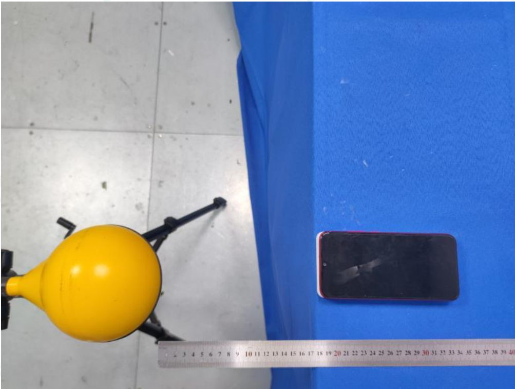
Test Position B(18cm) - Exposure photo from side edge surface-Rear(TM10)
