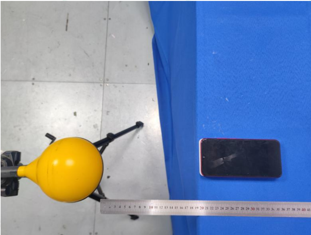
Test Position B(20cm) - Exposure photo from side edge surface-Rear(TM10)
