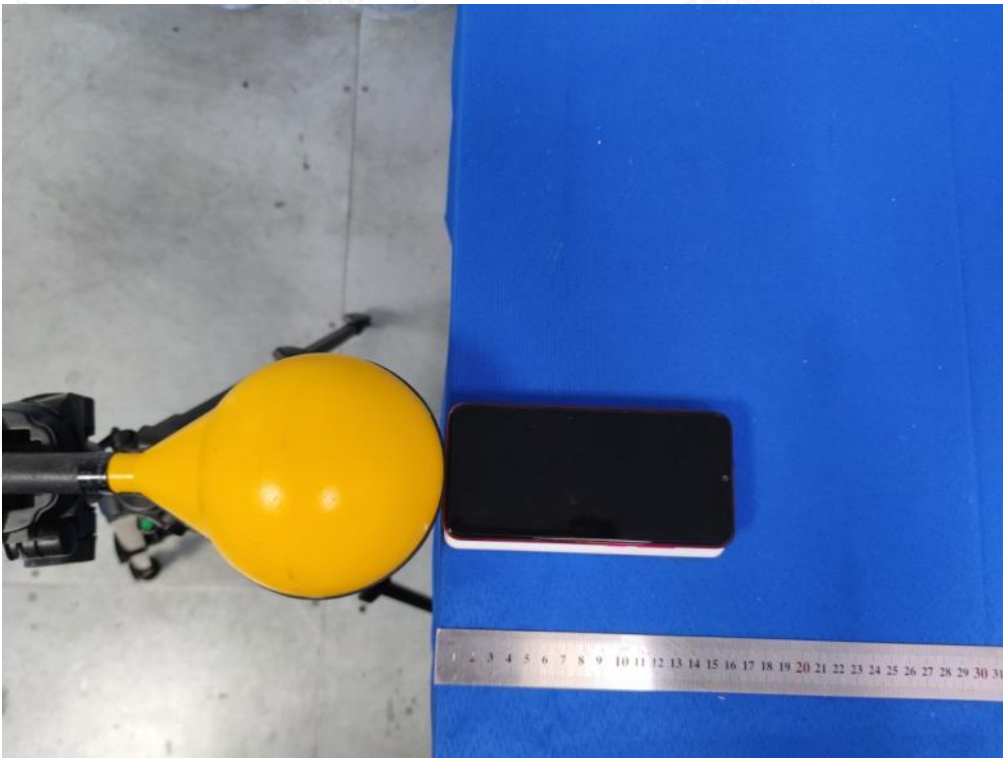
Test Position B(0cm) - Exposure photo from side edge surface-Rear(TM10)
