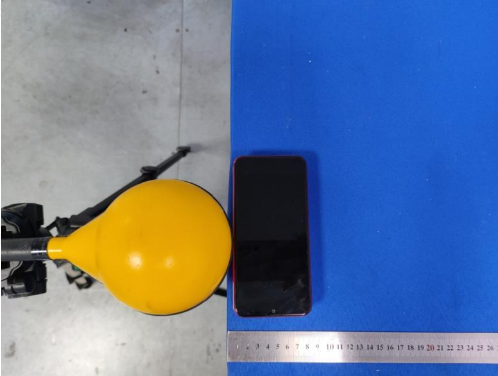
Test Position C(0cm) - Exposure photo from side edge surface-Left(TM10)
