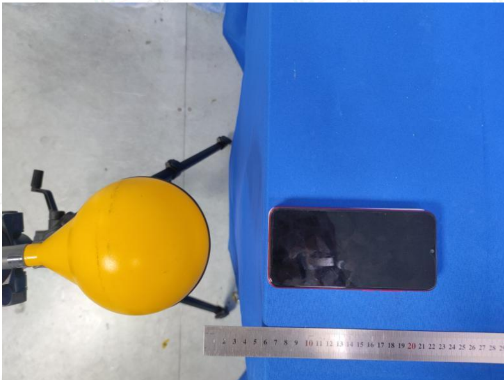
Test Position D(6cm) - Exposure photo from side edge surface-Front(TM10)
