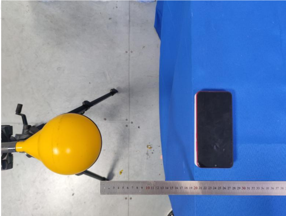
Test Position E(20cm) - Exposure photo from side edge surface-Right(TM10)
