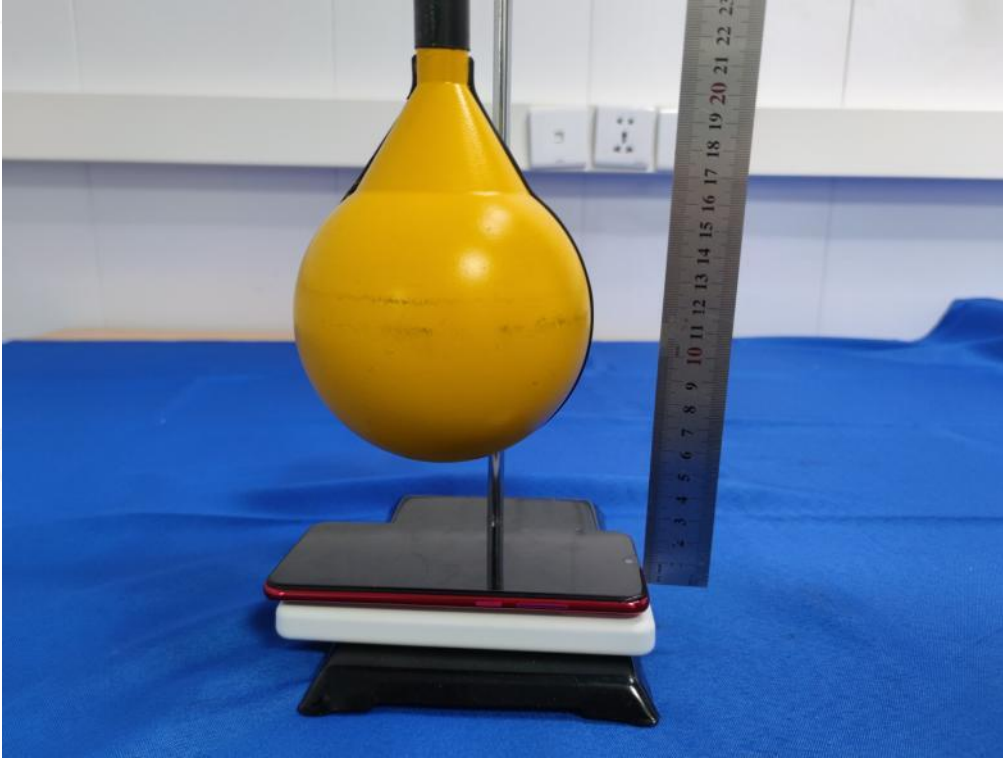
Test Position A (6cm) - Exposure photo from top surface (TM10)
