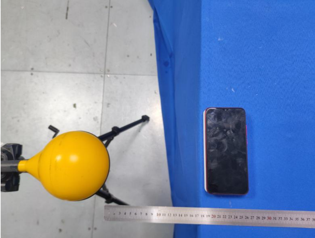
Test Position C(18cm) - Exposure photo from side edge surface-Left(TM10)
