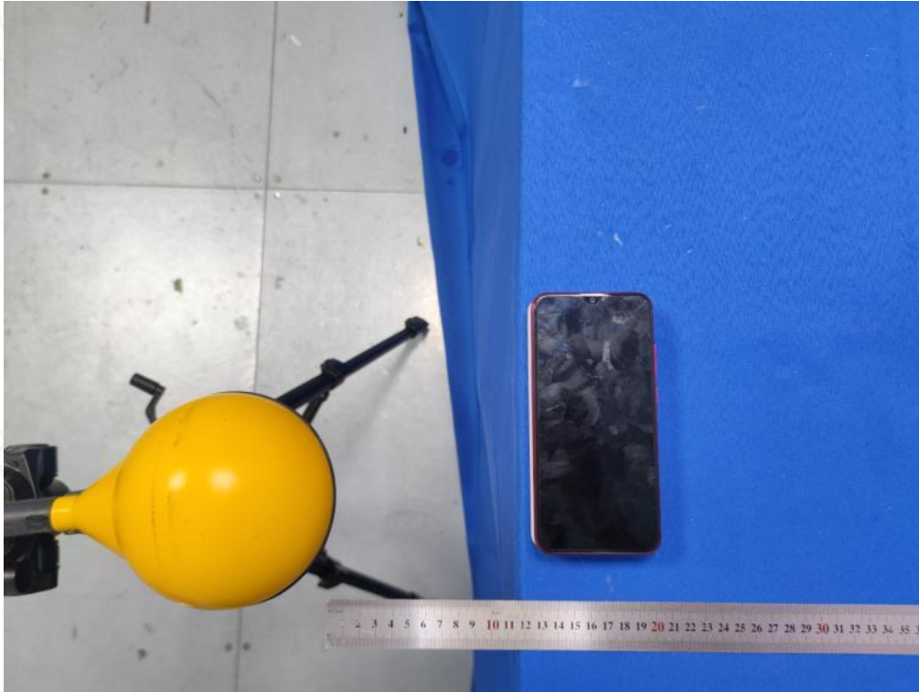
Test Position C(12cm) - Exposure photo from side edge surface-Left(TM10)
