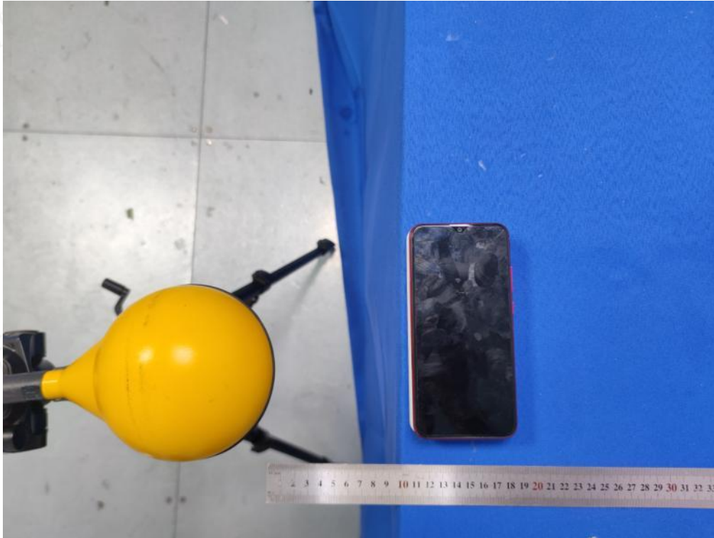
Test Position C(10cm) - Exposure photo from side edge surface-Left(TM10)
