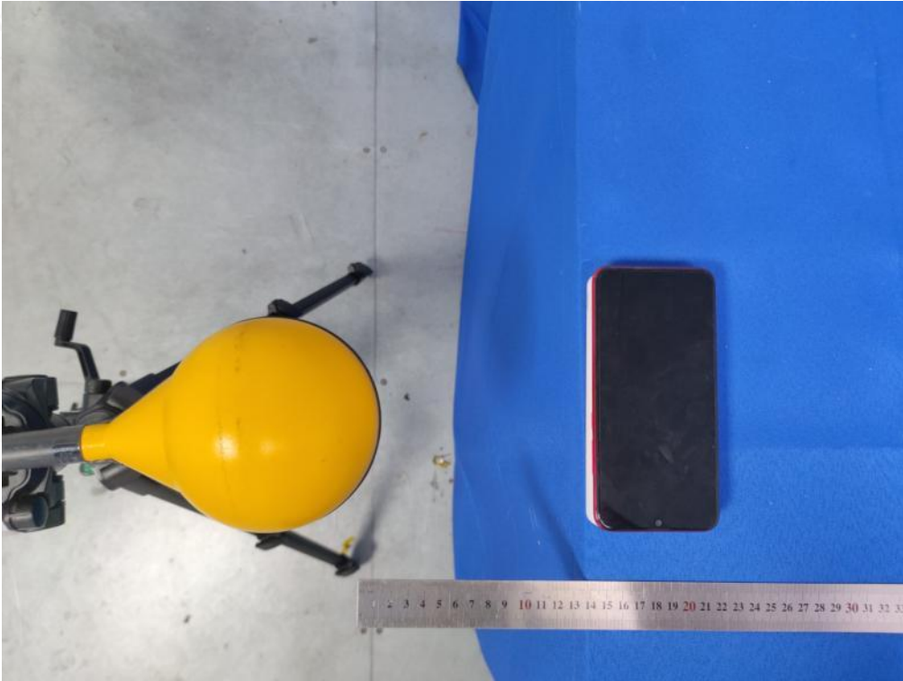
Test Position E(14cm) - Exposure photo from side edge surface-Right(TM10)
