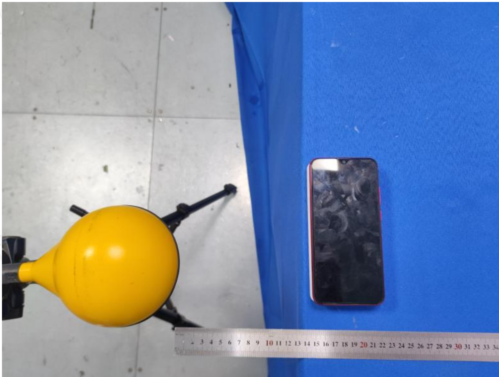
Test Position C(14cm) - Exposure photo from side edge surface-Left(TM10)
