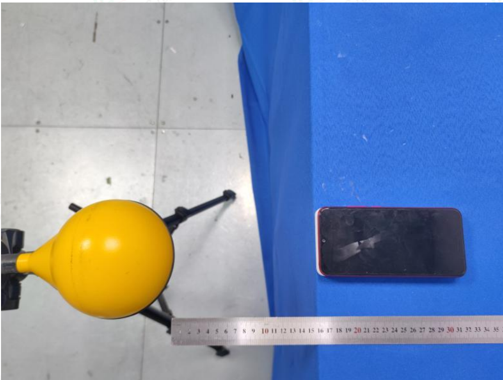
Test Position B(16cm) - Exposure photo from side edge surface-Rear(TM10)
