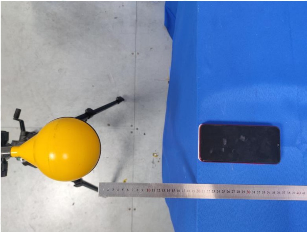
Test Position D(20cm) - Exposure photo from side edge surface-Front(TM10)
