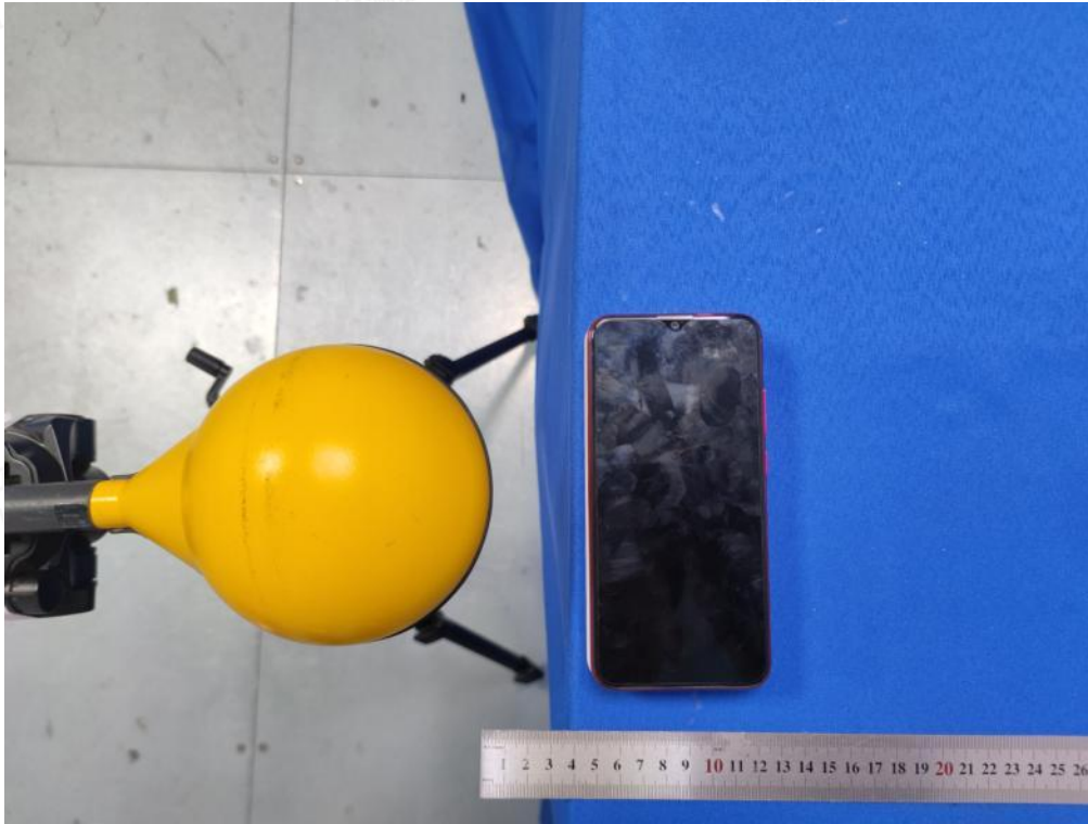
Test Position C(4cm) - Exposure photo from side edge surface-Left(TM10)
