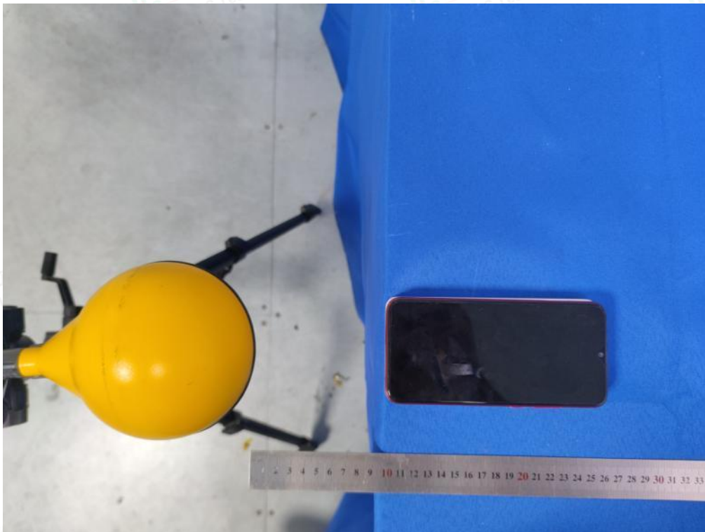
Test Position D(10cm) - Exposure photo from side edge surface-Front(TM10)
