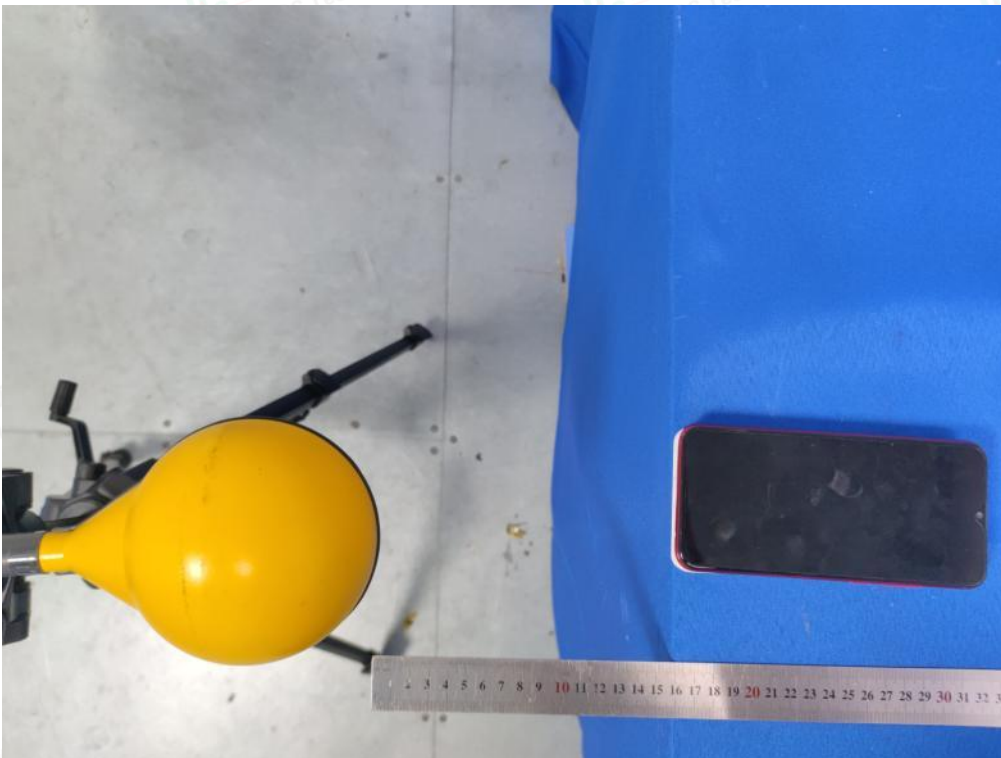
Test Position D(16cm) - Exposure photo from side edge surface-Front(TM10)
