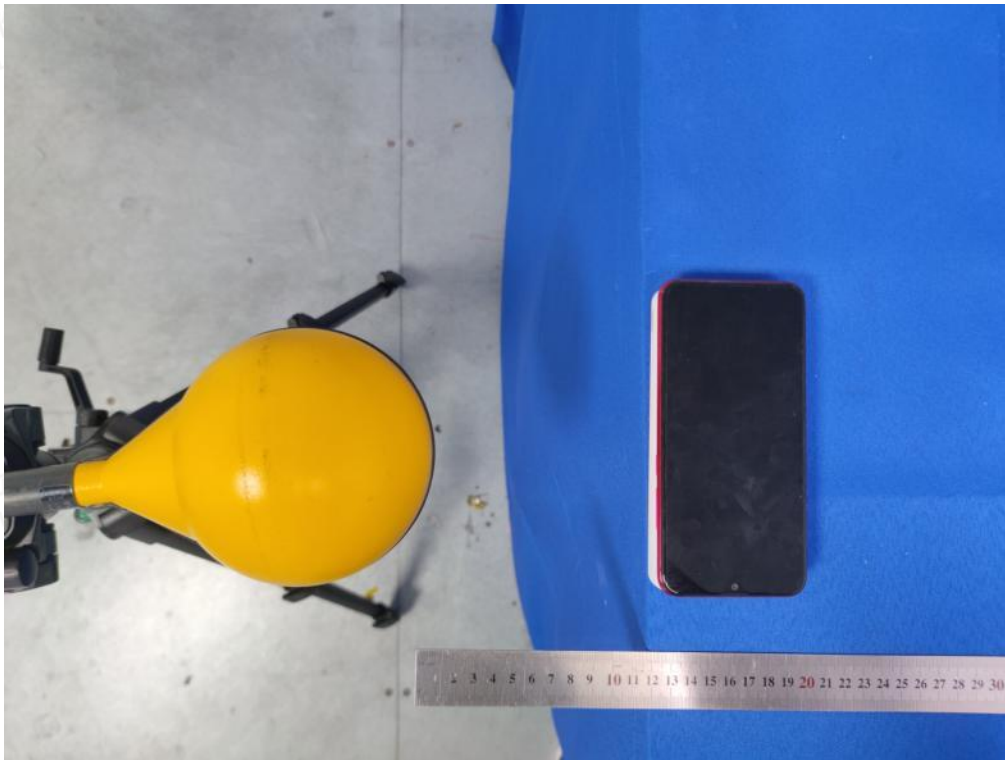
Test Position E(12cm) - Exposure photo from side edge surface-Right(TM10)
