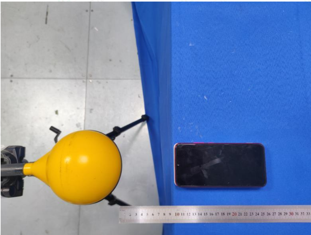
Test Position B(10cm) - Exposure photo from side edge surface-Rear(TM10)
