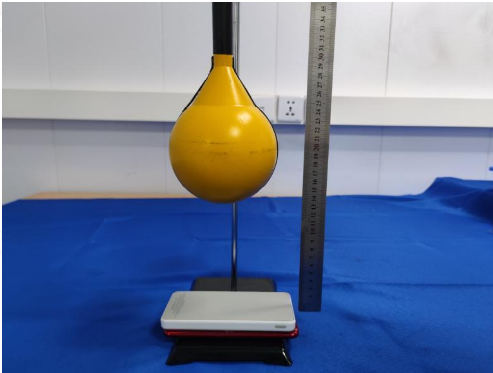
Test Position F(12cm) - Exposure photo from bottom surface(TM10)
