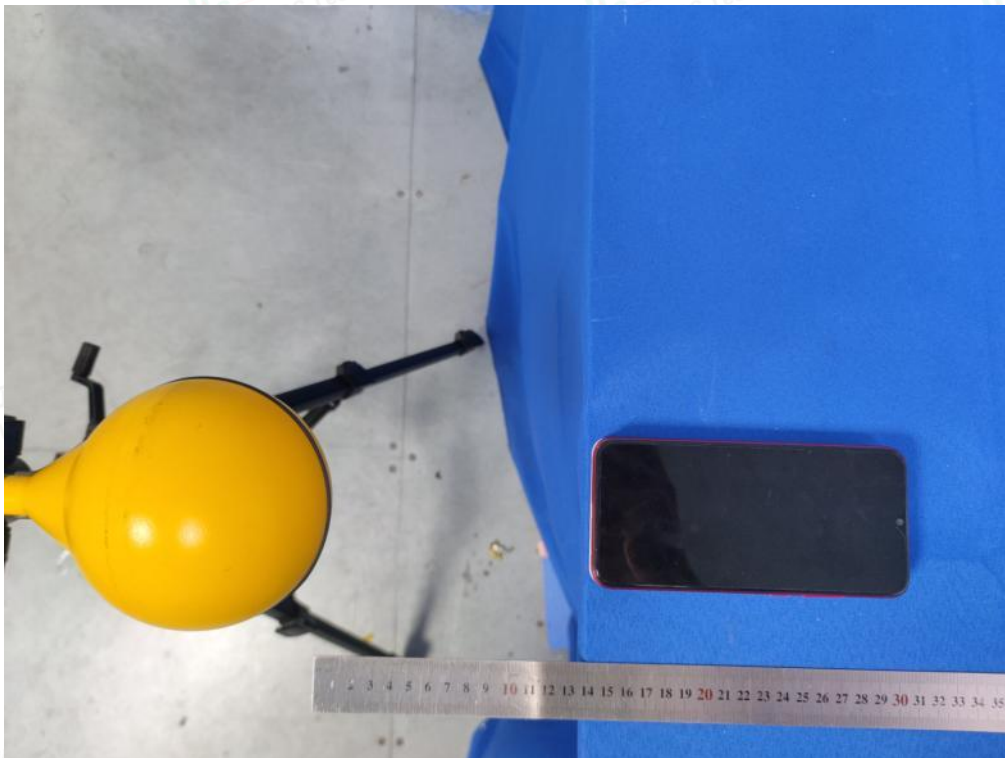
Test Position D(14cm) - Exposure photo from side edge surface-Front(TM10)
