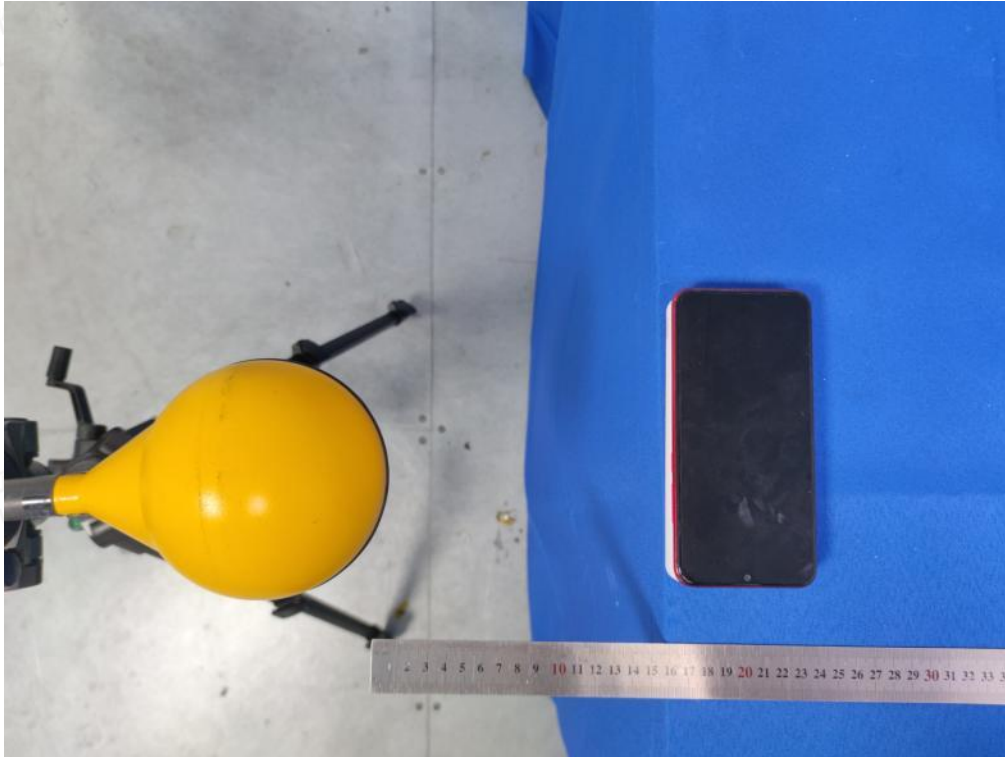
Test Position E(16cm) - Exposure photo from side edge surface-Right(TM10)
