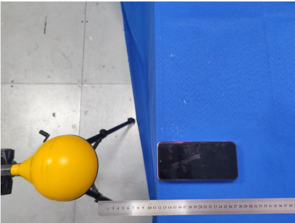
Test Position B(12cm) - Exposure photo from side edge surface-Rear(TM10)
