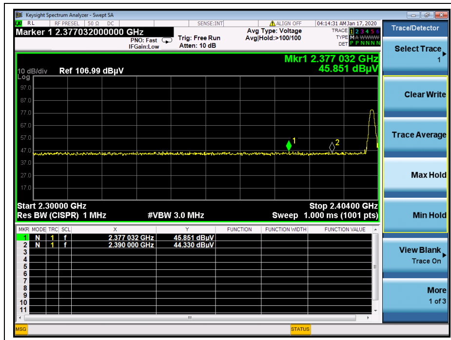
(PEAK, Channel = 0, π/4-DQPSK)
