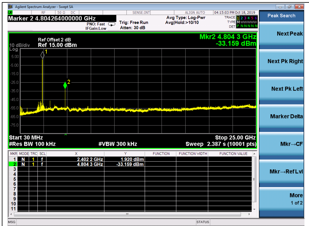
(Channel = 0, 30MHz to 25GHz, GFSK Mode)
