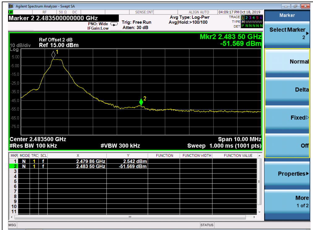
(Channel = 78, Band edge, GFSK Mode)
