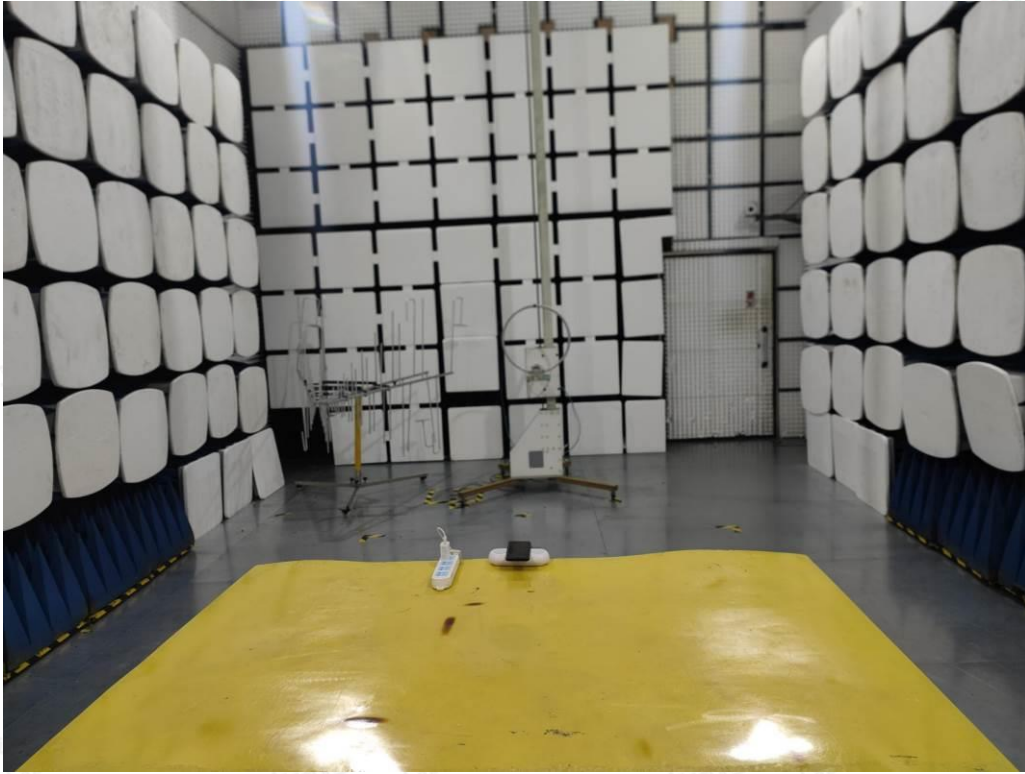
Radiated Emission
