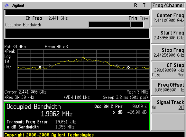
20dB Bandwidth plot on channel 39 (2Mbps)
