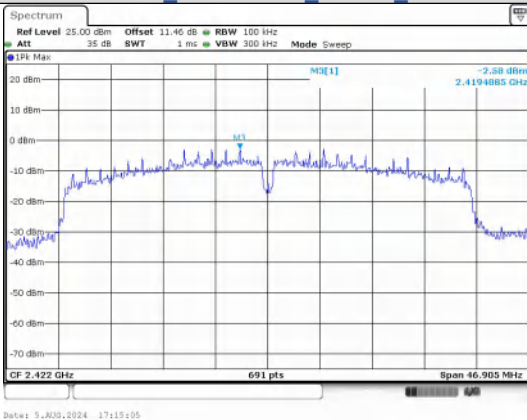
In-Band Reference Level IEEE 802.11n Channel 3 40MHz Antenna 0
