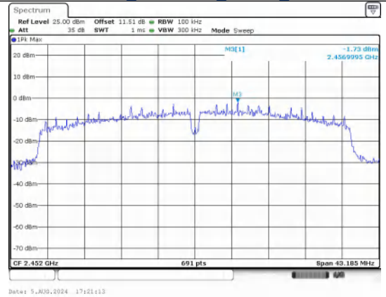
In-Band Reference Level IEEE 802.11n Channel 9 40MHz Antenna 0
