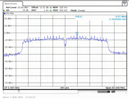
In-Band Reference Level IEEE 802.11n Channel 6 40MHz Antenna 0
