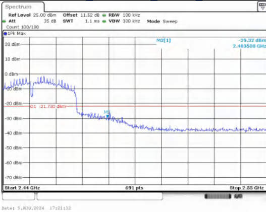
Out Of Band Emission IEEE 802.11n Channel 9 40MHz Antenna 0
