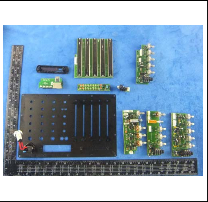
Cover Off - Top View 2
