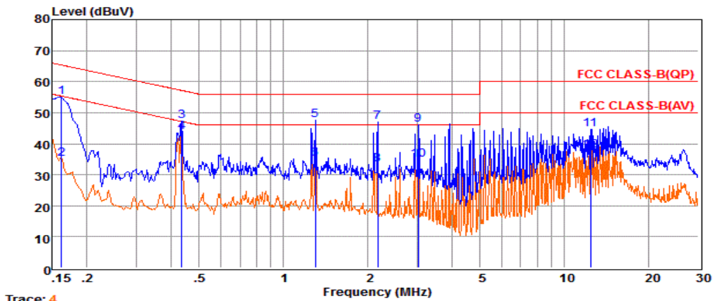
Trace: 4 Pol: NEUTRAL
