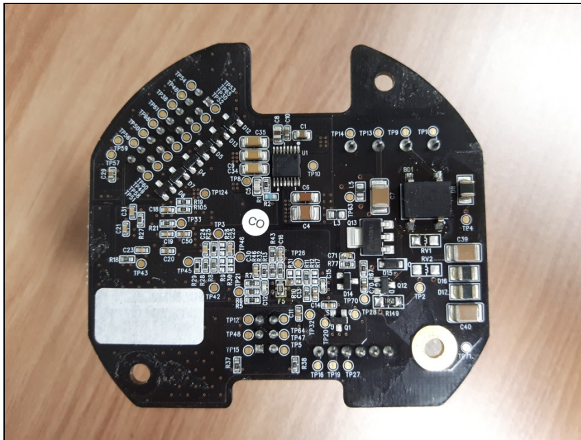
Bottom view of Host (Sub board)
