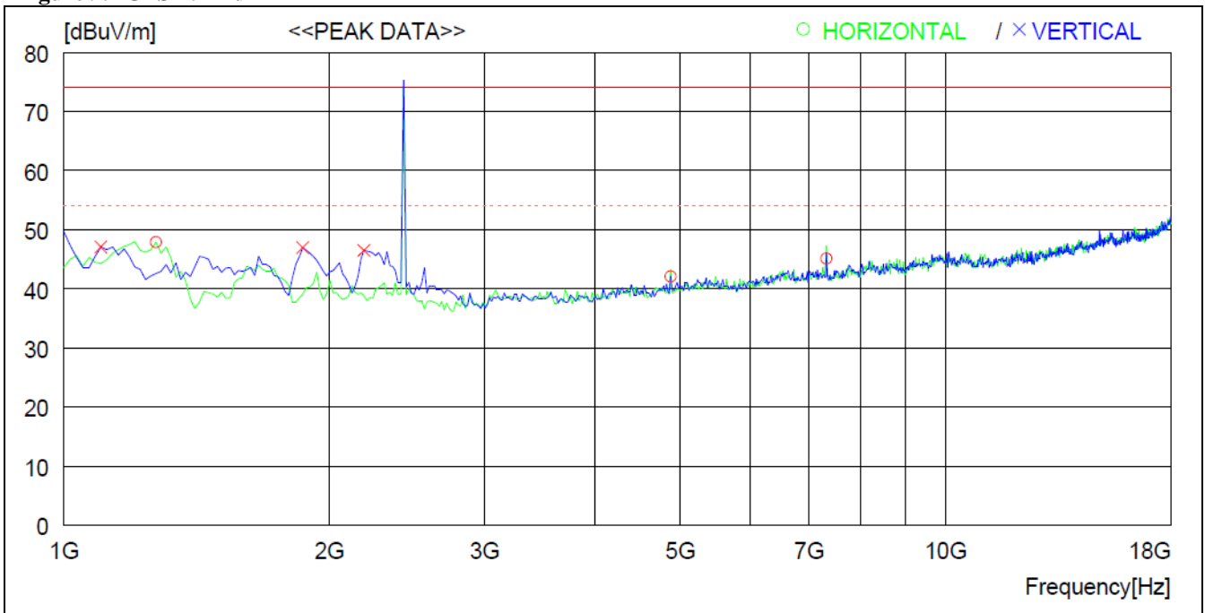
Figure 9. GFSK: Mid
