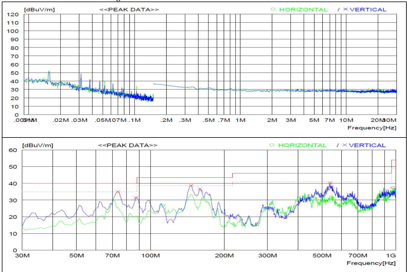
Figure 5. Test data for Radiated emission below 1GHz
