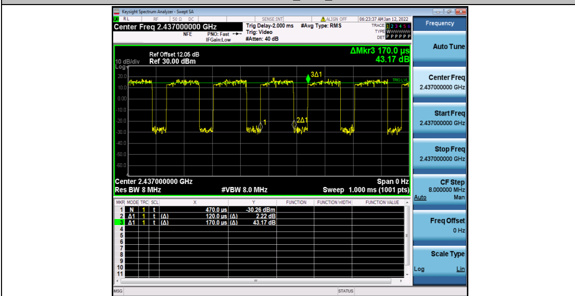
11AC40SISO_Ant1_2437
