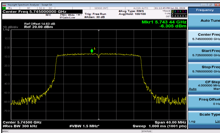
11AX20SISO-Ant1-5745-PASS
