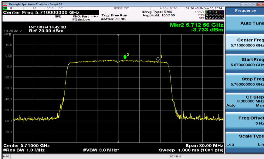
11AX40SISO-Ant1-5710_UNII-2C-PASS
