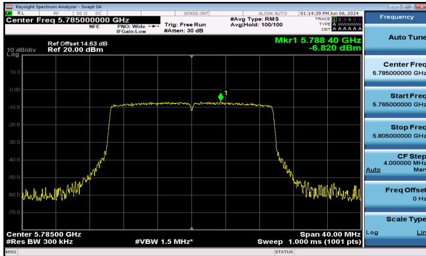
11AX20SISO-Ant1-5785-PASS
