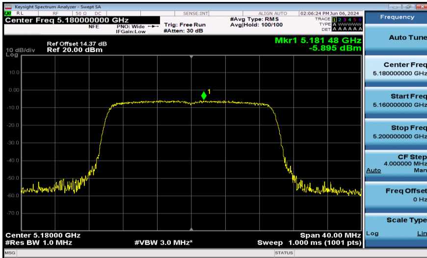
11AX20SISO-Ant1-5180-242Tone-PASS
