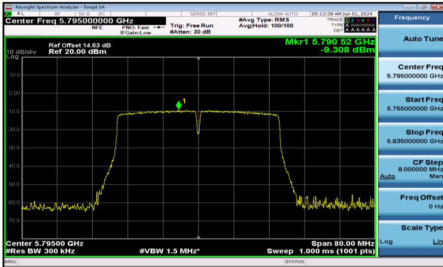
11AC40SISO-Ant1-5795-PASS
