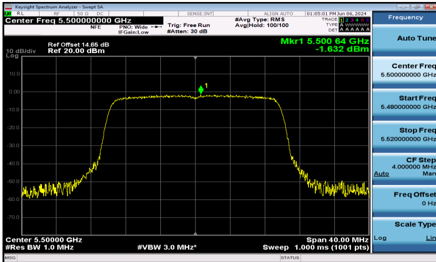
11AX20SISO-Ant1-5500-PASS
