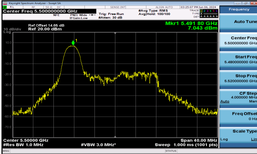
11AX20SISO-Ant1-5500-26Tone-PASS
