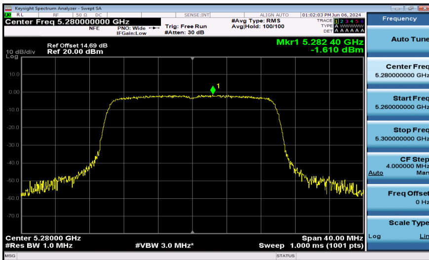
11AX20SISO-Ant1-5280-PASS
