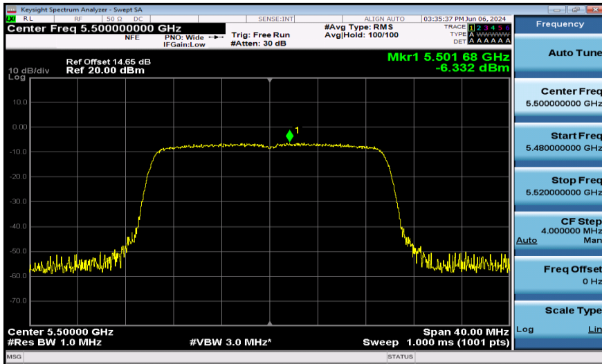
11AX20SISO-Ant1-5500-242Tone-PASS
