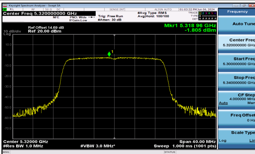
11AX20SISO-Ant1-5320-PASS
