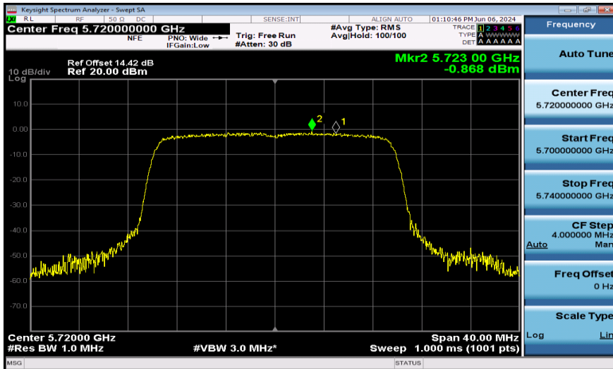
11AX20SISO-Ant1-5720_UNII-2C-PASS
