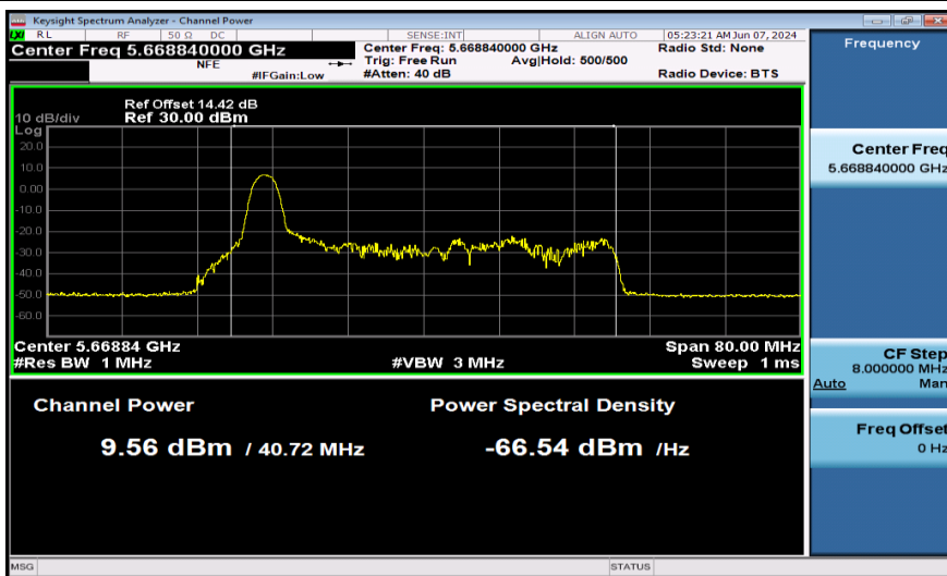
11AX40SISO-Ant1-5670-26Tone-PASS
