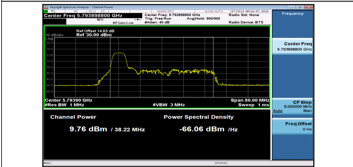
11AX40SISO-Ant1-5795-52Tone-PASS
