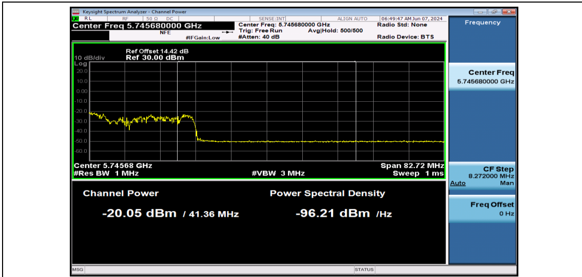
11AX40SISO-Ant1-5710_UNII-3-106Tone-PASS
