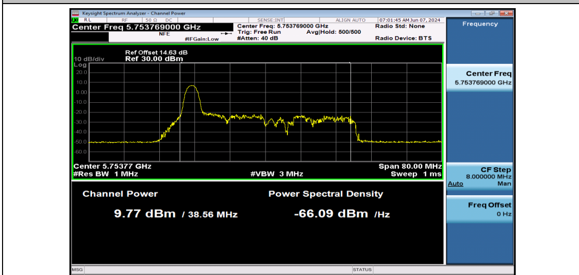
11AX40SISO-Ant1-5755-26Tone-PASS
