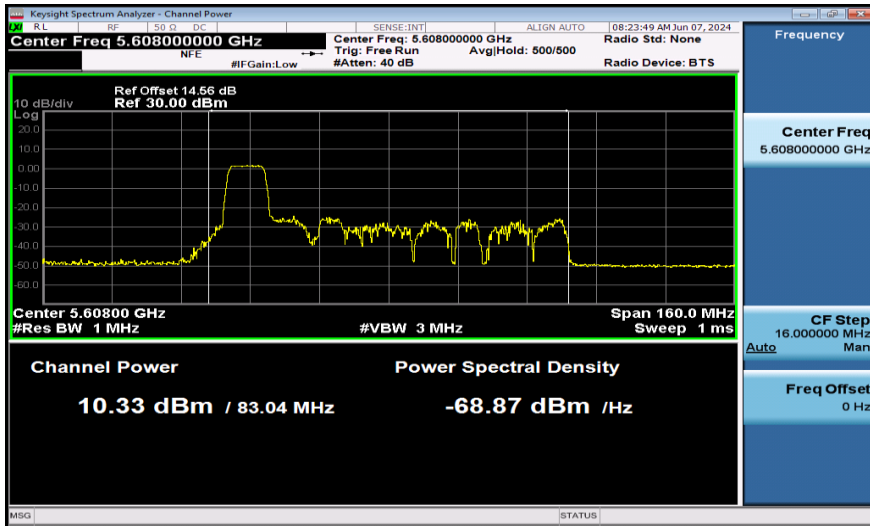
11AX80SISO-Ant1-5610-106Tone-PASS
