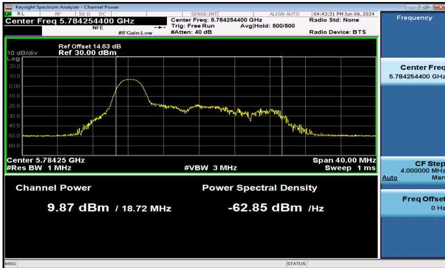
11AX20SISO-Ant1-5785-26Tone-PASS
