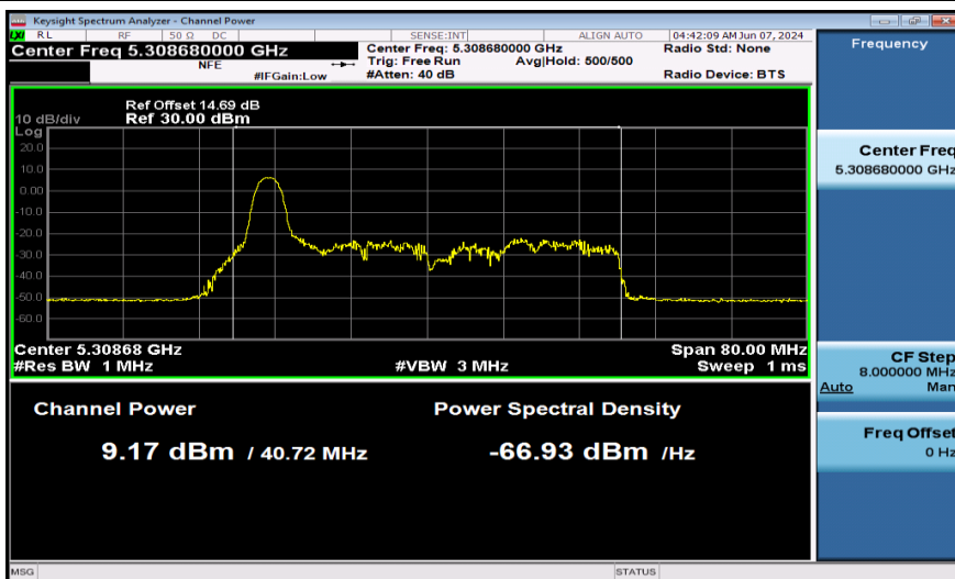
11AX40SISO-Ant1-5310-26Tone-PASS
