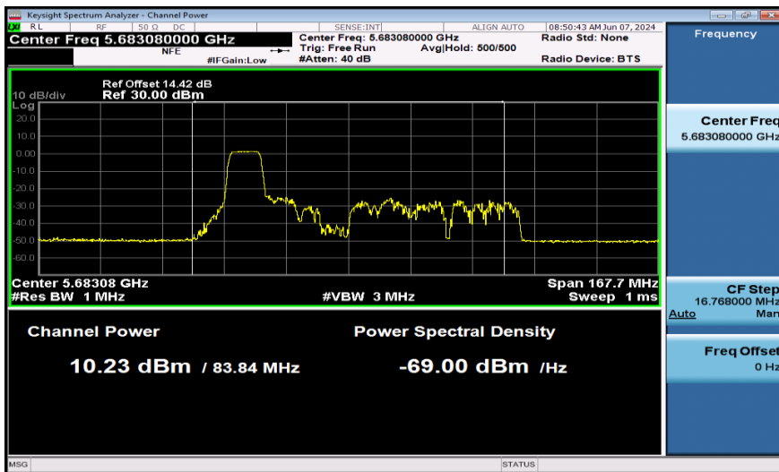
11AX80SISO-Ant1-5690_UNII-2C-106Tone-PASS
