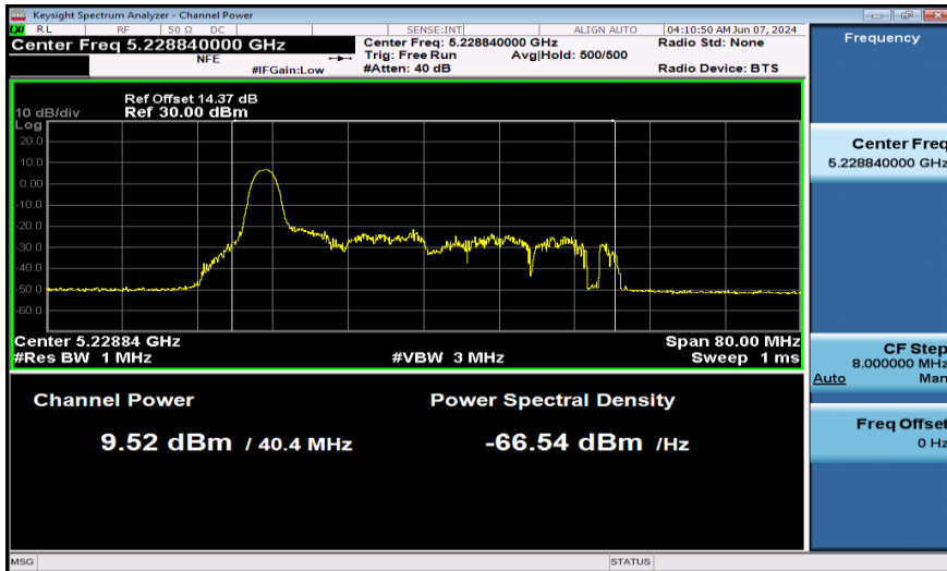
11AX40SISO-Ant1-5230-26Tone-PASS
