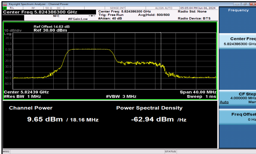
11AX20SISO-Ant1-5825-106Tone-PASS
