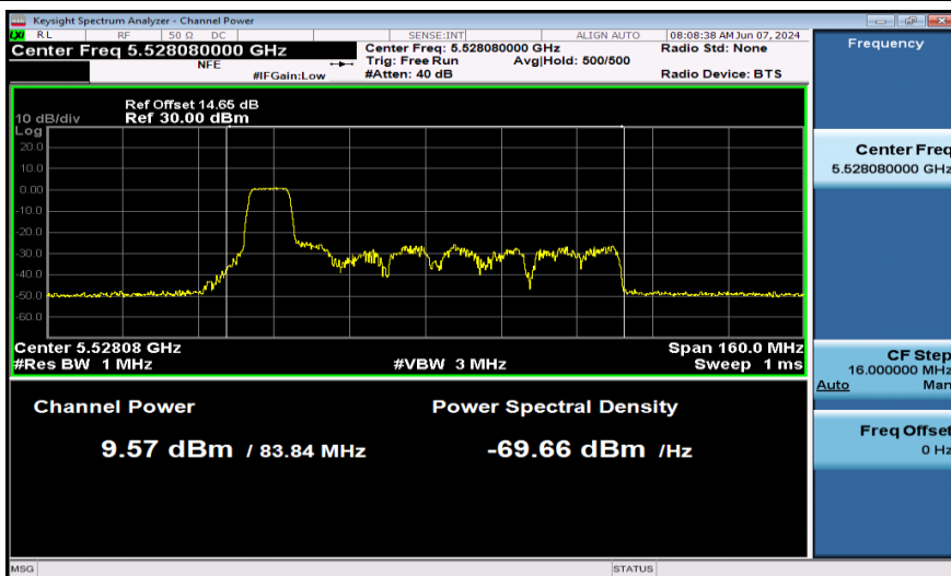
11AX80SISO-Ant1-5530-106Tone-PASS
