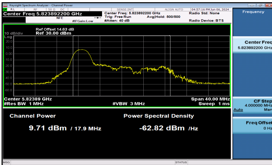
11AX20SISO-Ant1-5825-26Tone-PASS
