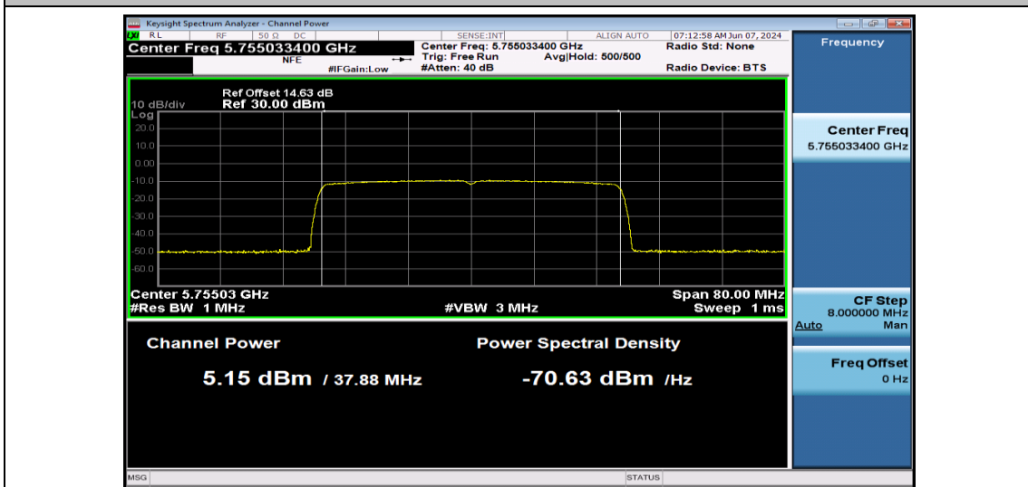
11AX40SISO-Ant1-5755-484Tone-PASS
