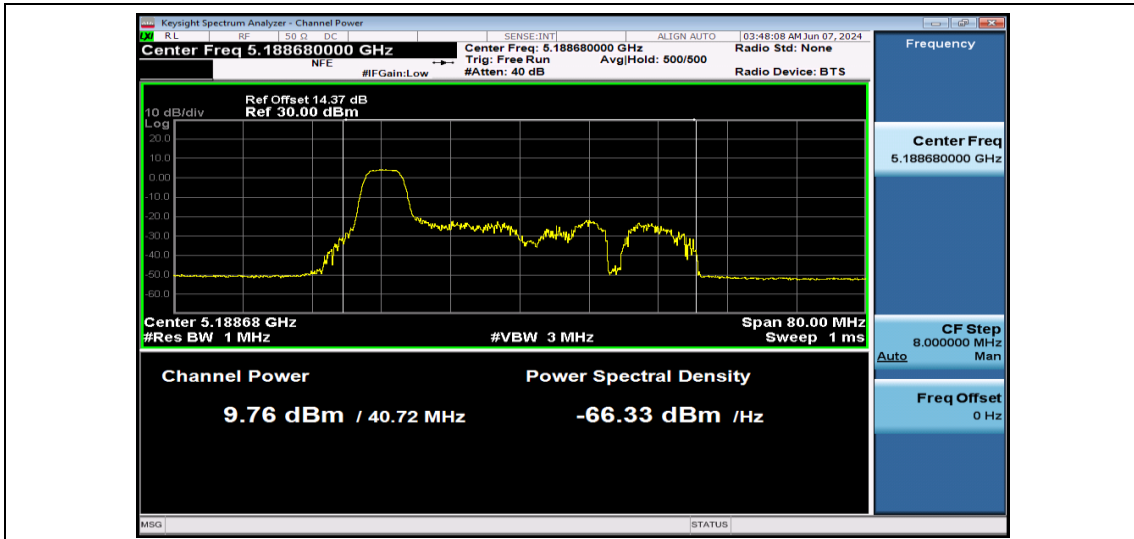
11AX40SISO-Ant1-5190-52Tone-PASS
