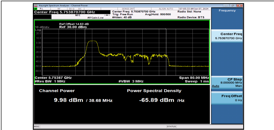
11AX40SISO-Ant1-5755-52Tone-PASS
