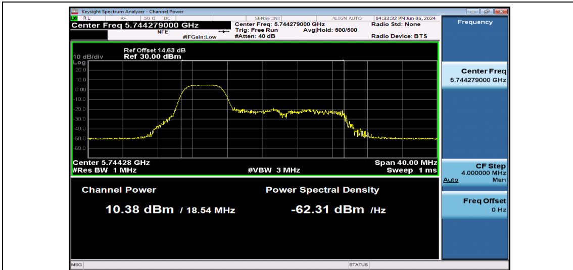
11AX20SISO-Ant1-5745-52Tone-PASS
