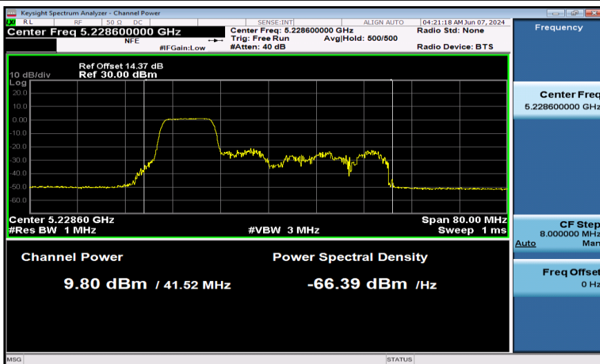
11AX40SISO-Ant1-5230-106Tone-PASS
