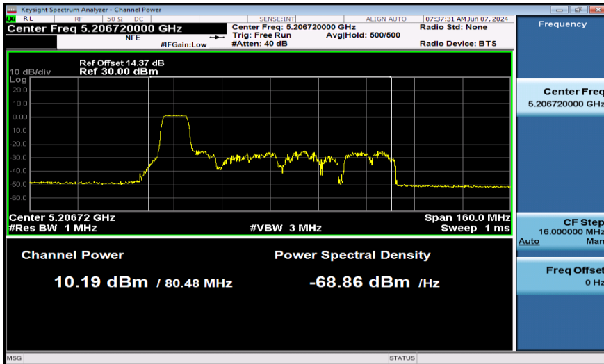
11AX80SISO-Ant1-5210-106Tone-PASS
