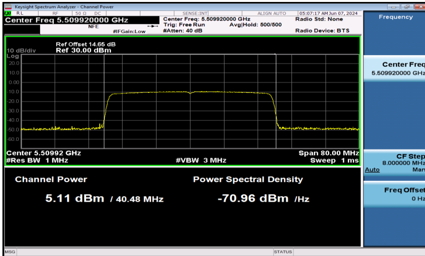
11AX40SISO-Ant1-5510-484Tone-PASS
