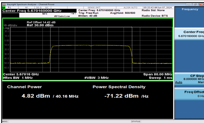
11AX40SISO-Ant1-5670-484Tone-PASS
