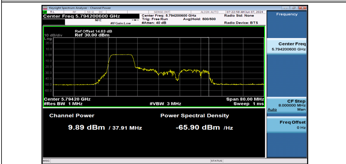
11AX40SISO-Ant1-5795-106Tone-PASS
