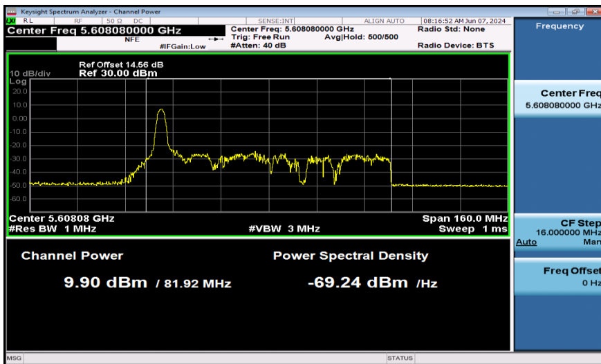
11AX80SISO-Ant1-5610-26Tone-PASS
