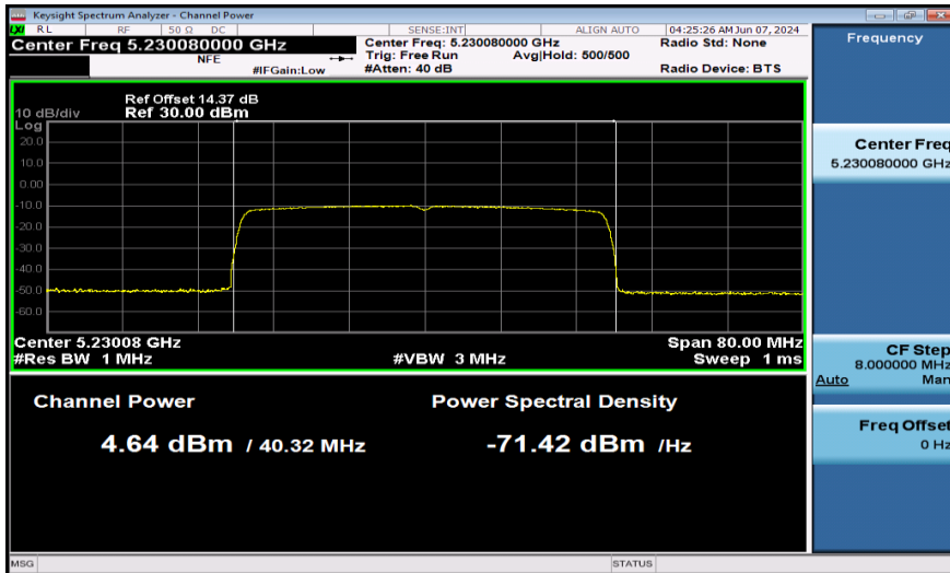
11AX40SISO-Ant1-5230-484Tone-PASS
