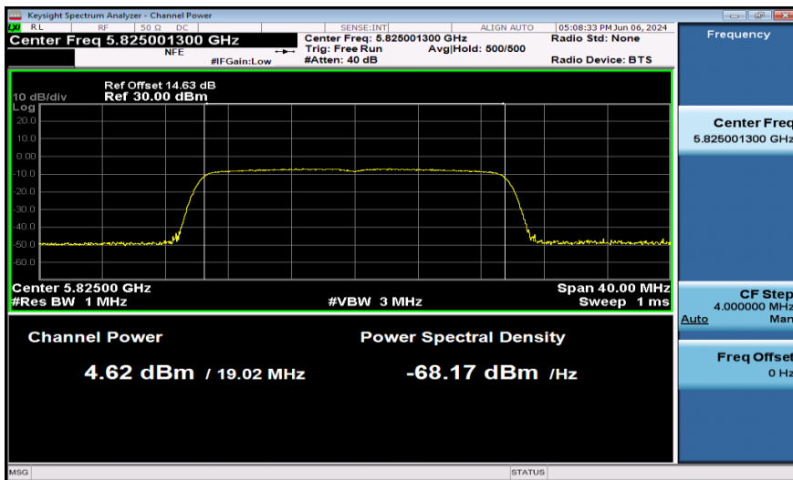
11AX20SISO-Ant1-5825-242Tone-PASS
