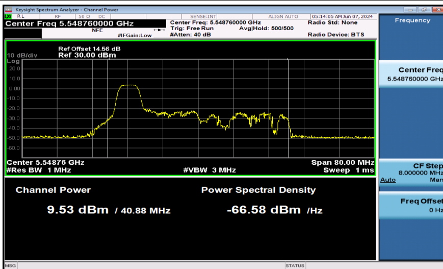
11AX40SISO-Ant1-5550-52Tone-PASS
