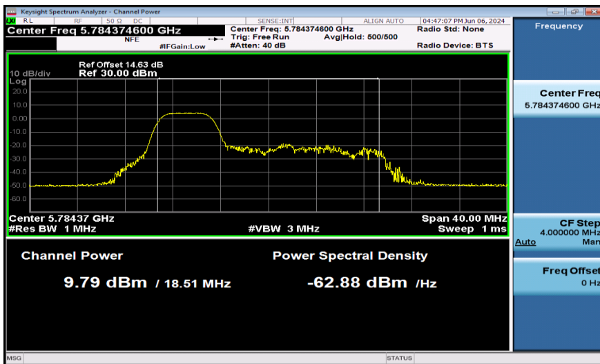
11AX20SISO-Ant1-5785-52Tone-PASS
