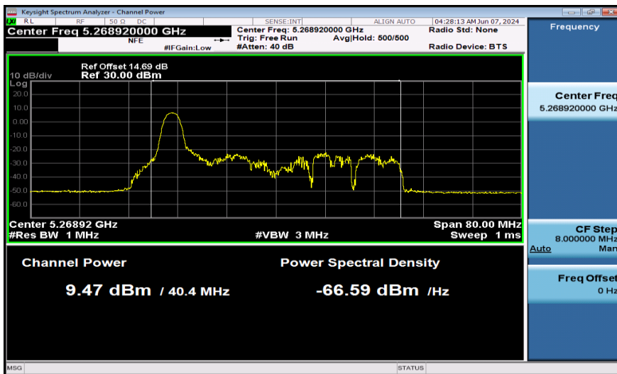
11AX40SISO-Ant1-5270-26Tone-PASS
