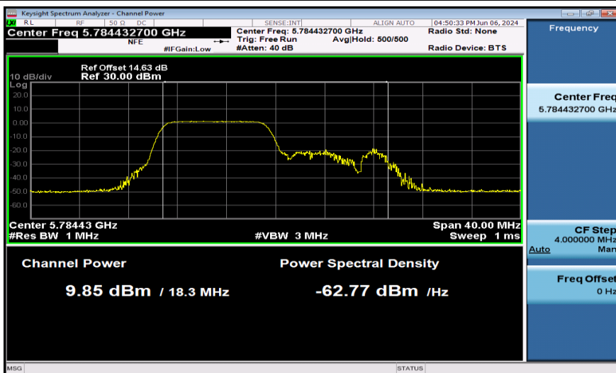
11AX20SISO-Ant1-5785-106Tone-PASS
