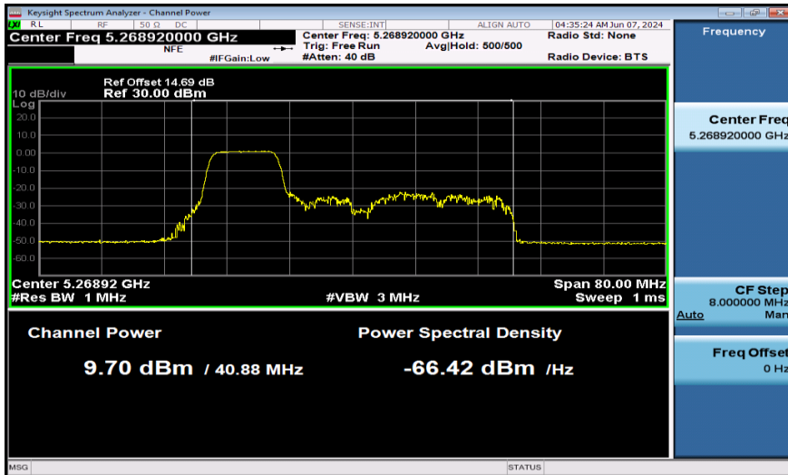
11AX40SISO-Ant1-5270-106Tone-PASS
