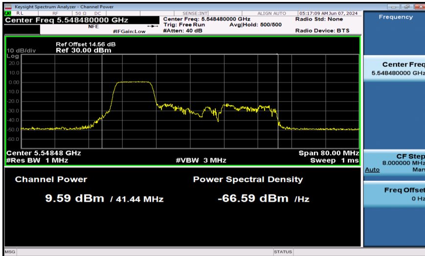
11AX40SISO-Ant1-5550-106Tone-PASS
