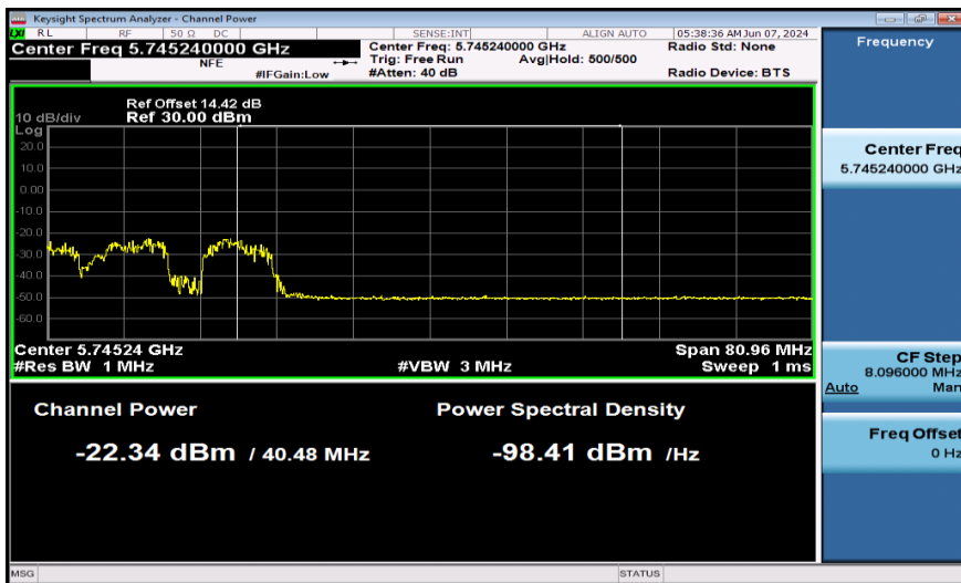
11AX40SISO-Ant1-5710_UNII-3-26Tone-PASS
