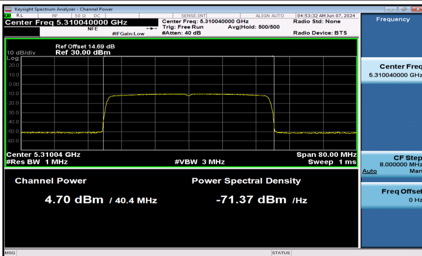
11AX40SISO-Ant1-5310-484Tone-PASS
