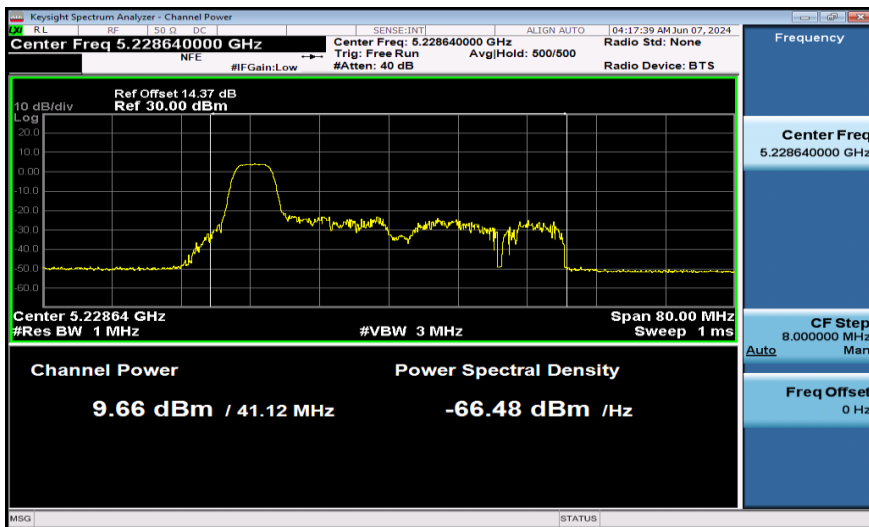
11AX40SISO-Ant1-5230-52Tone-PASS
