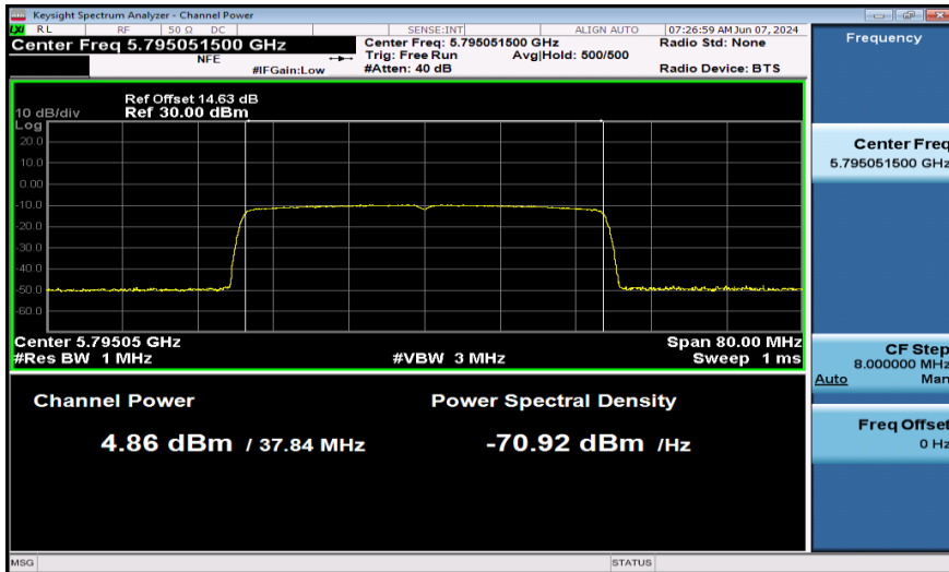
11AX40SISO-Ant1-5795-484Tone-PASS
