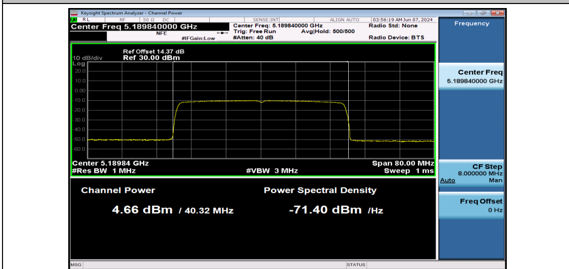
11AX40SISO-Ant1-5190-484Tone-PASS
