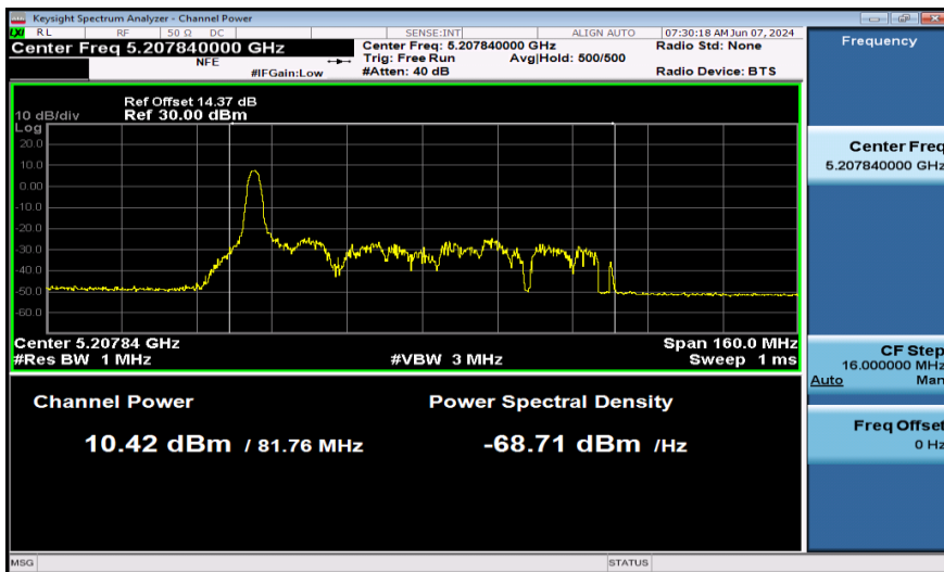
11AX80SISO-Ant1-5210-26Tone-PASS
