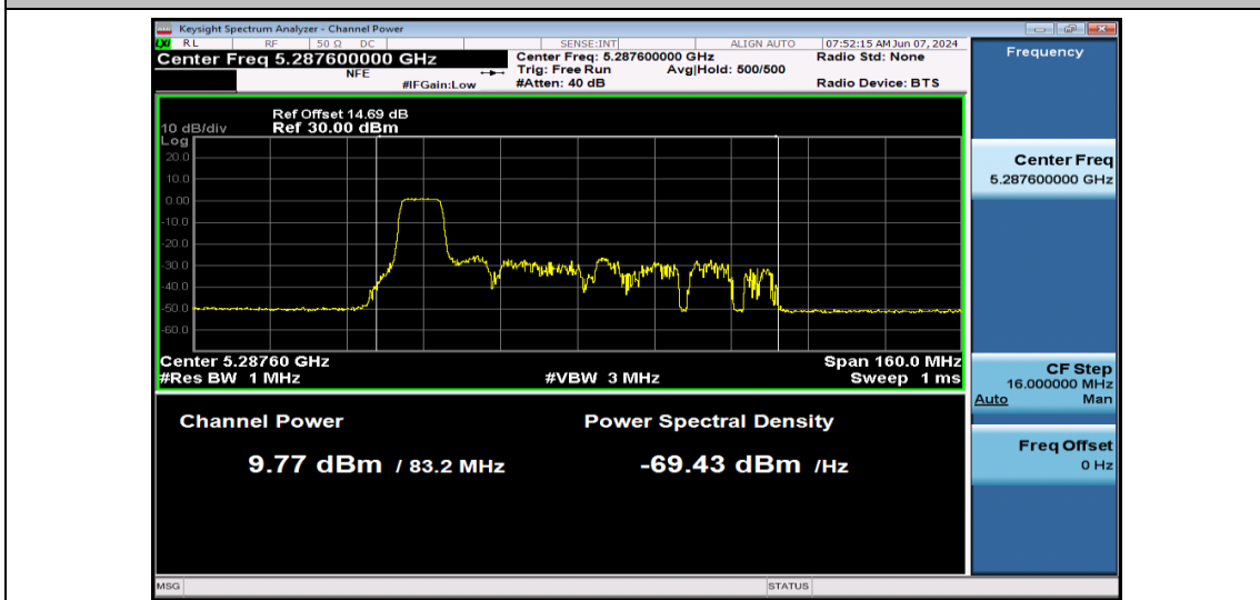
11AX80SISO-Ant1-5290-106Tone-PASS
