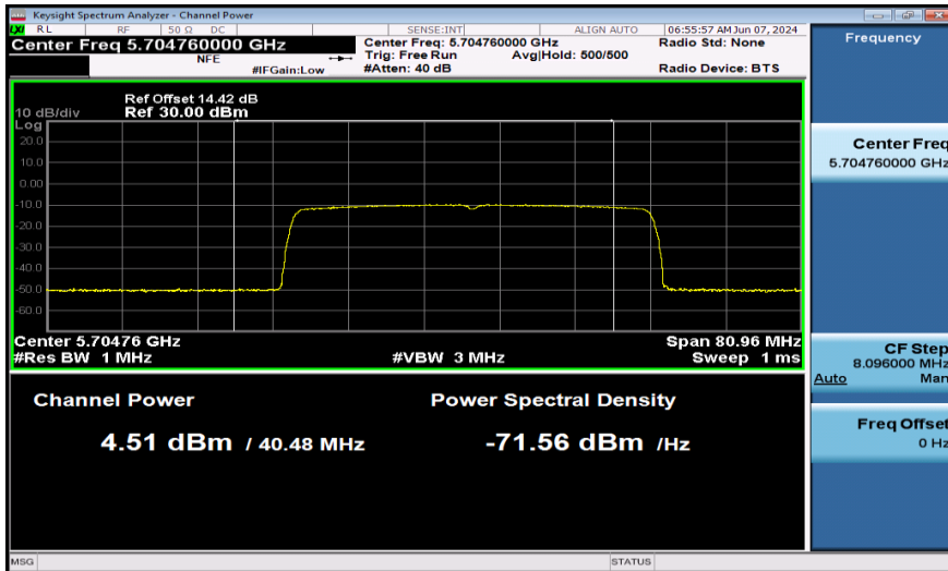
11AX40SISO-Ant1-5710_UNII-2C-484Tone-PASS
