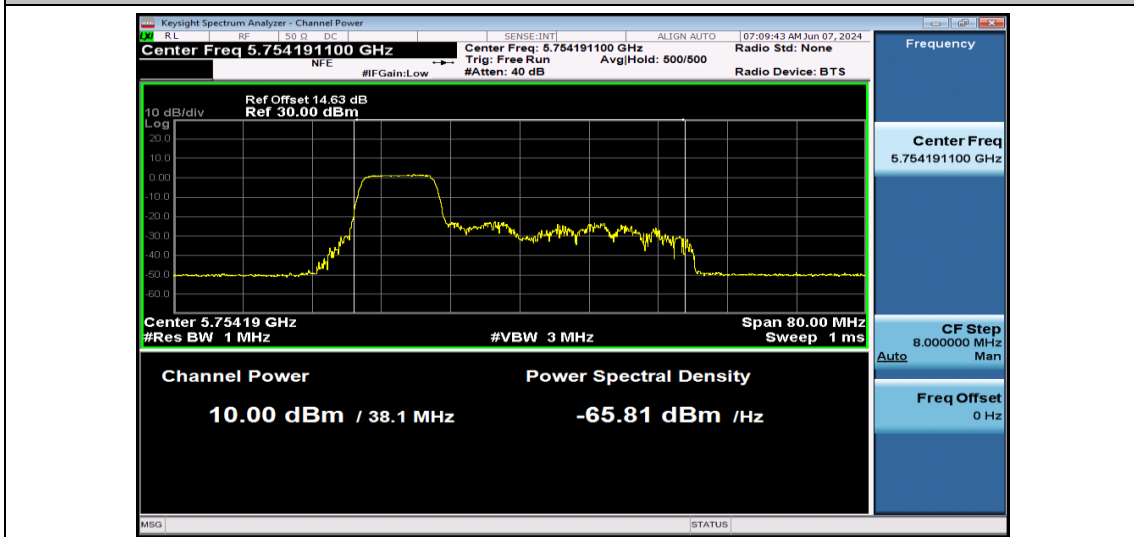
11AX40SISO-Ant1-5755-106Tone-PASS
