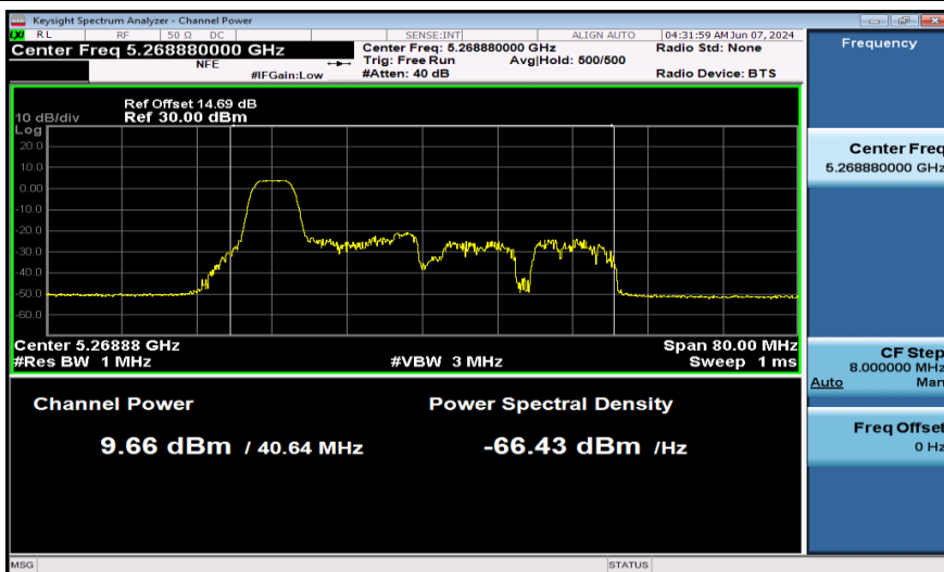
11AX40SISO-Ant1-5270-52Tone-PASS
