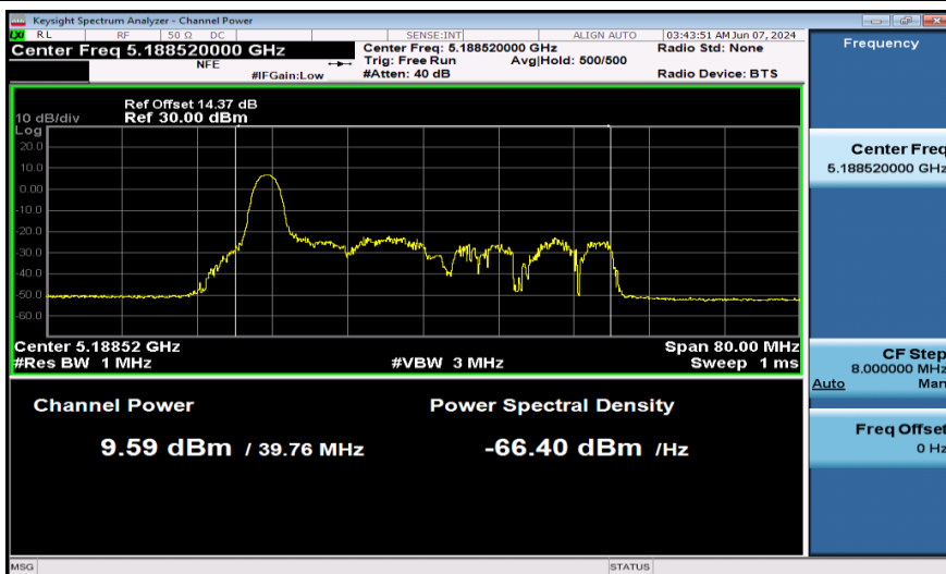
11AX40SISO-Ant1-5190-26Tone-PASS
