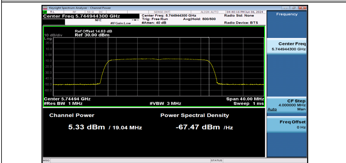
11AX20SISO-Ant1-5745-242Tone-PASS
