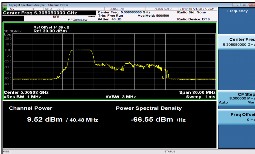
11AX40SISO-Ant1-5310-106Tone-PASS
