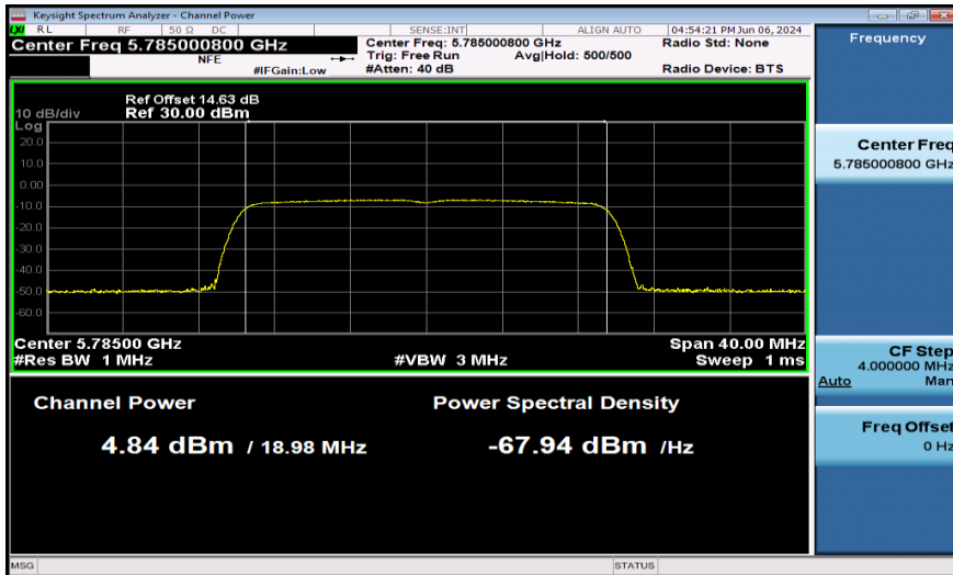
11AX20SISO-Ant1-5785-242Tone-PASS
