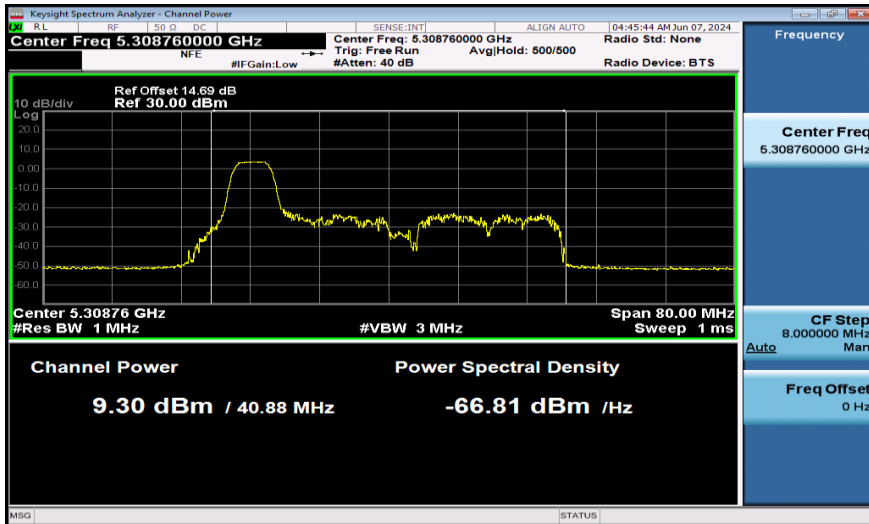
11AX40SISO-Ant1-5310-52Tone-PASS
