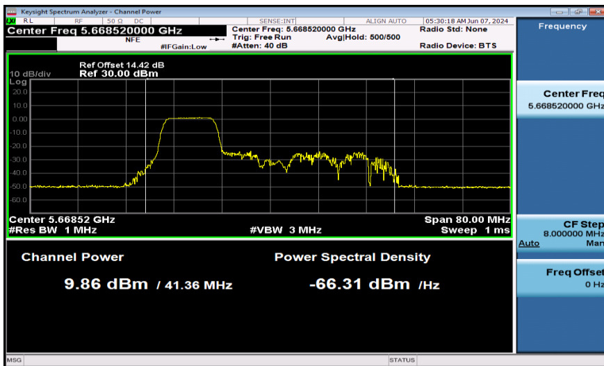
11AX40SISO-Ant1-5670-106Tone-PASS
