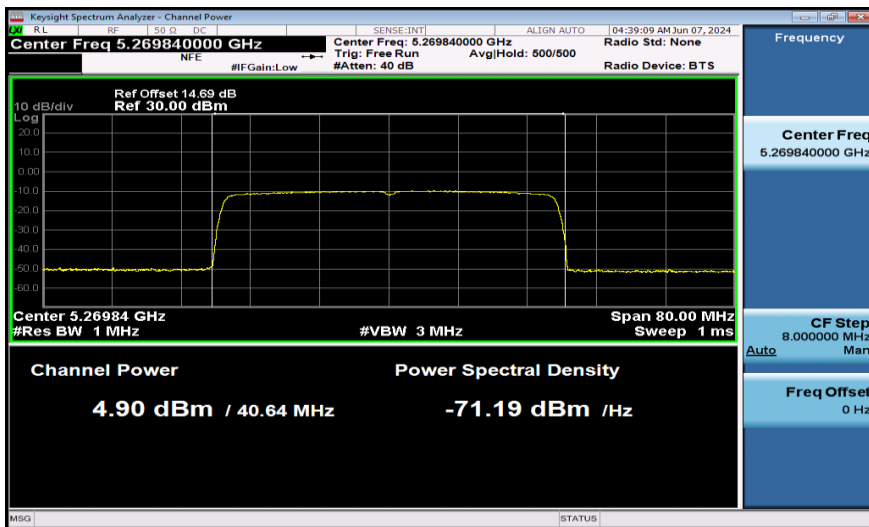
11AX40SISO-Ant1-5270-484Tone-PASS
