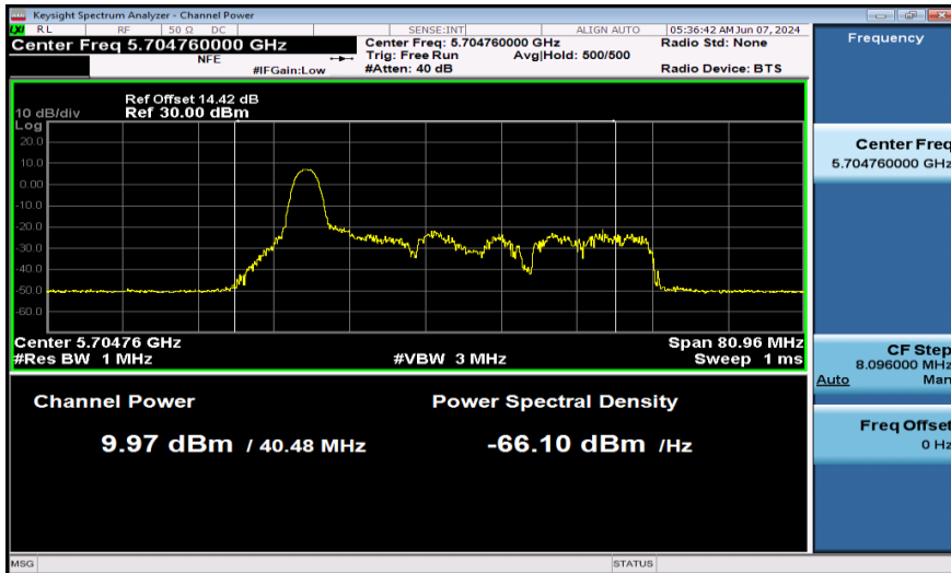
11AX40SISO-Ant1-5710_UNII-2C-26Tone-PASS
