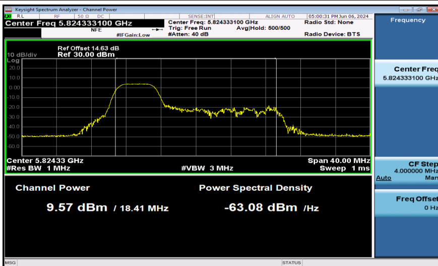
11AX20SISO-Ant1-5825-52Tone-PASS
