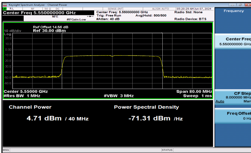
11AX40SISO-Ant1-5550-484Tone-PASS
