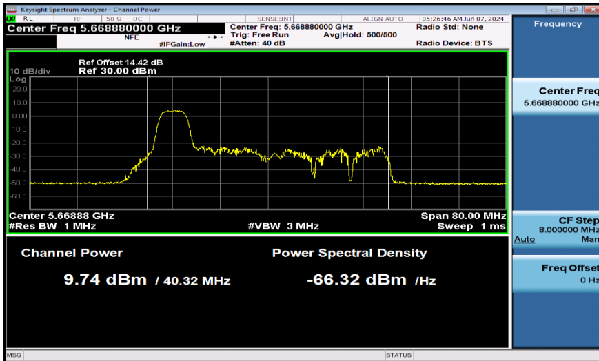
11AX40SISO-Ant1-5670-52Tone-PASS
