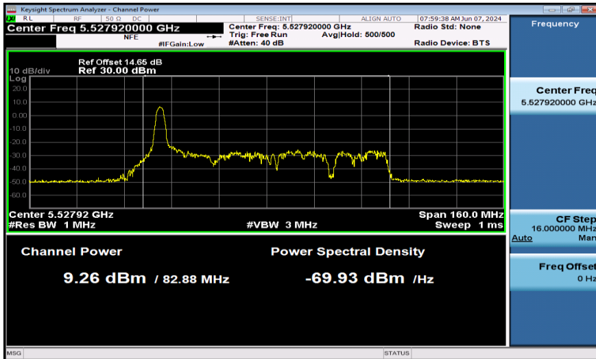
11AX80SISO-Ant1-5530-26Tone-PASS
