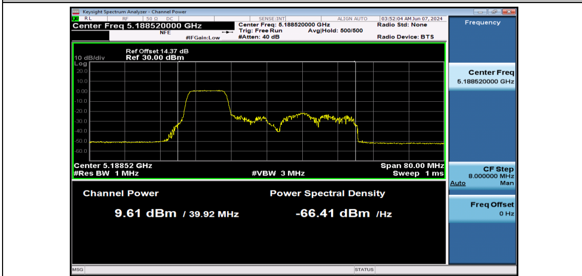
11AX40SISO-Ant1-5190-106Tone-PASS
