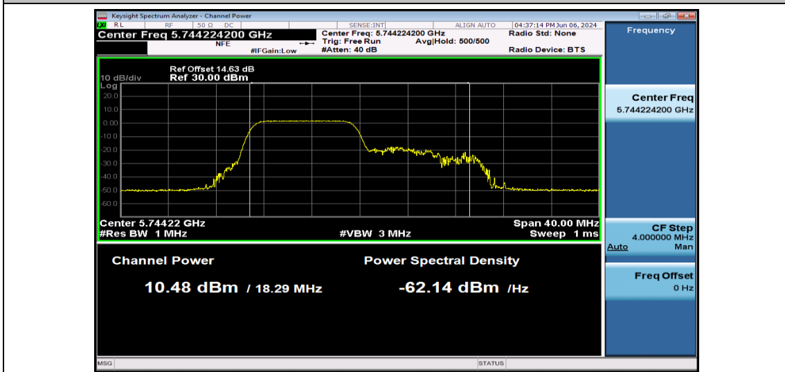
11AX20SISO-Ant1-5745-106Tone-PASS
