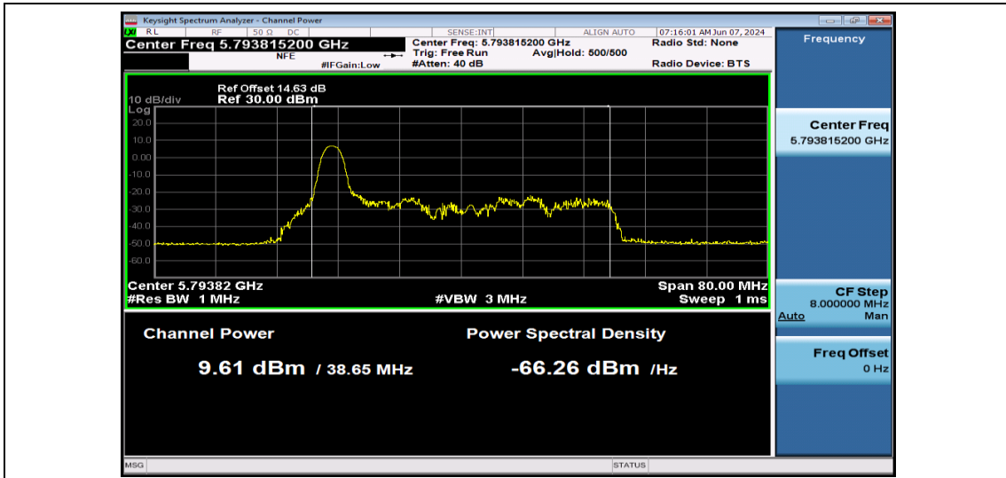
11AX40SISO-Ant1-5795-26Tone-PASS
