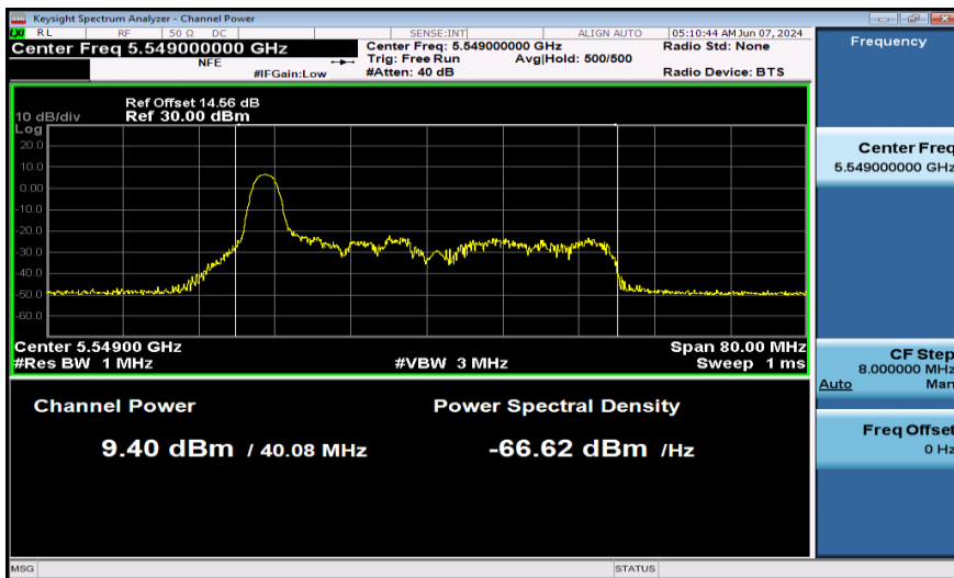
11AX40SISO-Ant1-5550-26Tone-PASS
