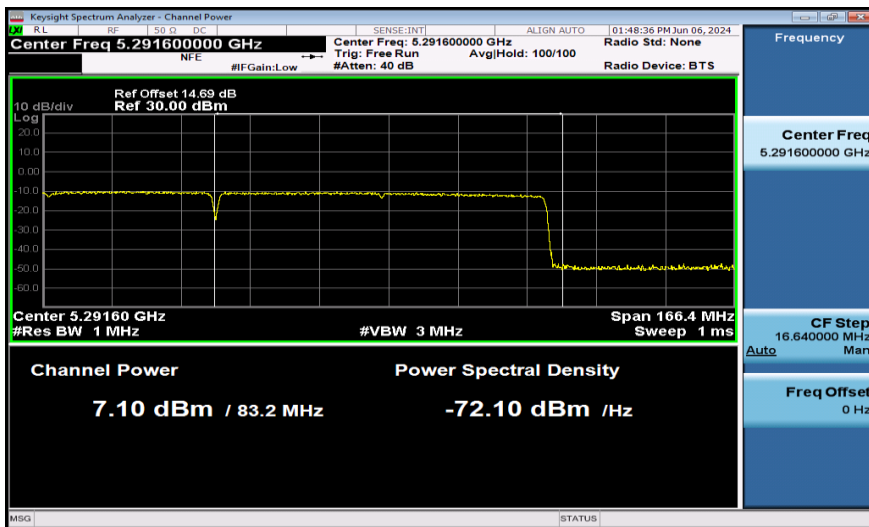
11AX160SISO-Ant1-5250_UNII-2A-PASS
