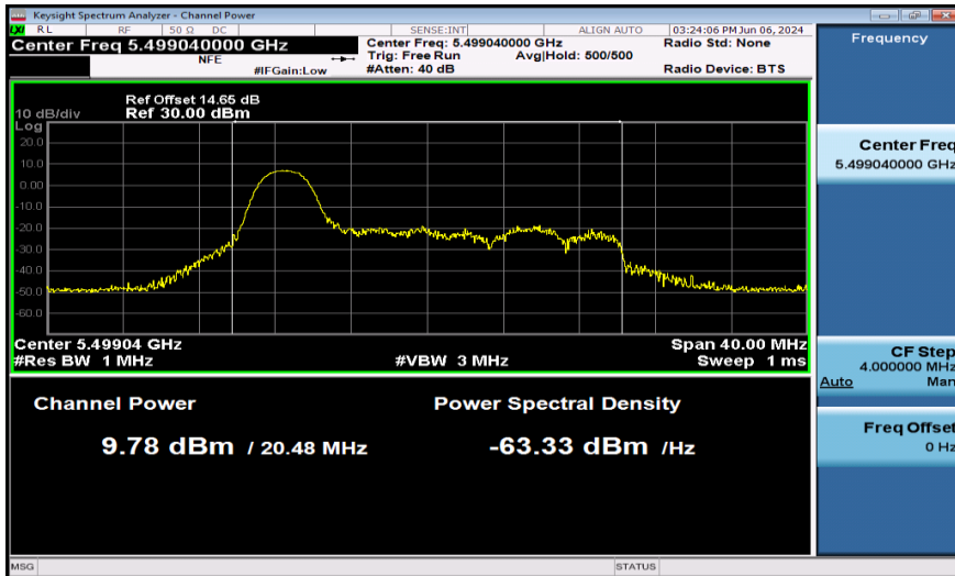
11AX20SISO-Ant1-5500-26Tone-PASS
