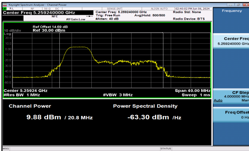
11AX20SISO-Ant1-5260-52Tone-PASS
