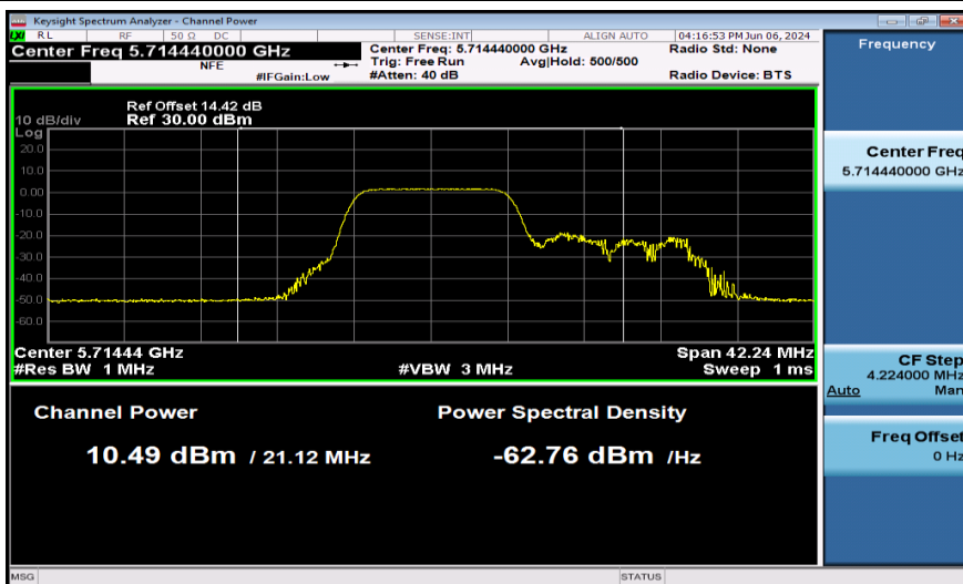
11AX20SISO-Ant1-5720_UNII-2C-106Tone-PASS
