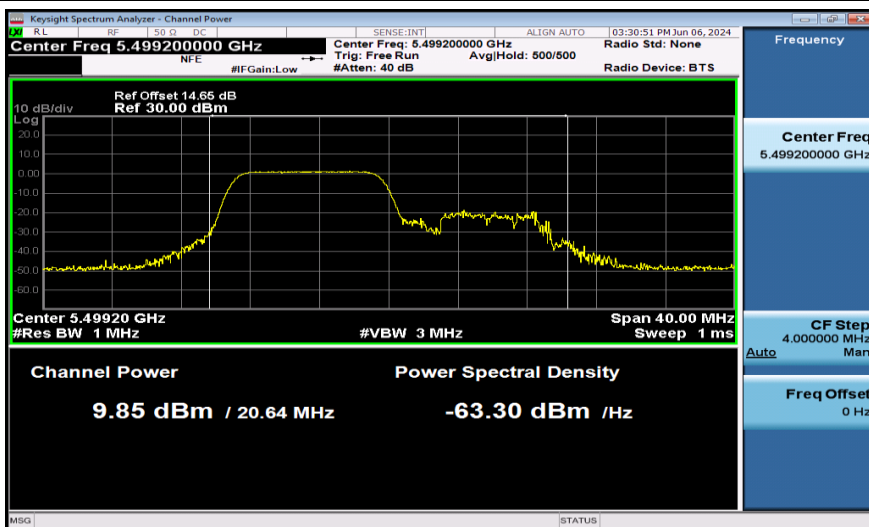
11AX20SISO-Ant1-5500-106Tone-PASS
