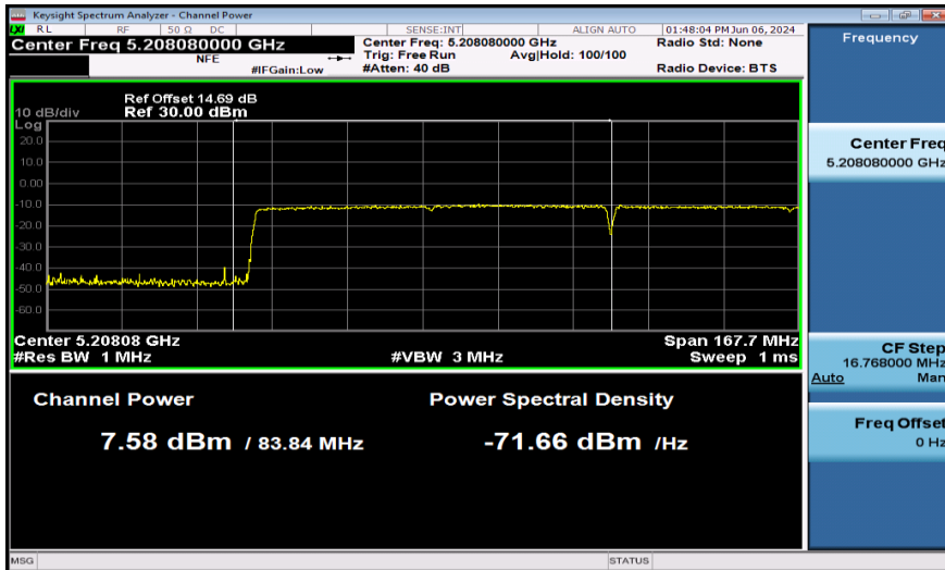
11AX160SISO-Ant1-5250_UNII-1-PASS
