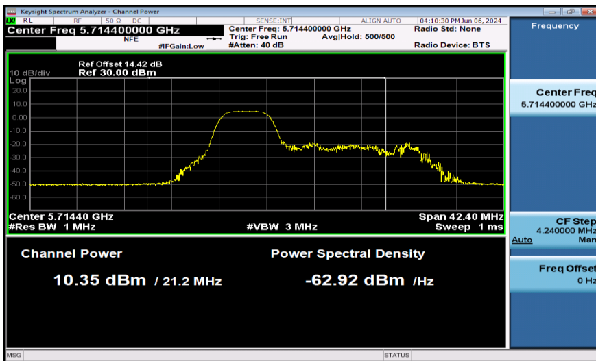
11AX20SISO-Ant1-5720_UNII-2C-52Tone-PASS
