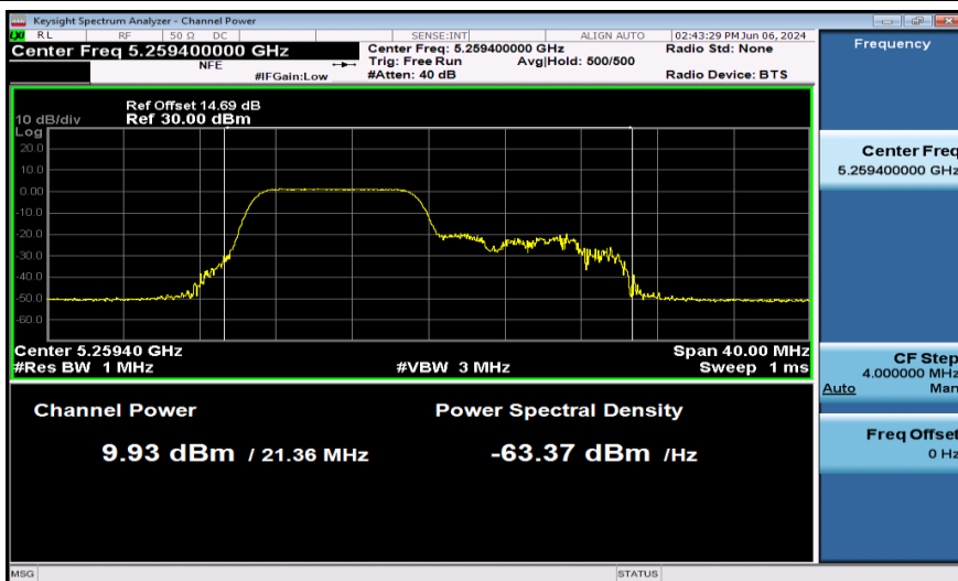
11AX20SISO-Ant1-5260-106Tone-PASS
