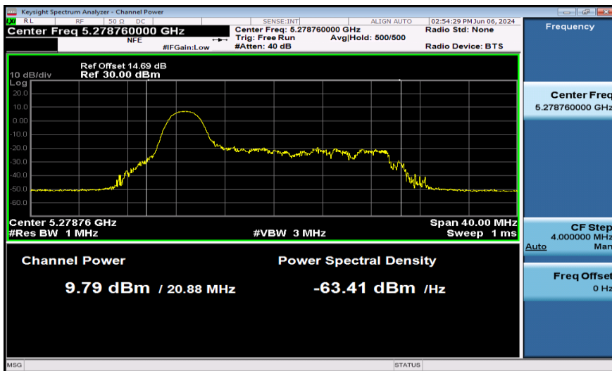
11AX20SISO-Ant1-5280-26Tone-PASS
