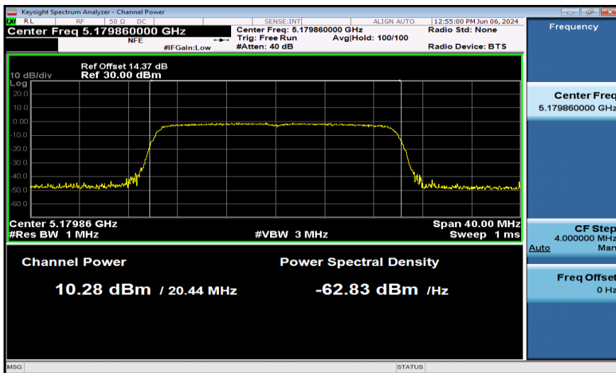
11AX20SISO-Ant1-5180-PASS
