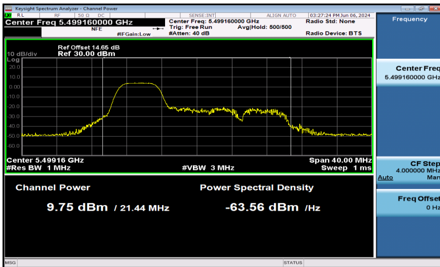
11AX20SISO-Ant1-5500-52Tone-PASS
