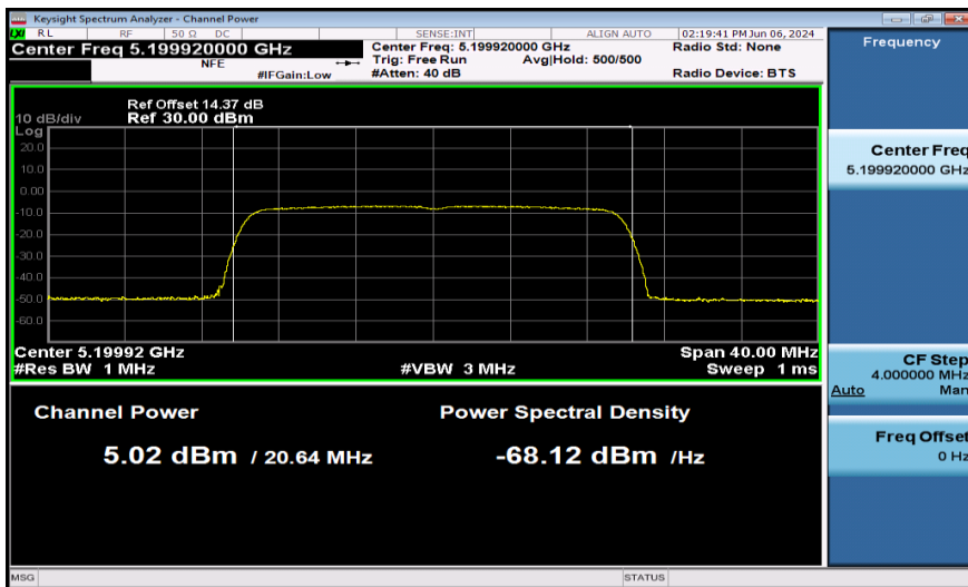
11AX20SISO-Ant1-5200-242Tone-PASS
