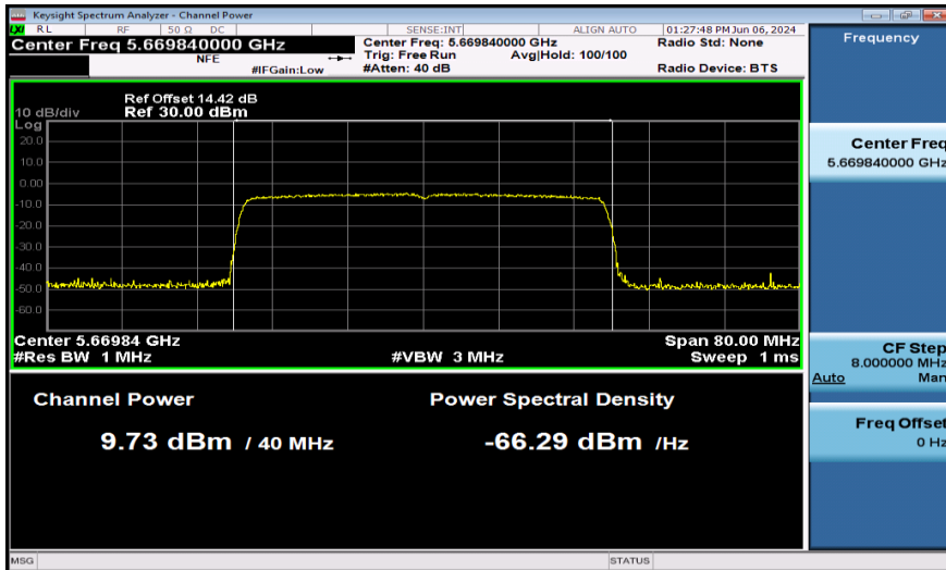
11AX40SISO-Ant1-5670-PASS
