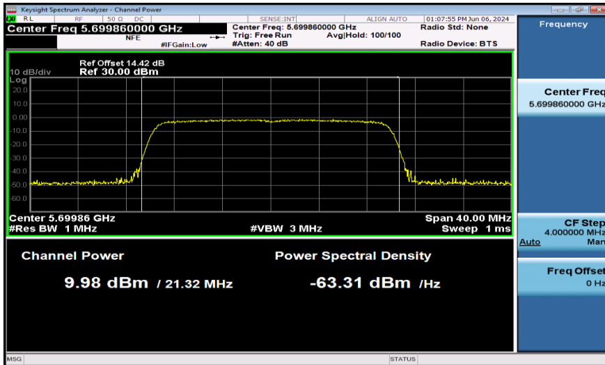
11AX20SISO-Ant1-5700-PASS
