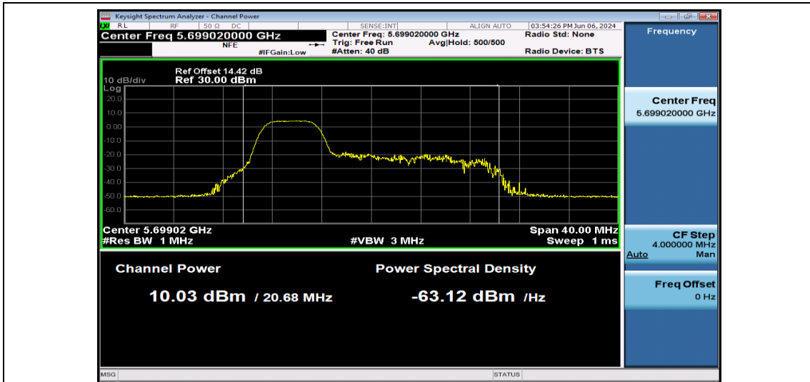
11AX20SISO-Ant1-5700-52Tone-PASS
