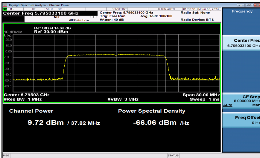
11AX40SISO-Ant1-5795-PASS
