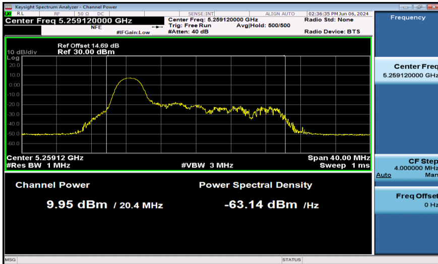
11AX20SISO-Ant1-5260-26Tone-PASS
