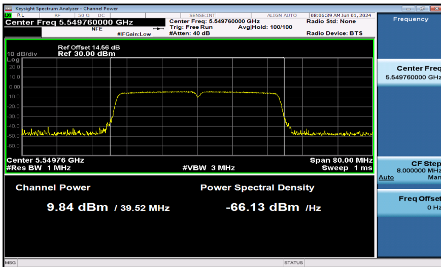
11AC40SISO-Ant1-5550-PASS
