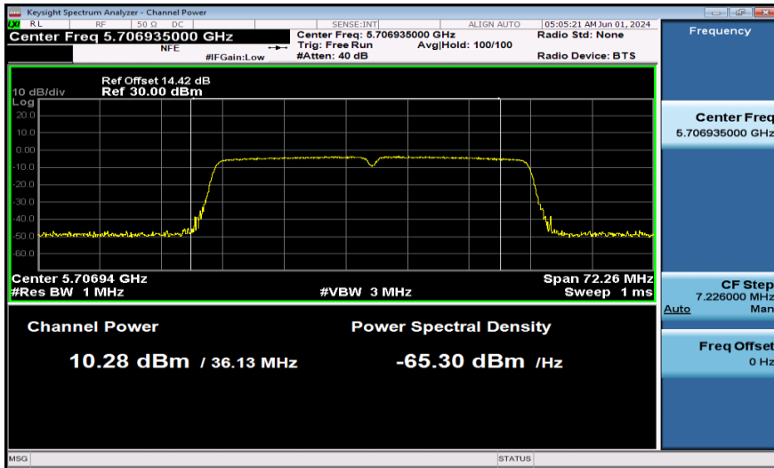
11AC40SISO-Ant1-5710_UNII-2C-PASS
