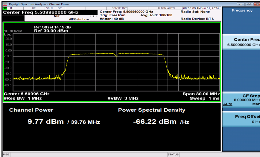
11AC40SISO-Ant1-5510-PASS
