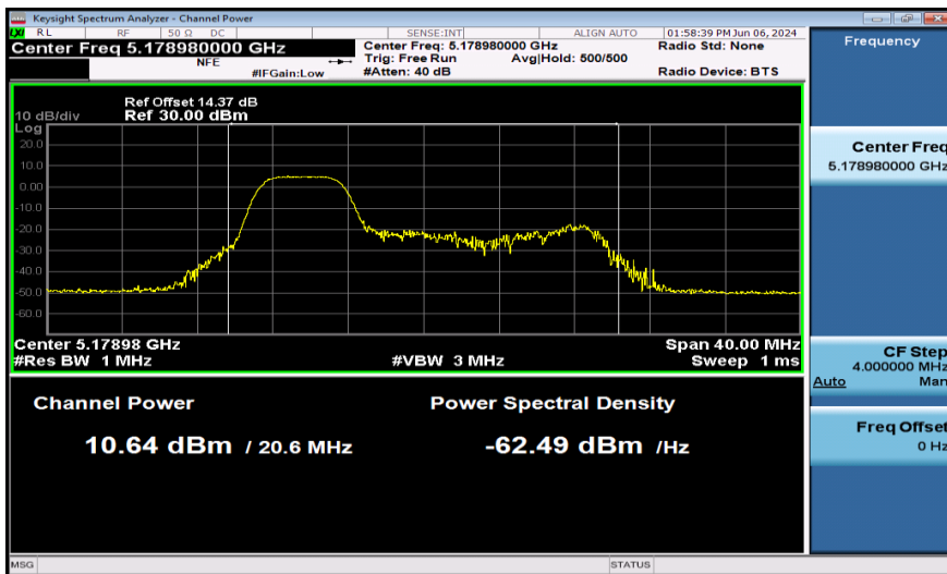
11AX20SISO-Ant1-5180-52Tone-PASS
