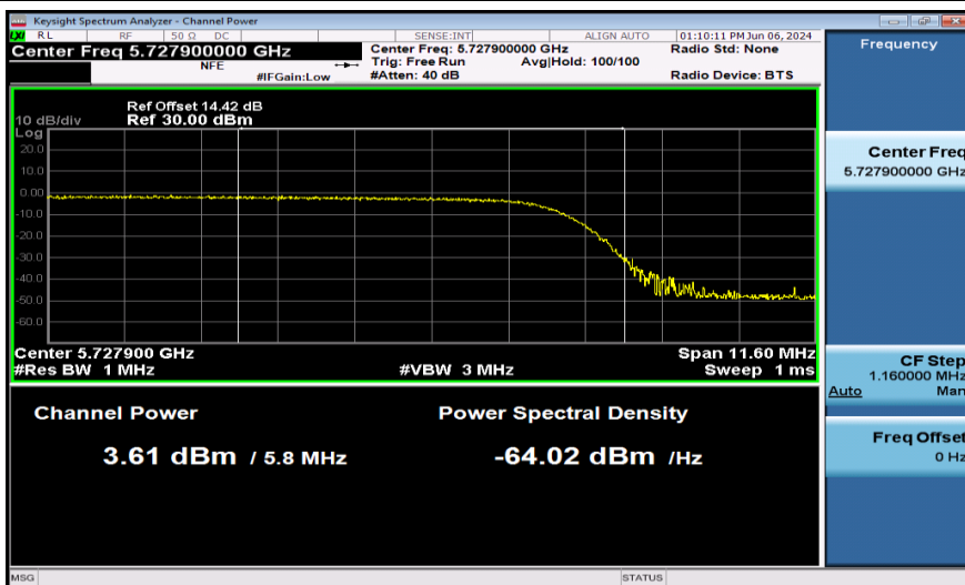
11AX20SISO-Ant1-5720_UNII-3-PASS
