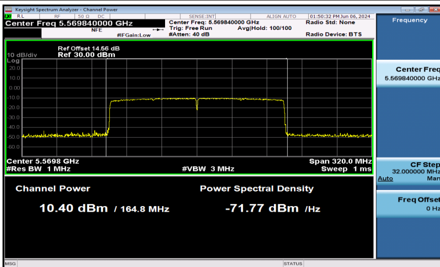
11AX160SISO-Ant1-5570-PASS
