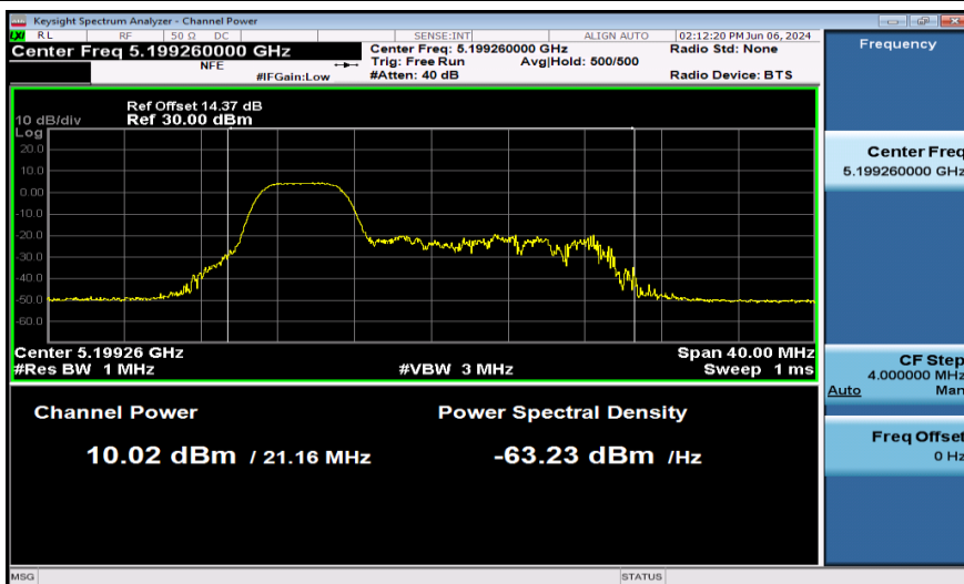
11AX20SISO-Ant1-5200-52Tone-PASS
