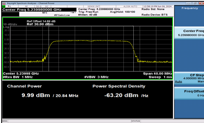
11AX20SISO-Ant1-5240-PASS
