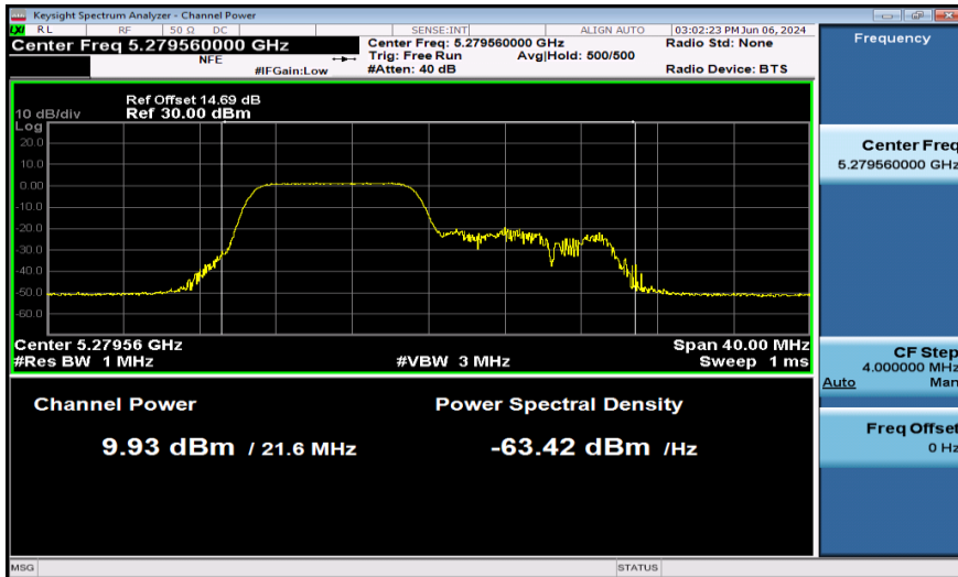
11AX20SISO-Ant1-5280-106Tone-PASS
