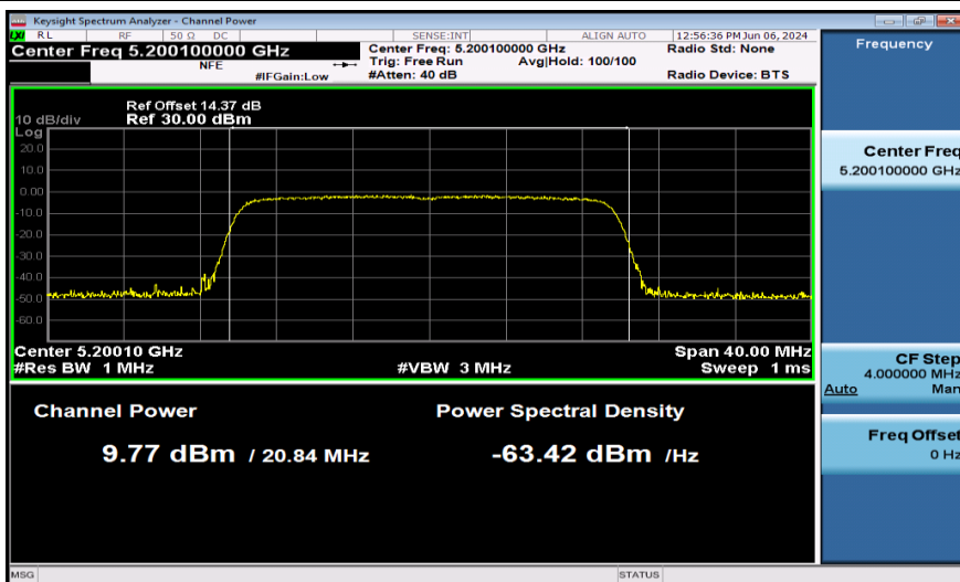
11AX20SISO-Ant1-5200-PASS
