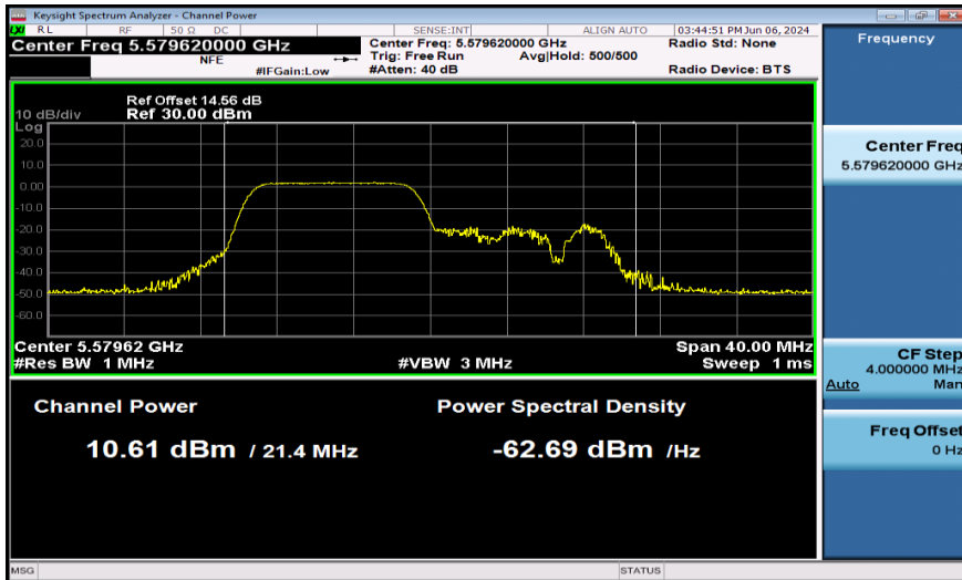
11AX20SISO-Ant1-5580-106Tone-PASS
