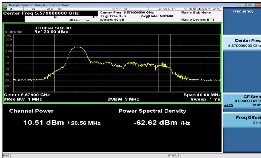
11AX20SISO-Ant1-5580-26Tone-PASS
