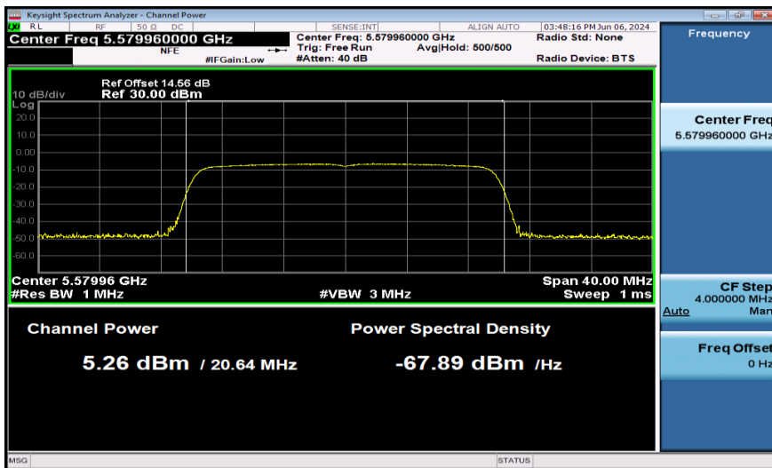
11AX20SISO-Ant1-5580-242Tone-PASS
