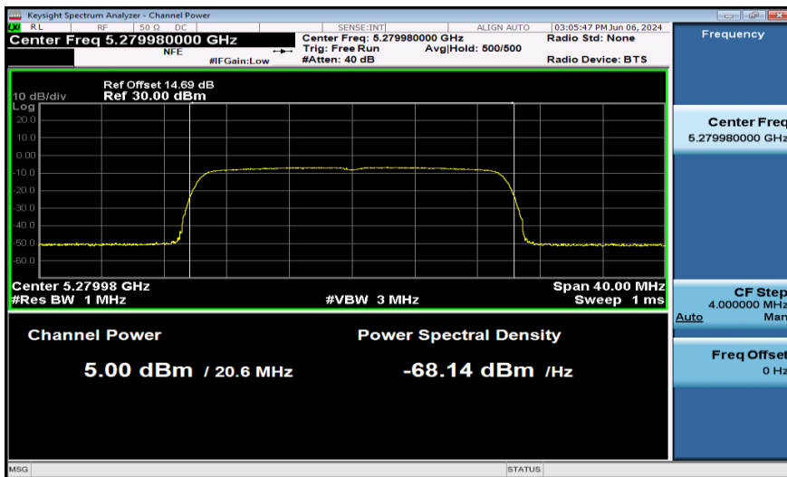
11AX20SISO-Ant1-5280-242Tone-PASS
