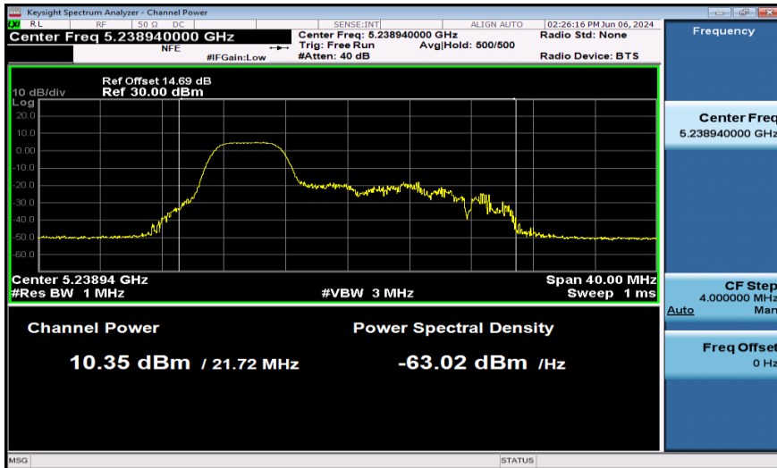
11AX20SISO-Ant1-5240-52Tone-PASS
