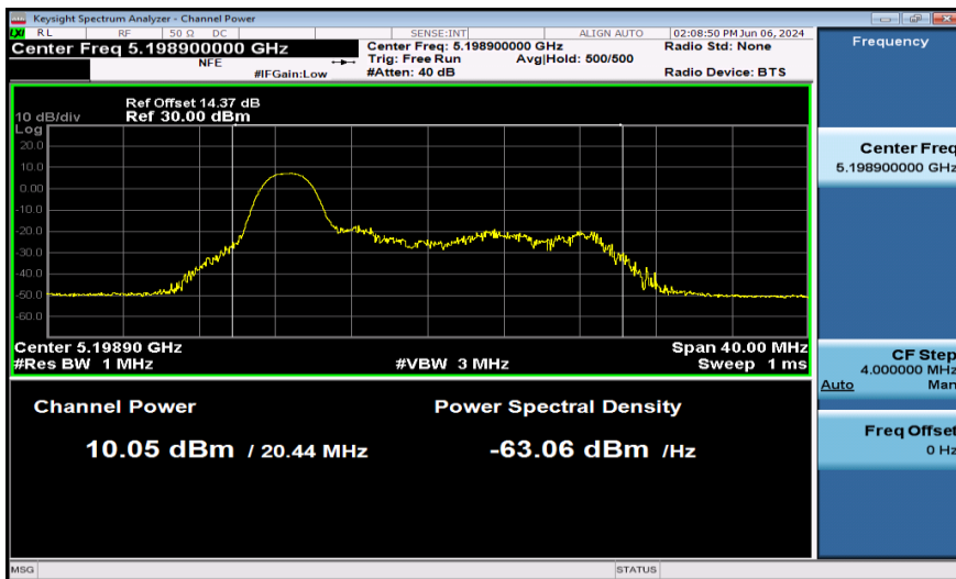
11AX20SISO-Ant1-5200-26Tone-PASS
