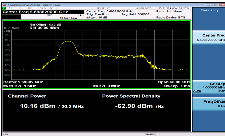
11AX20SISO-Ant1-5700-26Tone-PASS
