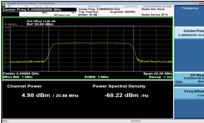
11AX20SISO-Ant1-5500-242Tone-PASS
