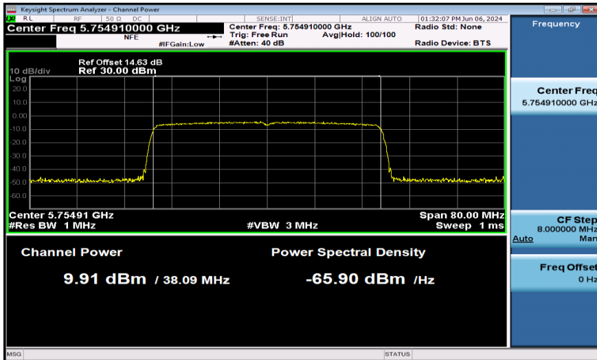
11AX40SISO-Ant1-5755-PASS
