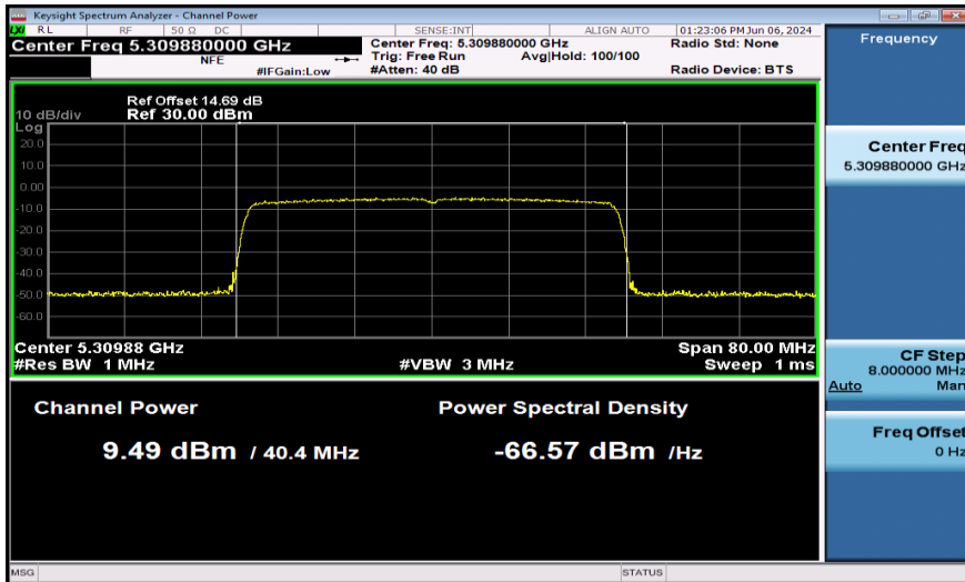
11AX40SISO-Ant1-5310-PASS
