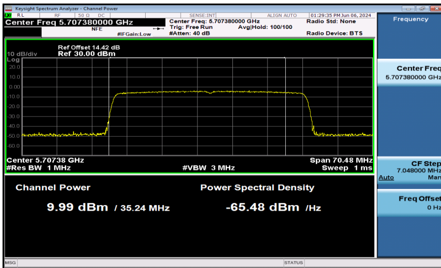
11AX40SISO-Ant1-5710_UNII-2C-PASS
