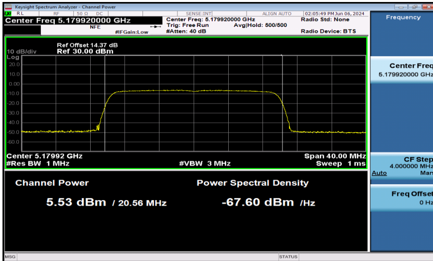
11AX20SISO-Ant1-5180-242Tone-PASS
