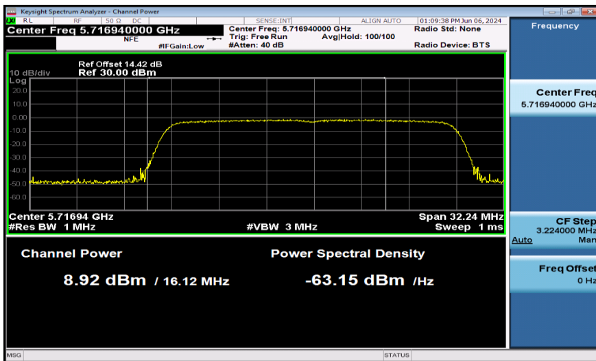
11AX20SISO-Ant1-5720_UNII-2C-PASS
