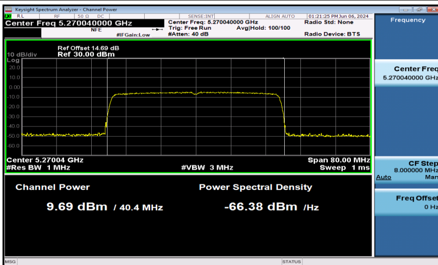
11AX40SISO-Ant1-5270-PASS
