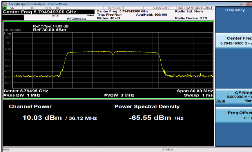
11AC40SISO-Ant1-5795-PASS
