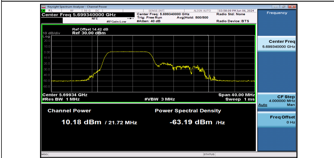
11AX20SISO-Ant1-5700-106Tone-PASS
