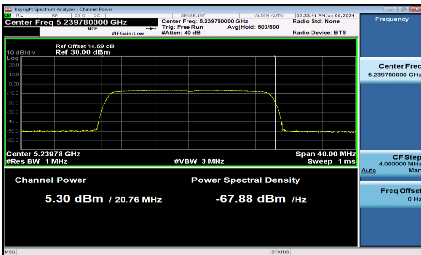
11AX20SISO-Ant1-5240-242Tone-PASS
