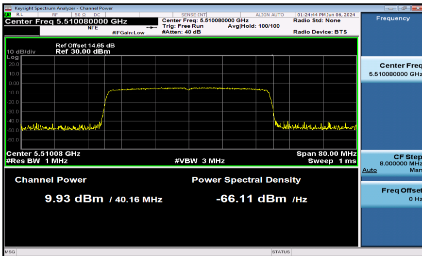
11AX40SISO-Ant1-5510-PASS
