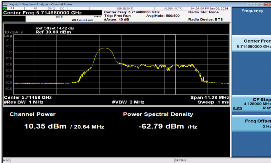
11AX20SISO-Ant1-5720_UNII-2C-26Tone-PASS
