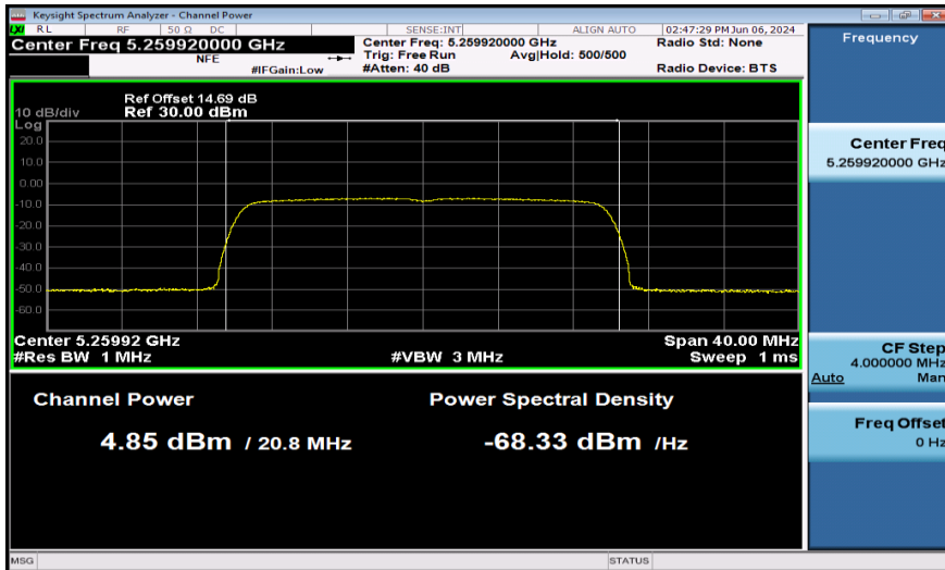
11AX20SISO-Ant1-5260-242Tone-PASS
