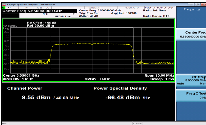
11AX40SISO-Ant1-5550-PASS
