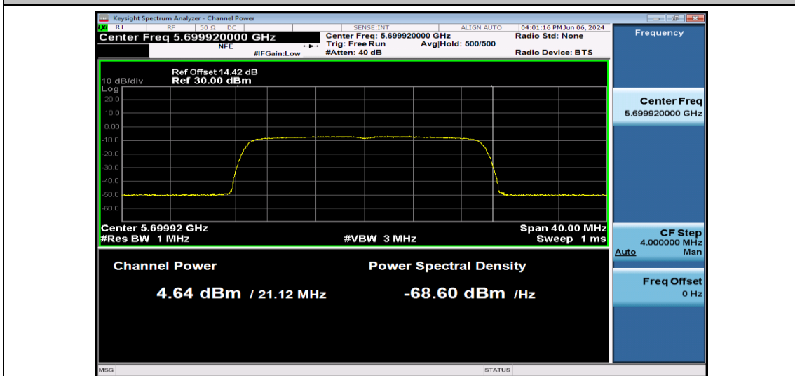
11AX20SISO-Ant1-5700-242Tone-PASS
