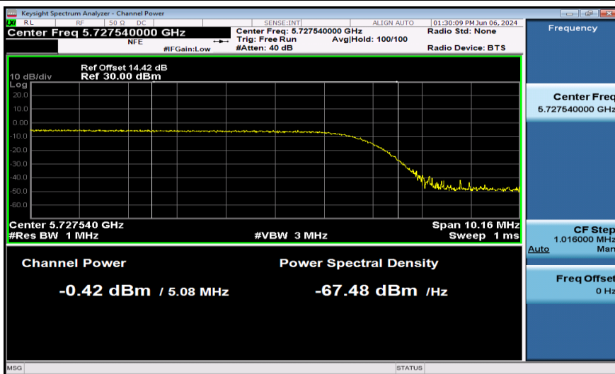
11AX40SISO-Ant1-5710_UNII-3-PASS
