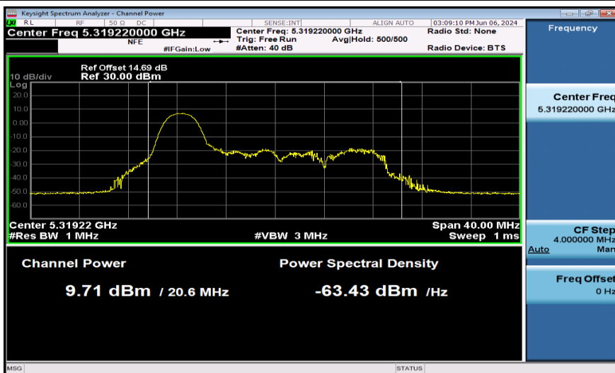
11AX20SISO-Ant1-5320-26Tone-PASS
