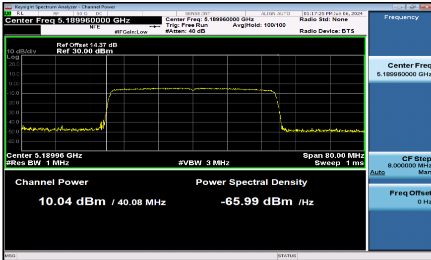
11AX40SISO-Ant1-5190-PASS
