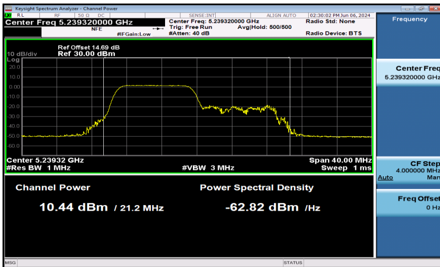
11AX20SISO-Ant1-5240-106Tone-PASS
