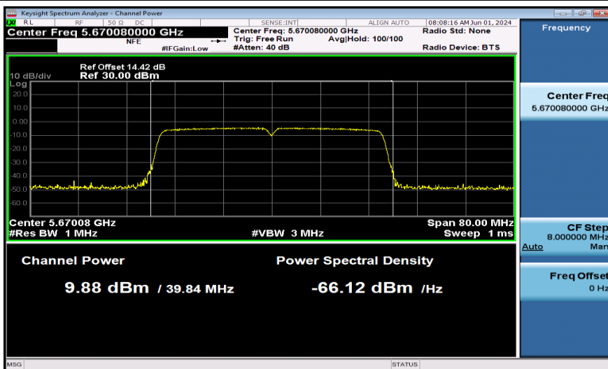
11AC40SISO-Ant1-5670-PASS
