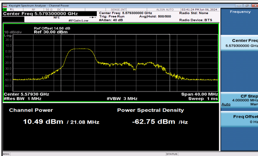
11AX20SISO-Ant1-5580-52Tone-PASS
