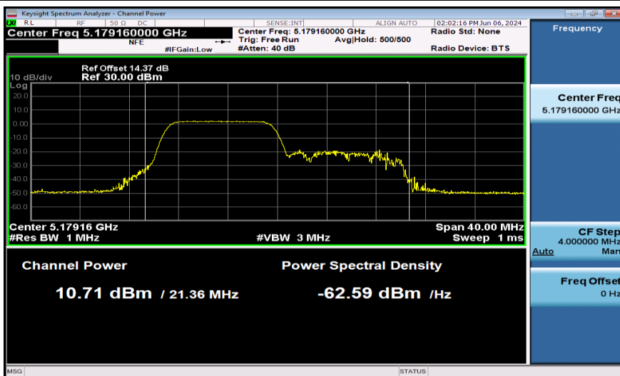
11AX20SISO-Ant1-5180-106Tone-PASS
