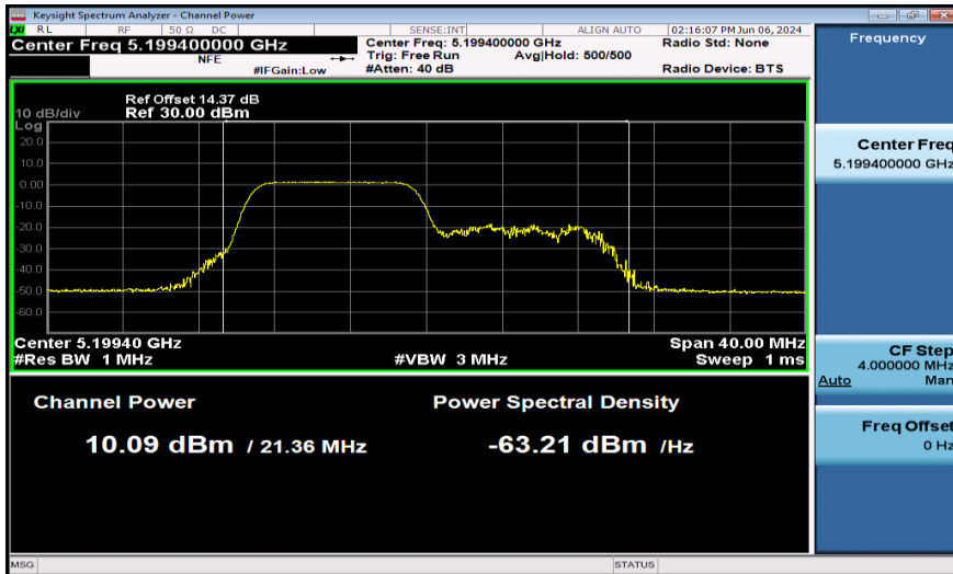
11AX20SISO-Ant1-5200-106Tone-PASS
