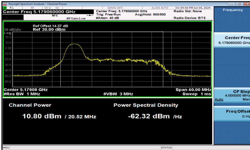
11AX20SISO-Ant1-5180-26Tone-PASS
