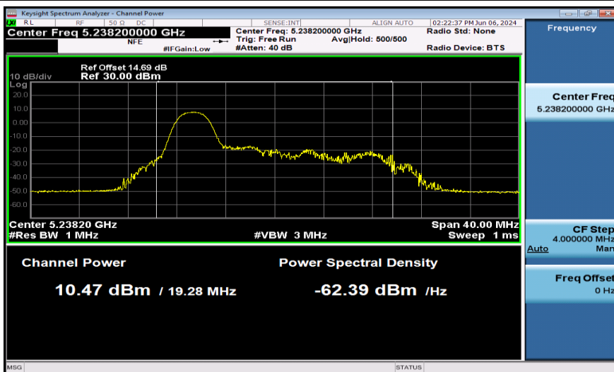
11AX20SISO-Ant1-5240-26Tone-PASS
