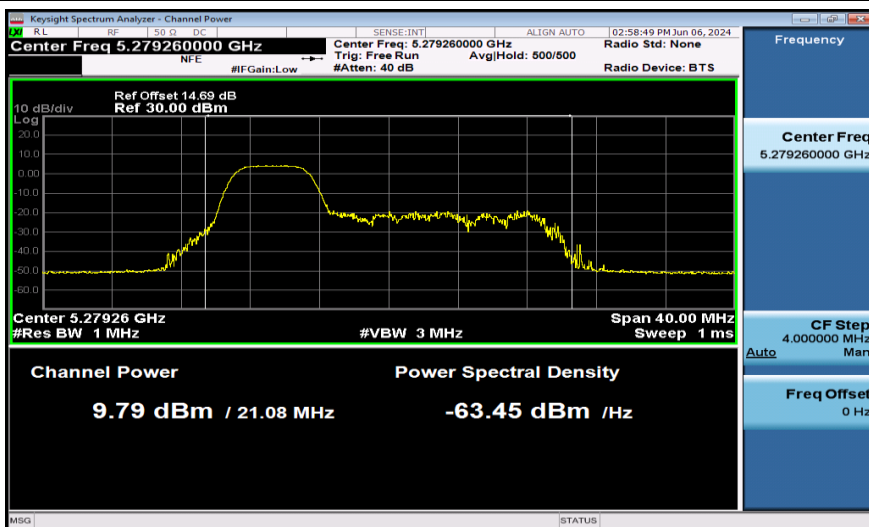
11AX20SISO-Ant1-5280-52Tone-PASS
