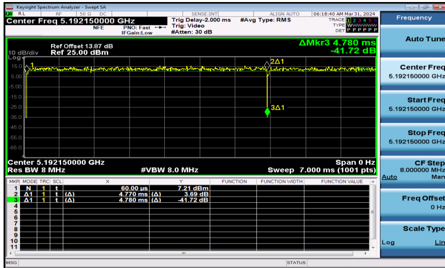
NTNV-11AX20SISO-Ant1-5200-106Tone
