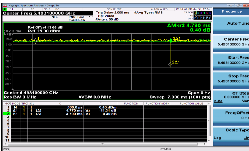
NTNV-11AX20SISO-Ant1-5500-106Tone
