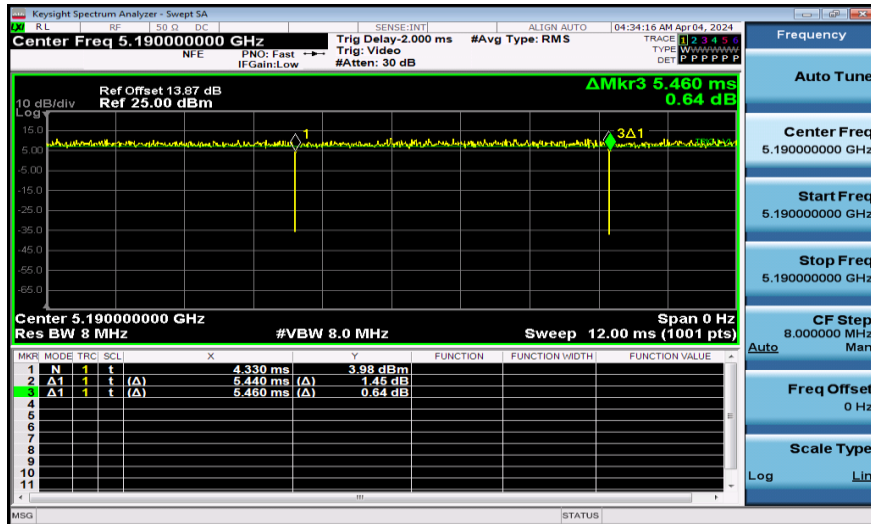
NTNV-11AX40SISO-Ant1-5190
