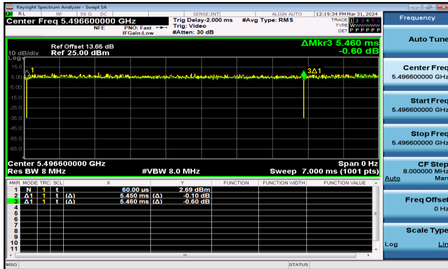
NTNV-11AX20SISO-Ant1-5500-242Tone
