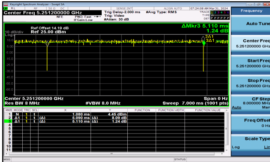
NTNV-11AX20SISO-Ant1-5260-26Tone
