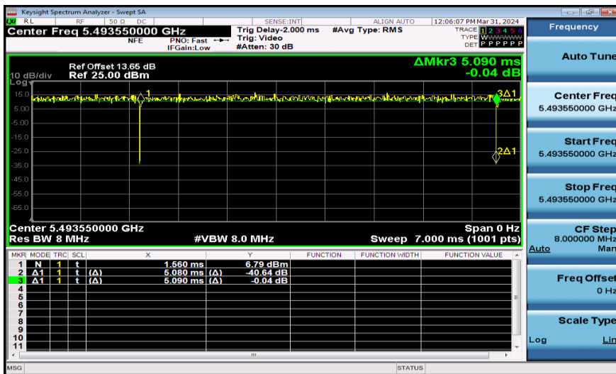
NTNV-11AX20SISO-Ant1-5500-52Tone
