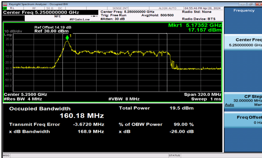
11AX160SISO-Ant1-5250-52Tone
