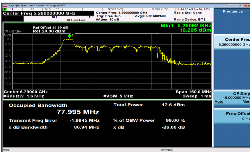
11AX80SISO-Ant1-5290-106Tone
