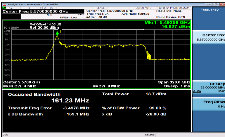
11AX160SISO-Ant1-5570-52Tone
