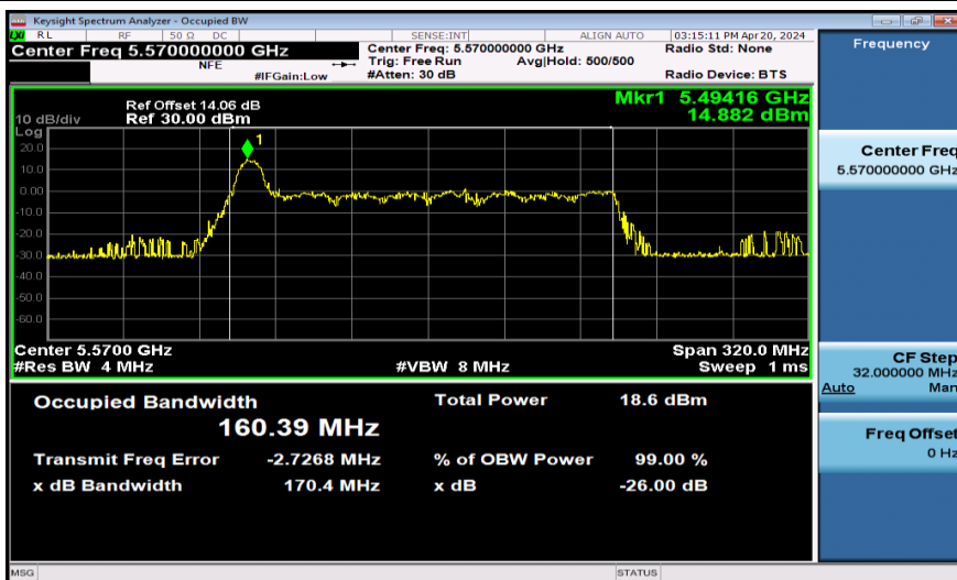
11AX160SISO-Ant1-5570-106Tone
