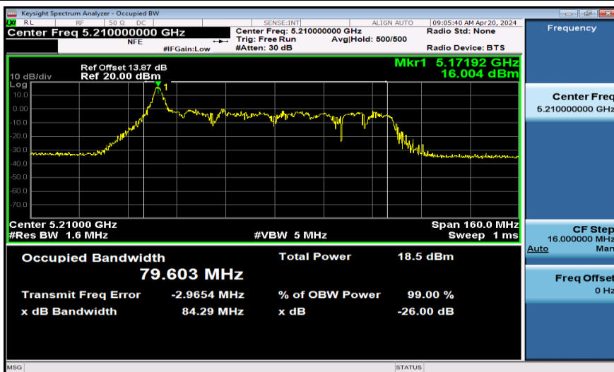
11AX80SISO-Ant1-5210-26Tone
