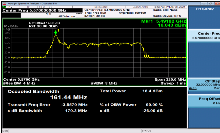
11AX160SISO-Ant1-5570-26Tone
