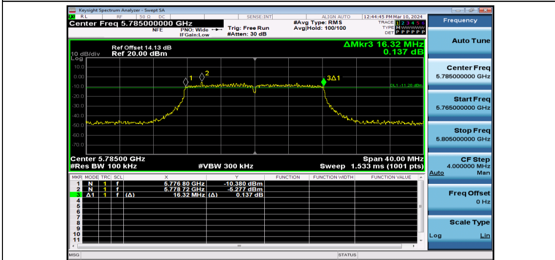
11A-Ant1-5785-PASS
