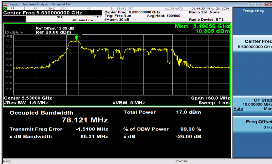
11AX80SISO-Ant1-5530-106Tone
