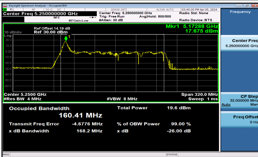
11AX160SISO-Ant1-5250-26Tone
