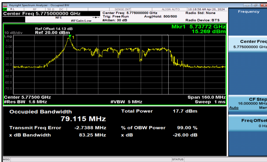
11AX80SISO-Ant1-5775-26Tone
