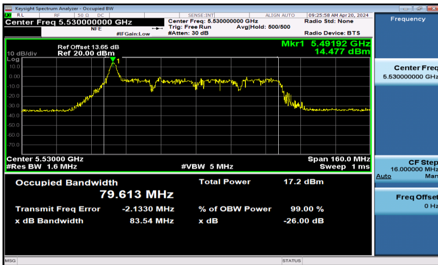
11AX80SISO-Ant1-5530-26Tone
