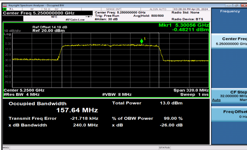
11AX160SISO-Ant1-5250-2*996Tone
