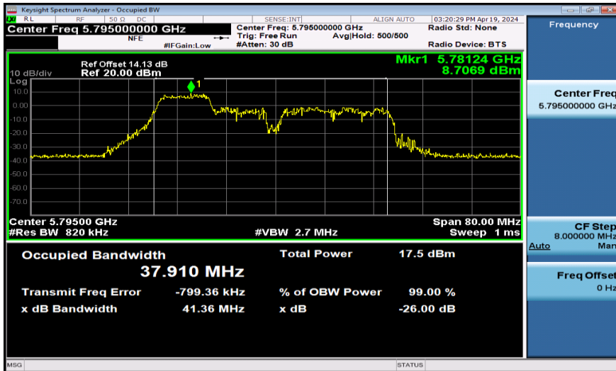
11AX40SISO-Ant1-5795-106Tone
