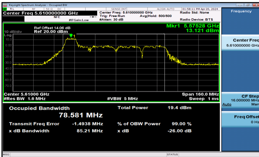
11AX80SISO-Ant1-5610-106Tone
