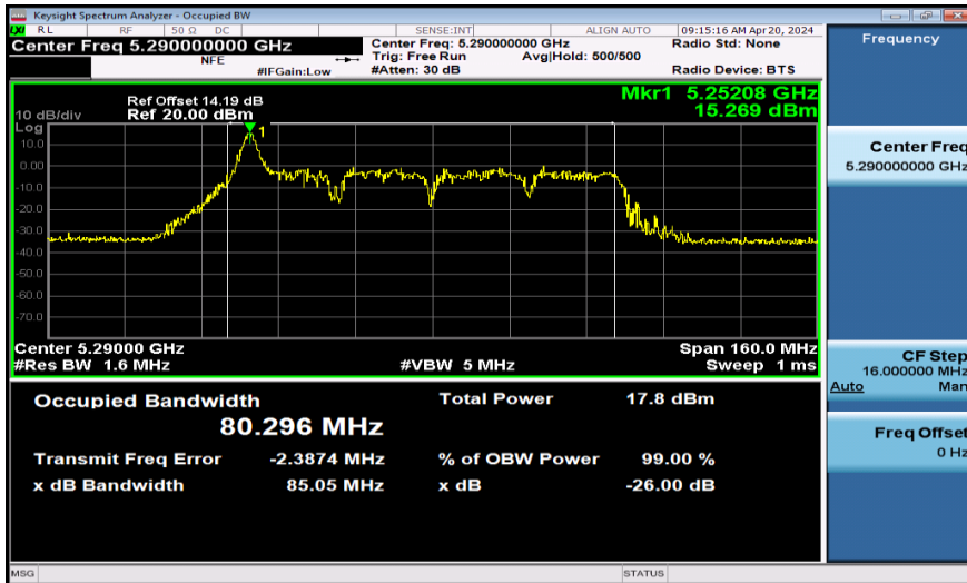
11AX80SISO-Ant1-5290-26Tone
