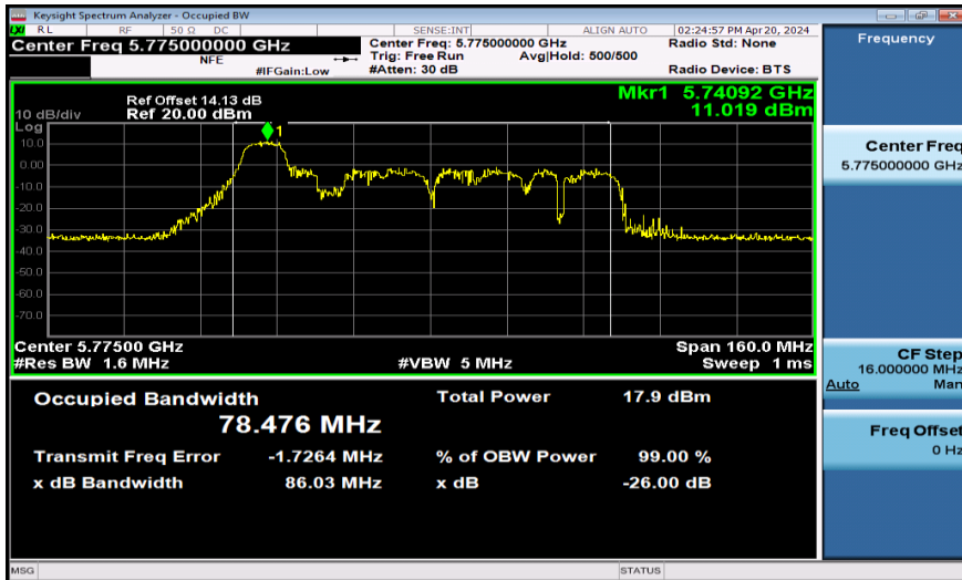
11AX80SISO-Ant1-5775-106Tone
