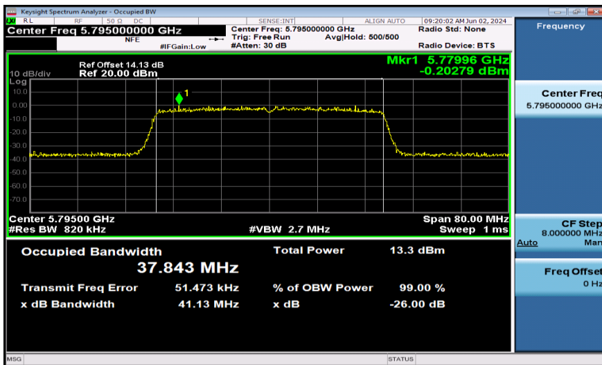
11AX40SISO-Ant1-5795-484Tone
