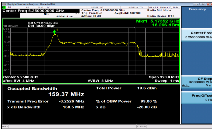
11AX160SISO-Ant1-5250-106Tone
