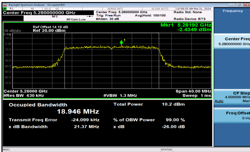
11AX20SISO-Ant1-5280-242Tone
