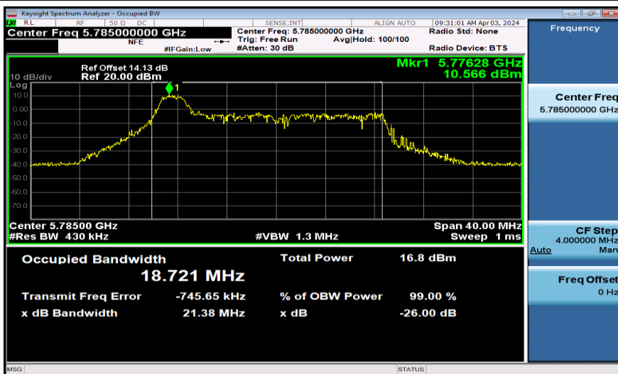
11AX20SISO-Ant1-5785-26Tone
