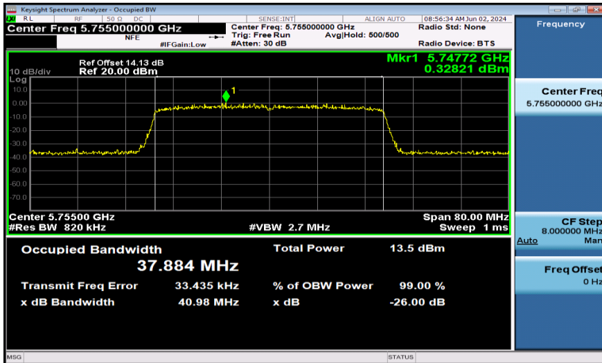
11AX40SISO-Ant1-5755-484Tone
