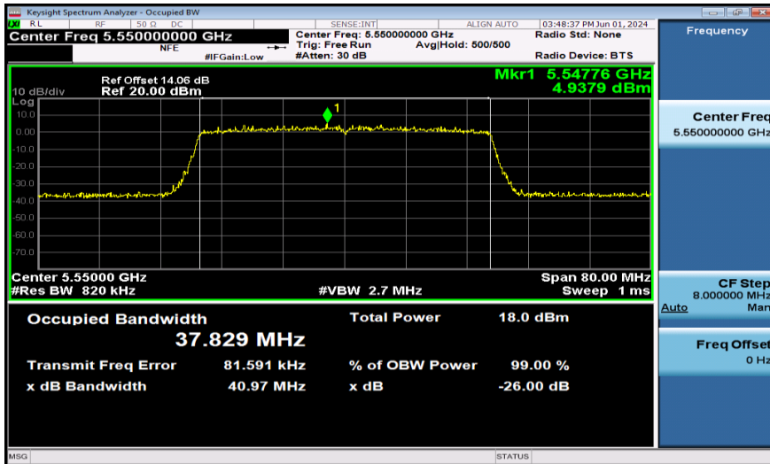
11AX40SISO-Ant1-5550-484Tone
