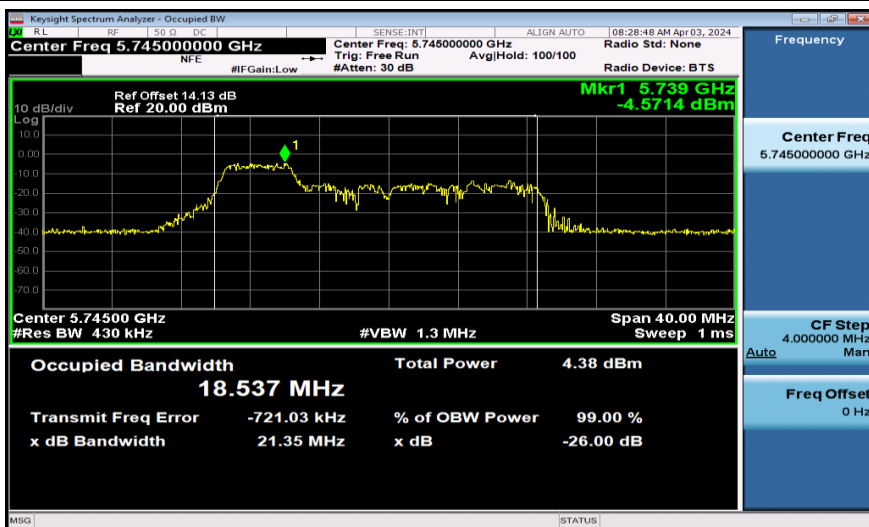
11AX20SISO-Ant1-5745-52Tone
