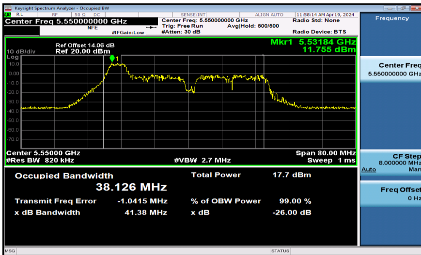
11AX40SISO-Ant1-5550-52Tone
