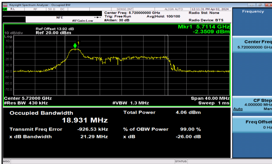
11AX20SISO-Ant1-5720-26Tone
