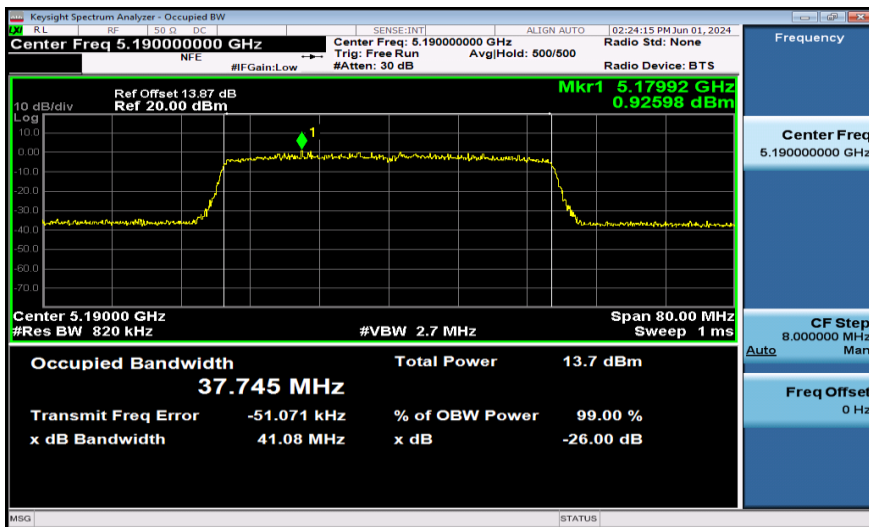
11AX40SISO-Ant1-5190-484Tone-RU61
