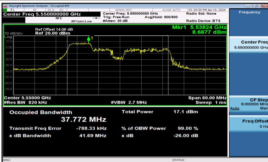
11AX40SISO-Ant1-5550-106Tone
