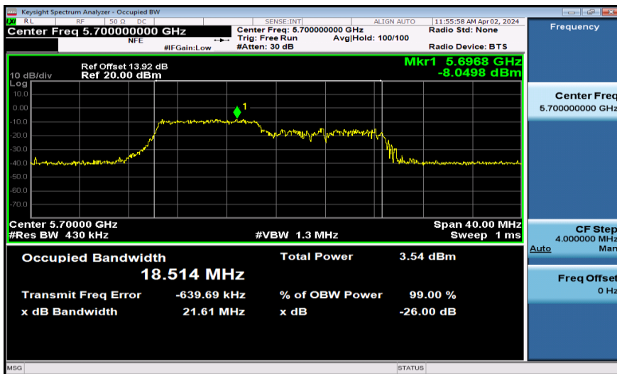
11AX20SISO-Ant1-5700-106Tone
