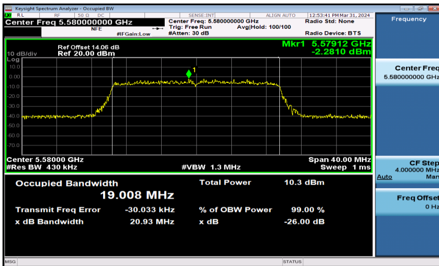
11AX20SISO-Ant1-5580-242Tone
