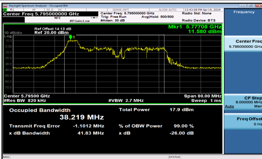
11AX40SISO-Ant1-5795-52Tone
