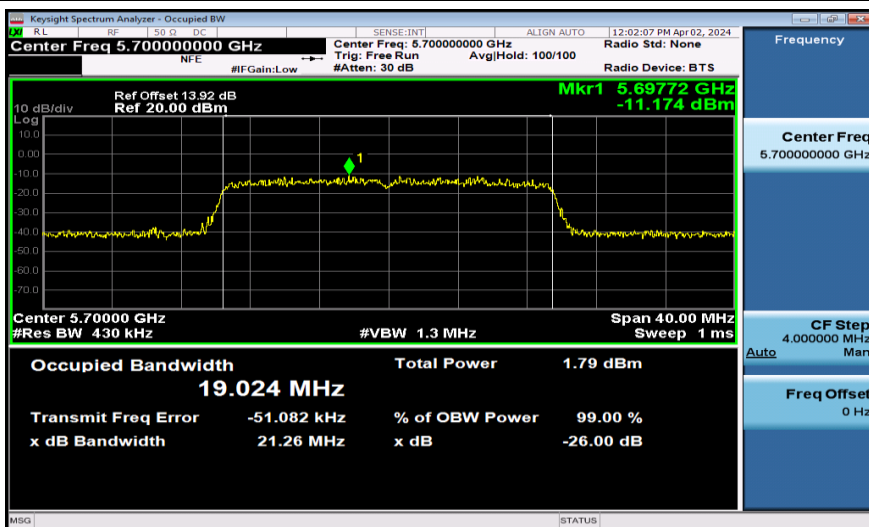
11AX20SISO-Ant1-5700-242Tone
