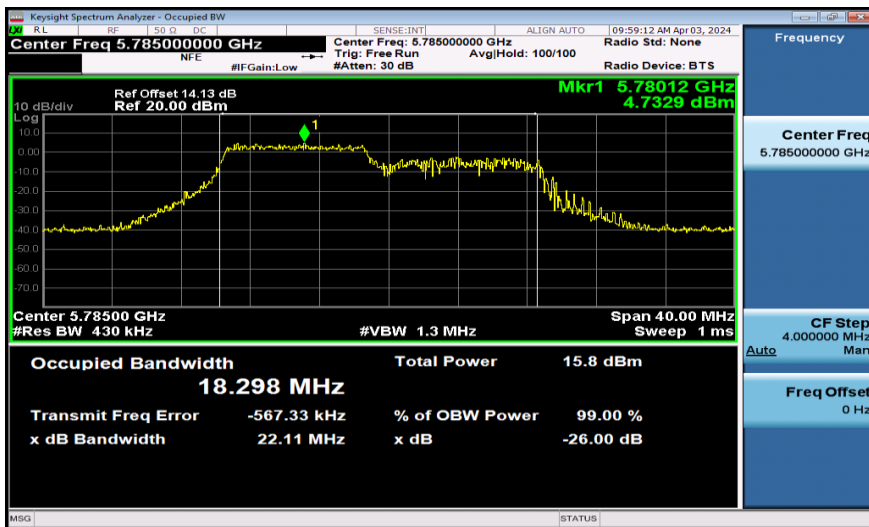
11AX20SISO-Ant1-5785-106Tone
