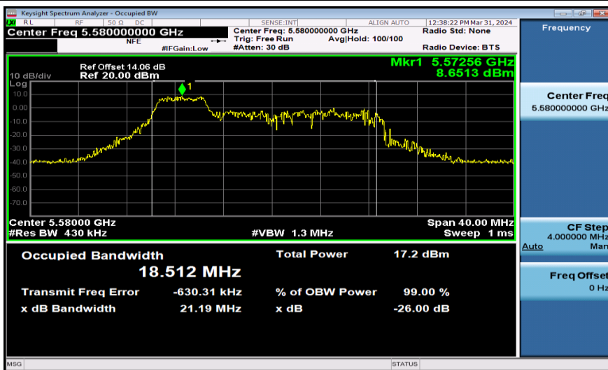
11AX20SISO-Ant1-5580-52Tone
