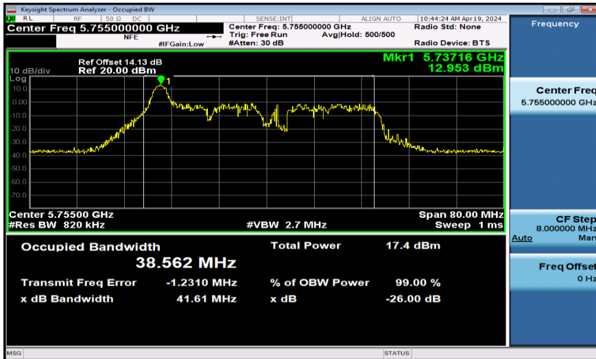
11AX40SISO-Ant1-5755-26Tone
