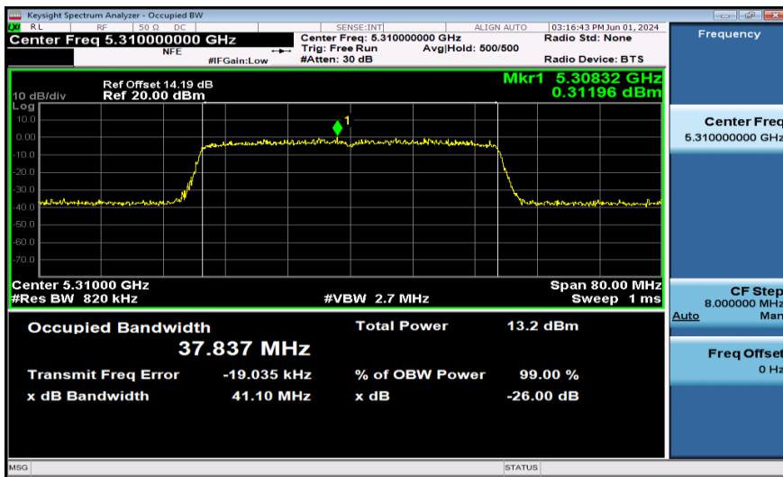
11AX40SISO-Ant1-5310-484Tone-RU61
