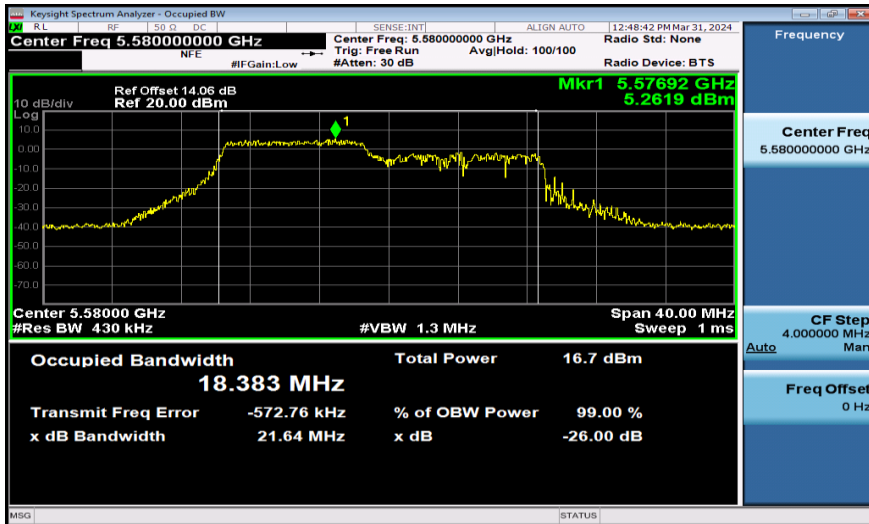
11AX20SISO-Ant1-5580-106Tone
