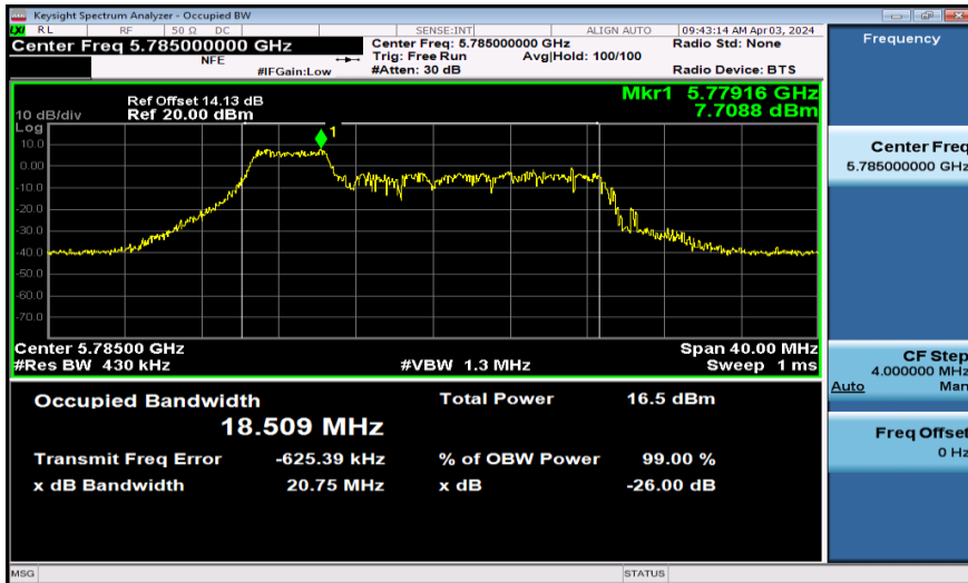
11AX20SISO-Ant1-5785-52Tone
