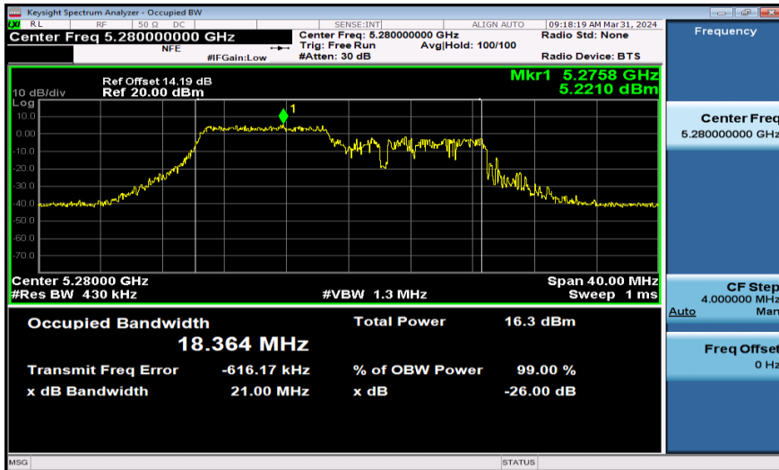
11AX20SISO-Ant1-5280-106Tone
