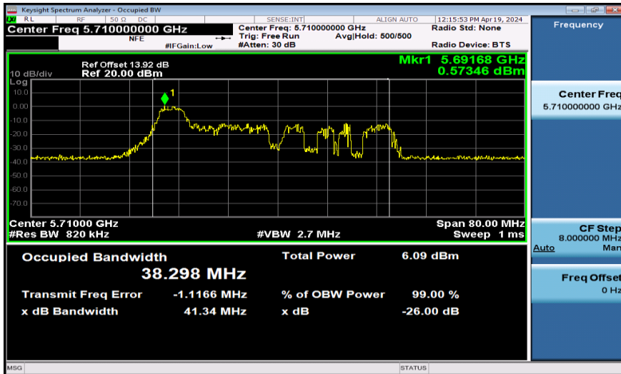
11AX40SISO-Ant1-5710-52Tone
