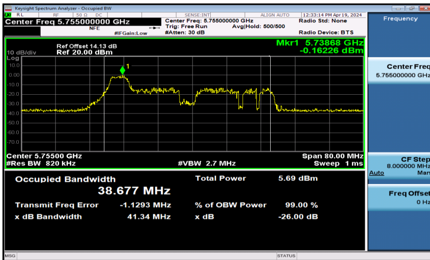
11AX40SISO-Ant1-5755-52Tone
