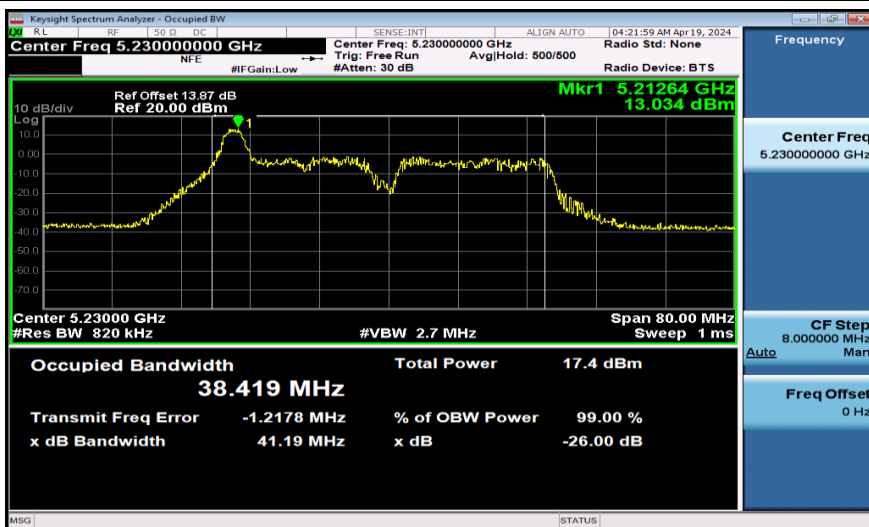
11AX40SISO-Ant1-5230-26Tone-RU0
