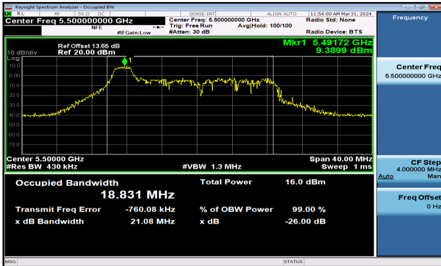
11AX20SISO-Ant1-5500-26Tone
