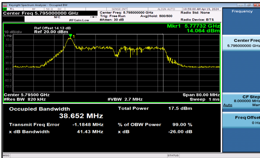
11AX40SISO-Ant1-5795-26Tone
