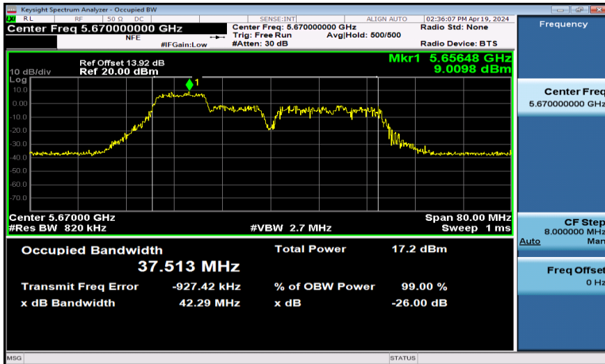
11AX40SISO-Ant1-5670-106Tone
