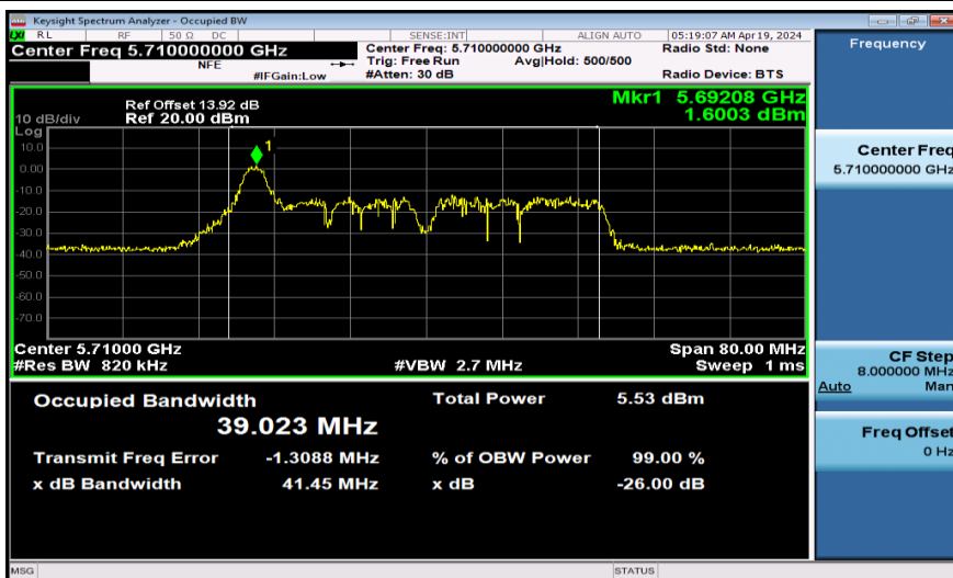
11AX40SISO-Ant1-5710-26Tone
