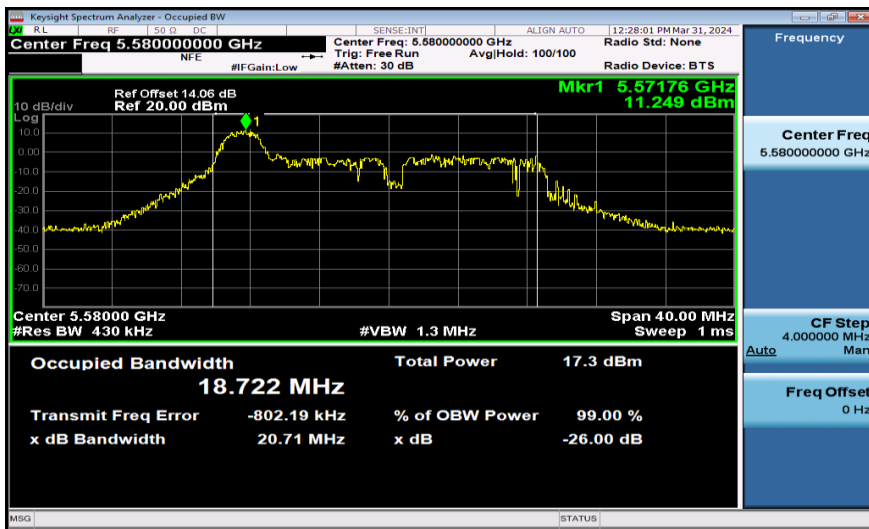
11AX20SISO-Ant1-5580-26Tone
