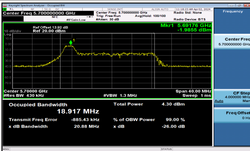
11AX20SISO-Ant1-5700-26Tone
