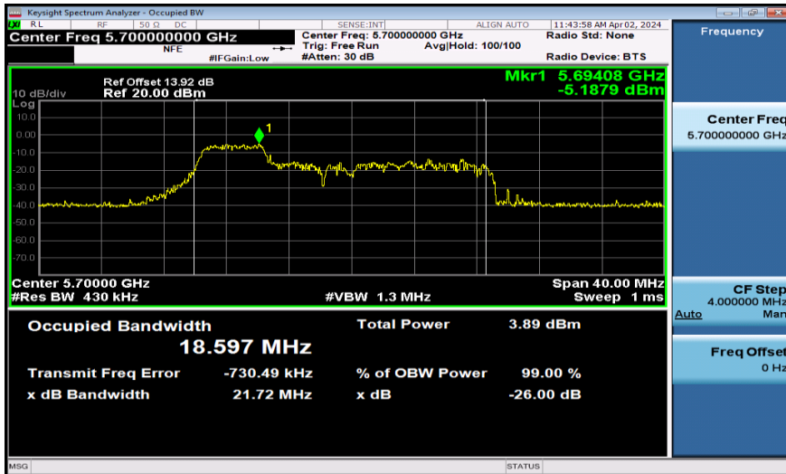
11AX20SISO-Ant1-5700-52Tone
