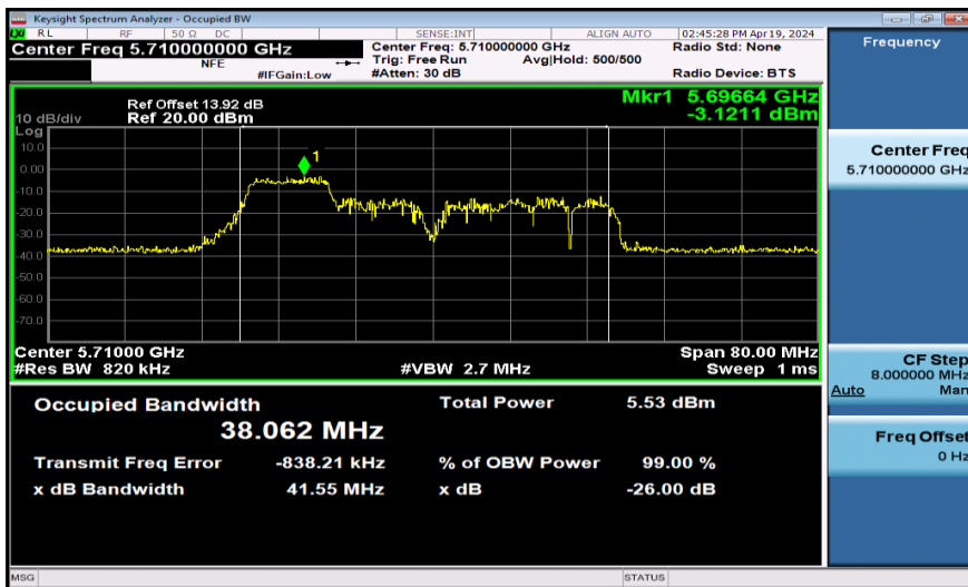
11AX40SISO-Ant1-5710-106Tone
