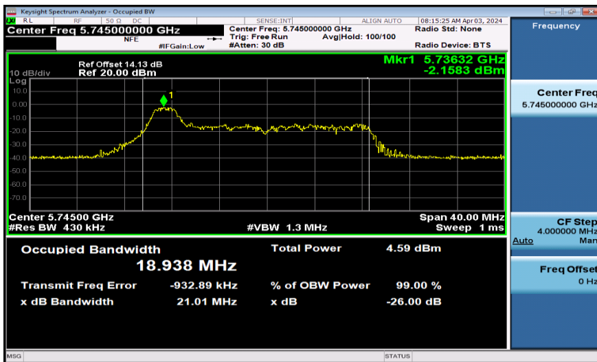
11AX20SISO-Ant1-5745-26Tone
