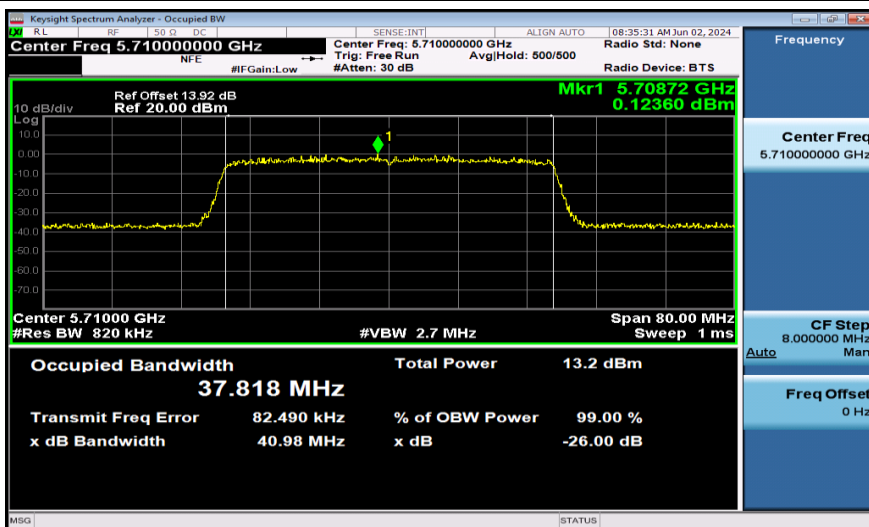
11AX40SISO-Ant1-5710-484Tone
