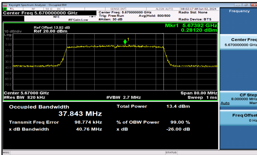
11AX40SISO-Ant1-5670-484Tone
