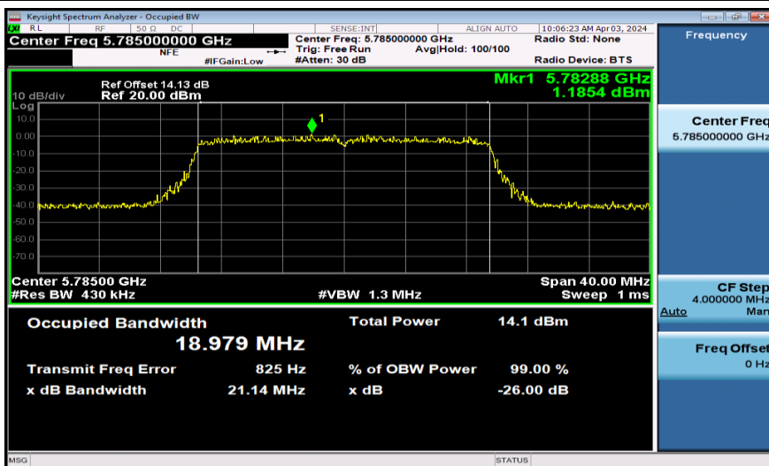
11AX20SISO-Ant1-5785-242Tone
