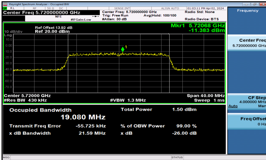
11AX20SISO-Ant1-5720-242Tone
