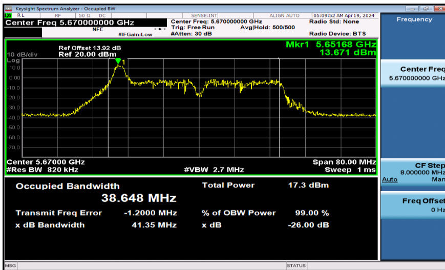
11AX40SISO-Ant1-5670-26Tone
