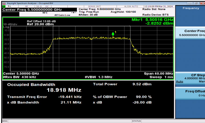
11AX20SISO-Ant1-5500-242Tone
