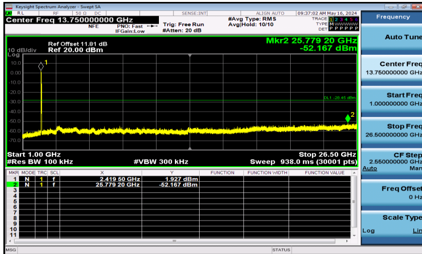
11AX40SISO-Ant1-2437-52Tone-1000~26500-PASS
