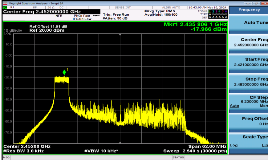
11AX40SISO-Ant1-2452-52Tone-PASS
