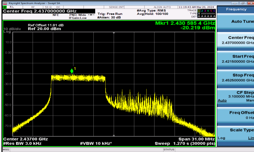
11AX20SISO-Ant1-2437-106Tone-PASS
