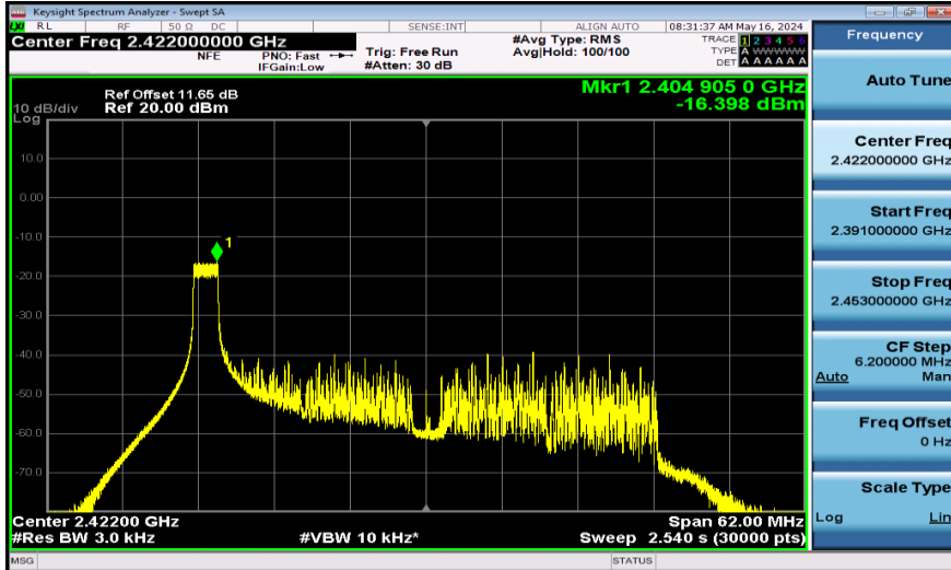
11AX40SISO-Ant1-2422-26Tone-PASS
